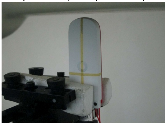
USB Cable Plug-in for USB Configuration 5 (Tip Mode, Test Separation 5 mm)
