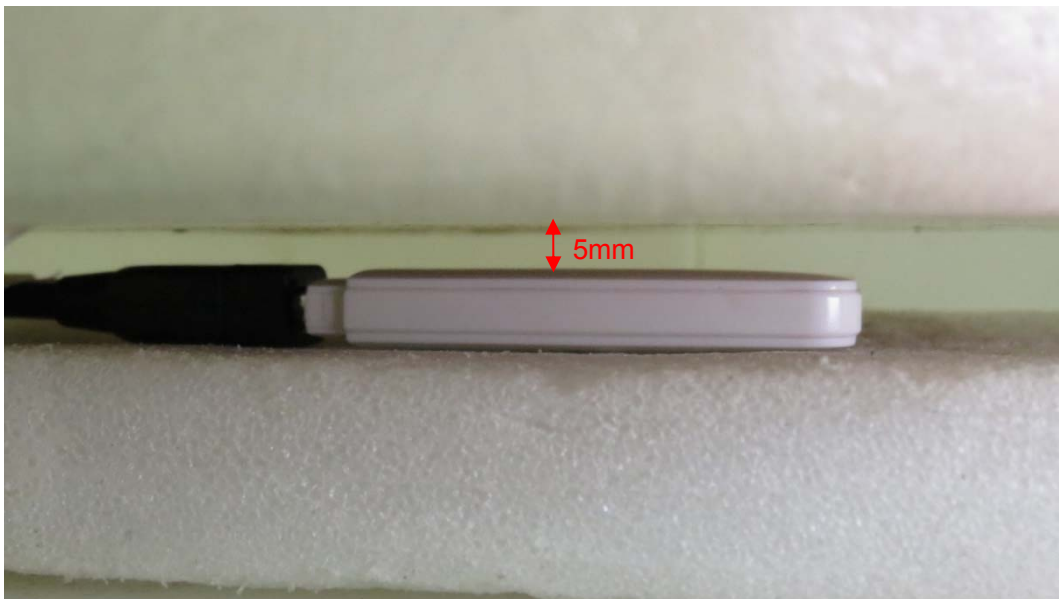
Picture 8: Front Side, the distance from EUT to the bottom of the Phantom is 5mm
