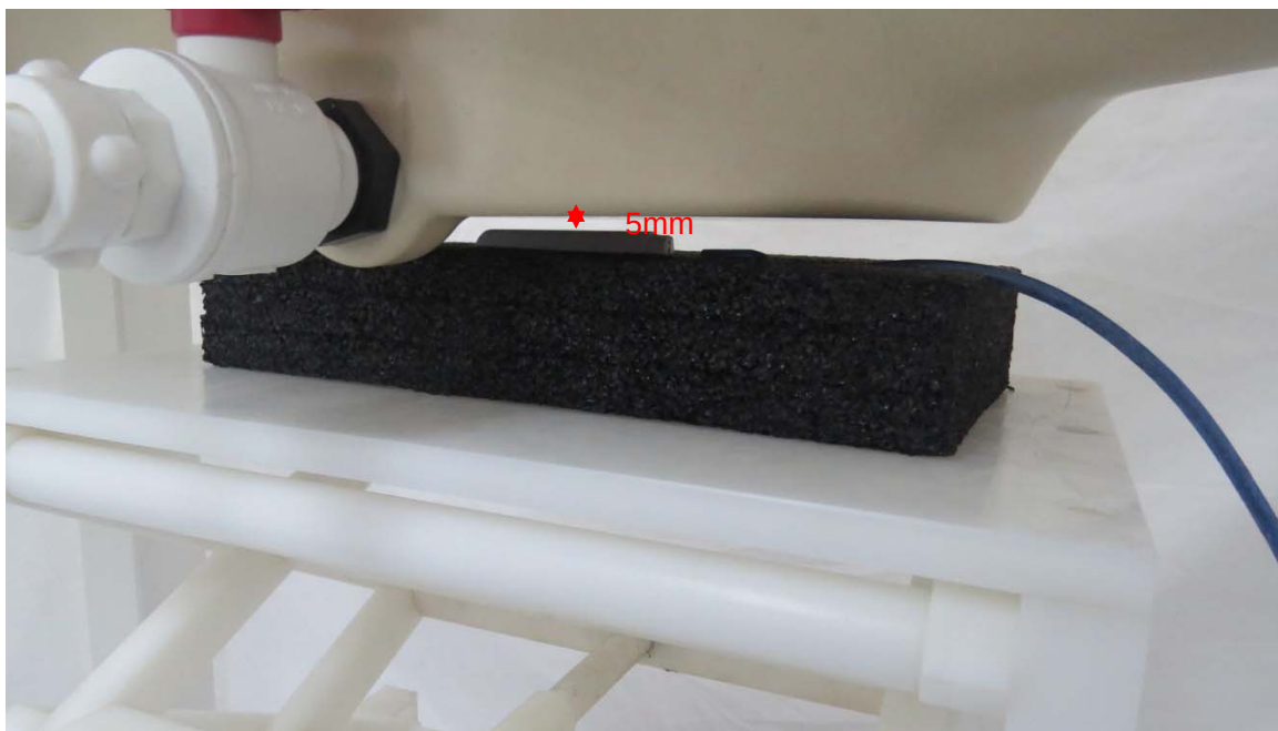
Picture 4: Right Edge, the distance from handset to the bottom of the Phantom is 5mm
