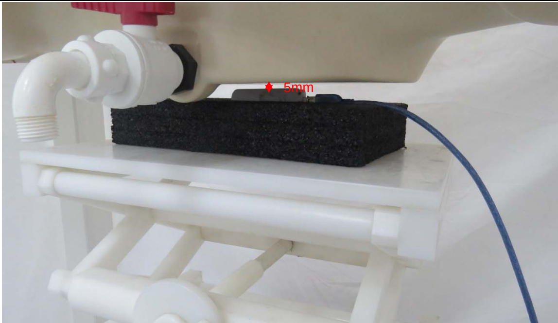
Picture 3: Left Edge, the distance from handset to the bottom of the Phantom is 5mm
