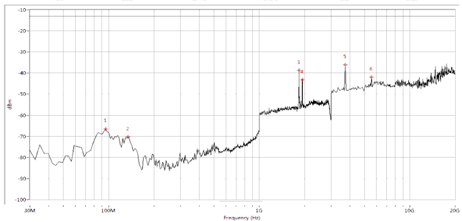
(Plot I.6: HSUPA 850MHz Channel = 4233, Test Antenna Vertical)
