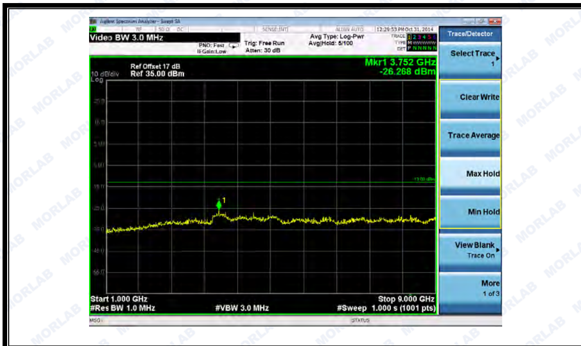
(Plot II.1: HSUPA 850MHz Channel = 4132, 1GHz to 9GHz)
