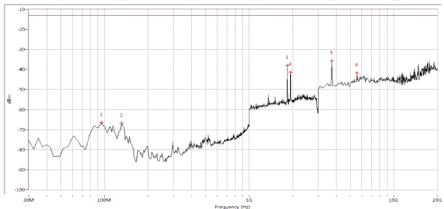
(Plot K.6: HSPA+ 850MHz Channel = 4233, Test Antenna Vertical)
