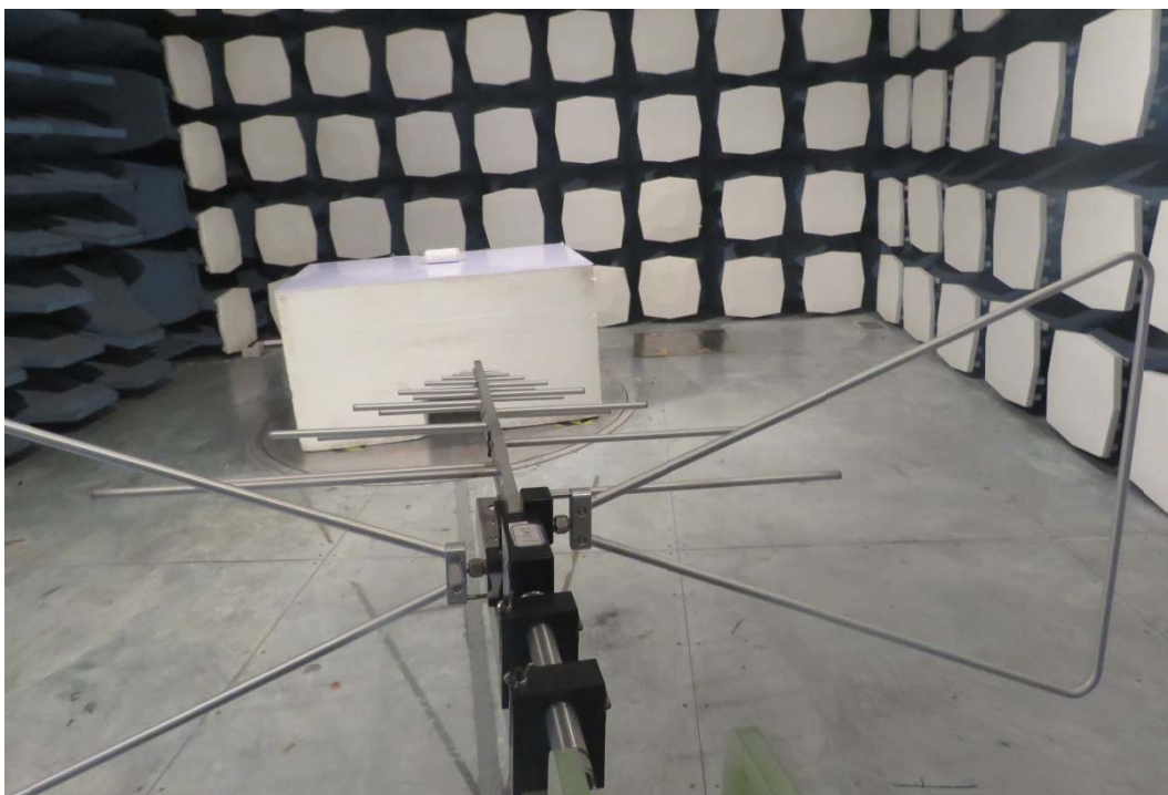
30MHz-1GHz
