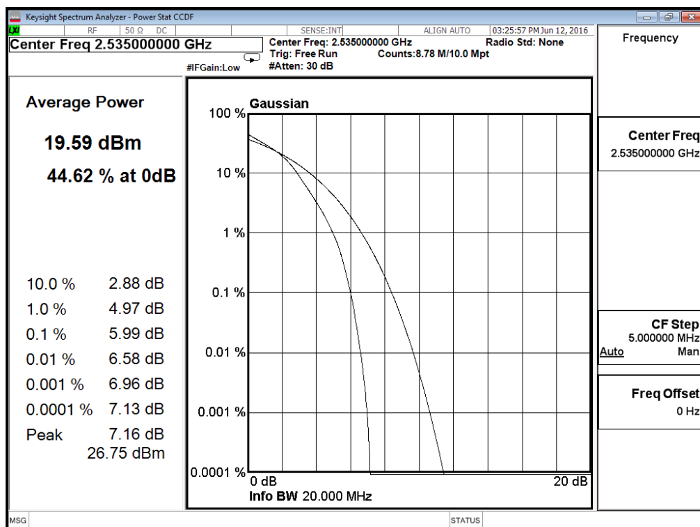
(Plot B4: Band 7/20MHz/16QAM in M Ch 100RB Size)
