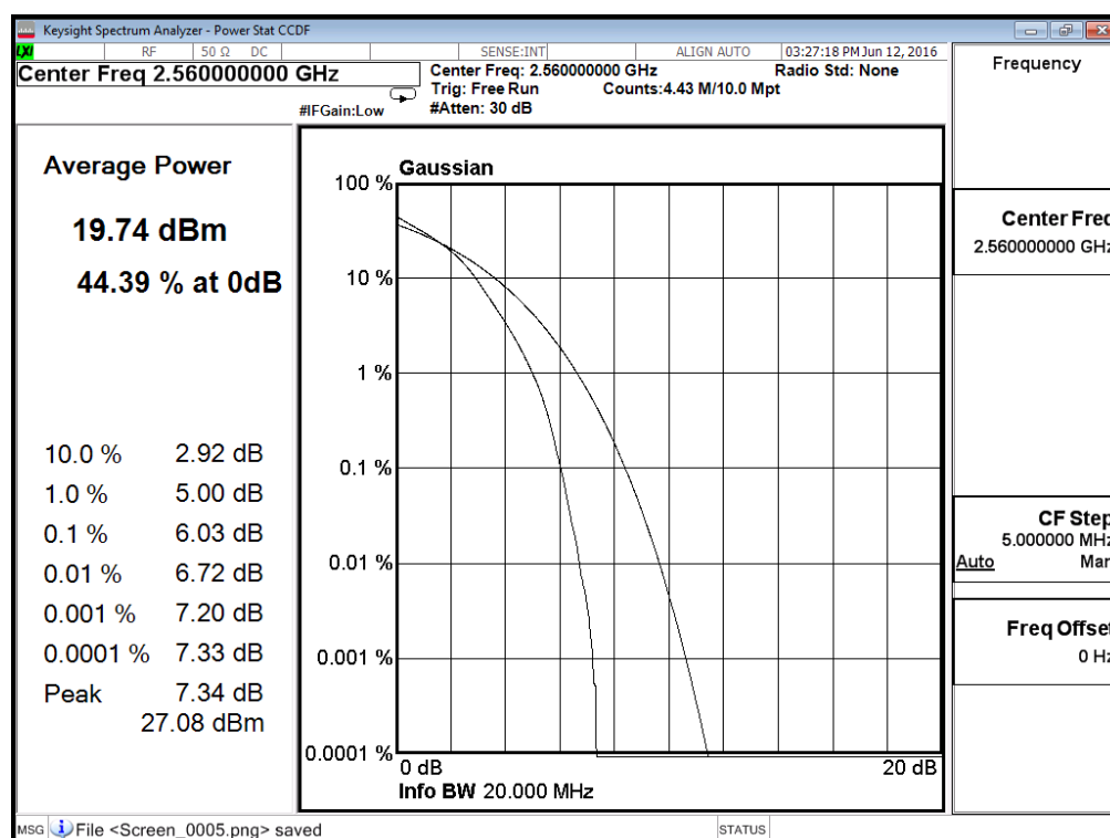
(Plot B6: Band 7/20MHz/16QAM in H Ch 100RB Size)
