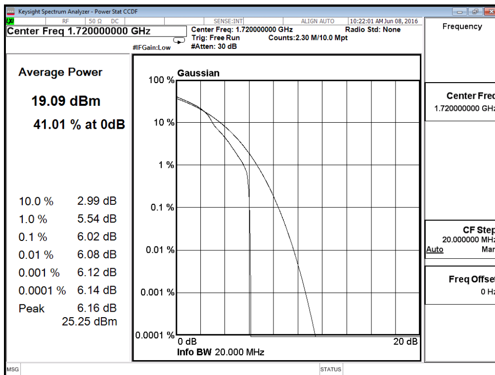
(Plot A1: Band 4/20MHz/16QAM in L Ch 1RB Size)
