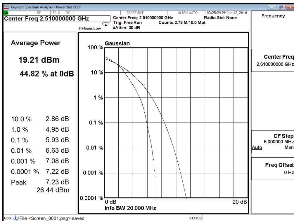
(Plot B2: Band 7/20MHz/16QAM in L Ch 100RB Size)
