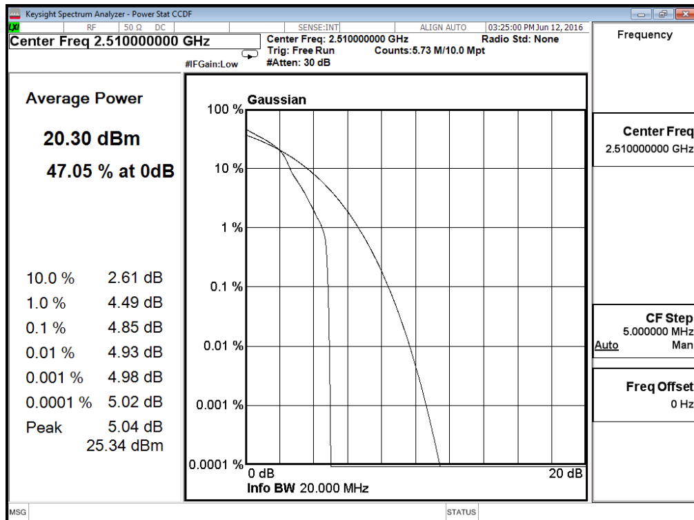
(Plot B1: Band 7/20MHz/16QAM in L Ch 1RB Size )
