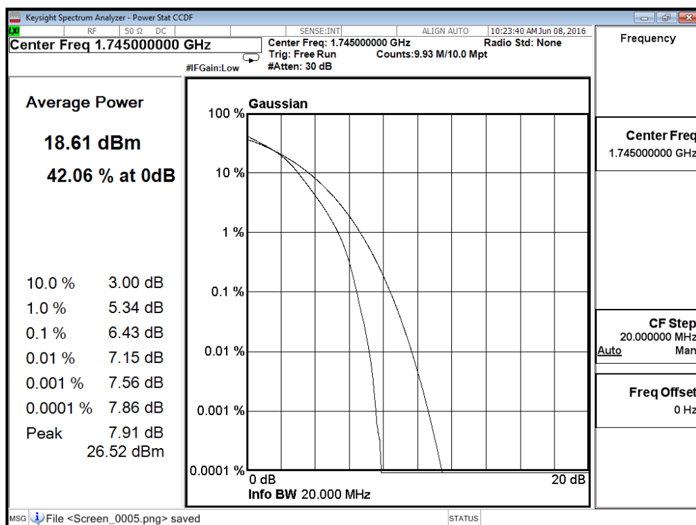
(Plot A6: Band 4/20MHz/16QAM in H Ch 100RB Size)
