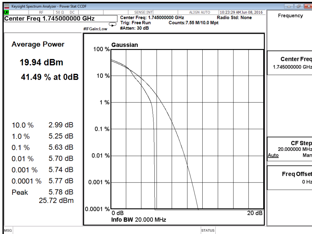
(Plot A5: Band 4/20MHz/16QAM in H Ch 1RB Size)
