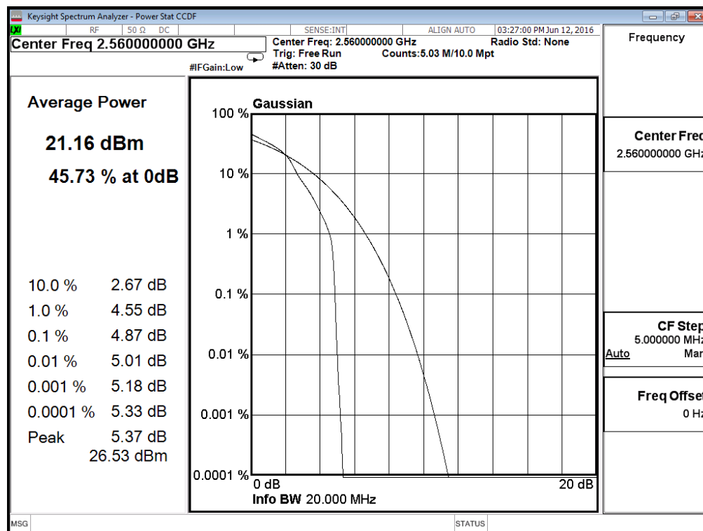
(Plot B5: Band 7/20MHz/16QAM in H Ch 1RB Size)
