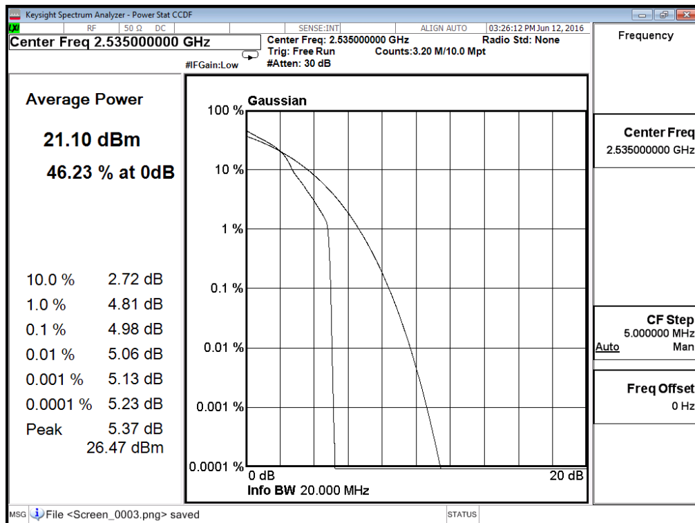
(Plot B3: Band 7/20MHz/16QAM in M Ch 1RB Size)
