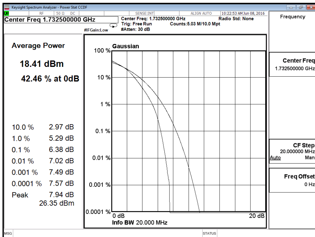
(Plot A4: Band 4/20MHz/16QAM in M Ch 100RB Size)
