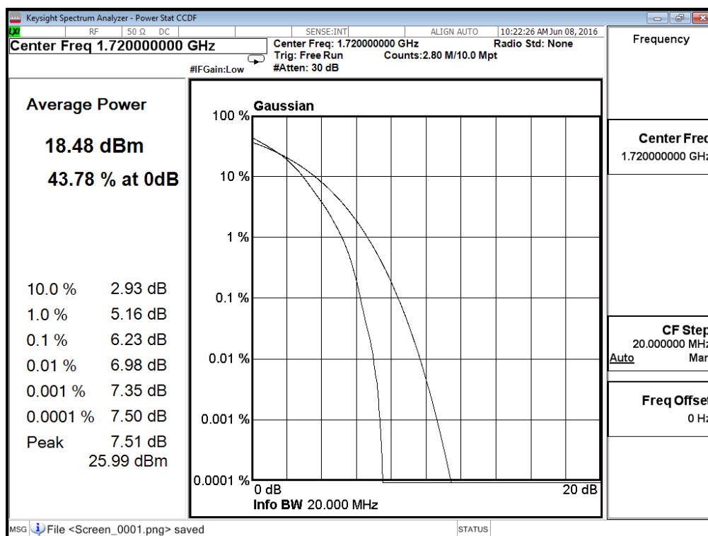
(Plot A2: Band 4/20MHz/16QAM in L Ch 100RB Size)
