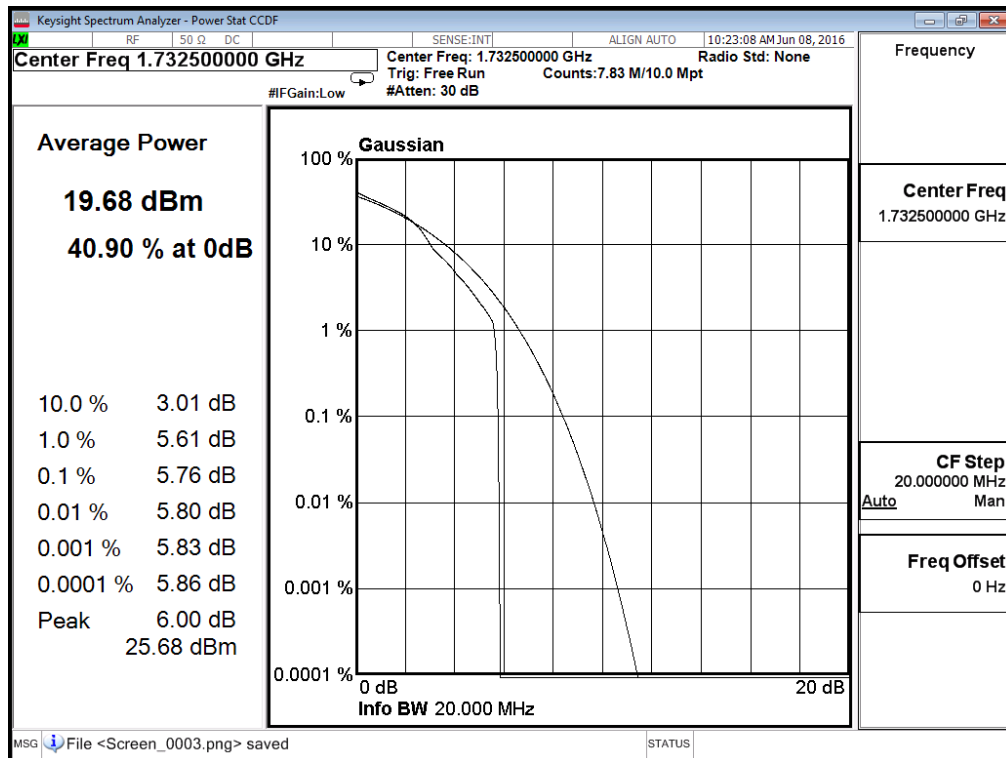
(Plot A3: Band 4/20MHz/16QAM in M Ch 1RB Size)
