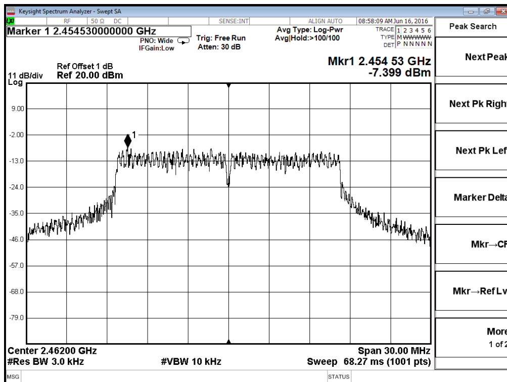
Antenna 1 - 802.11g - Channel 11
