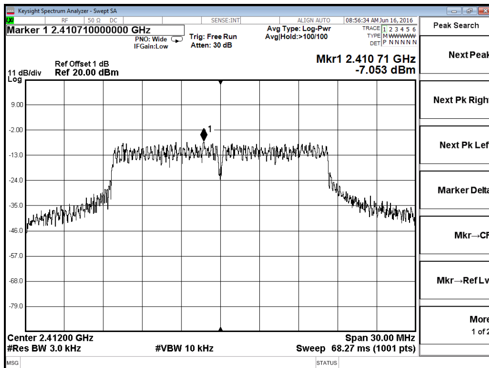
Antenna 1 - 802.11g - Channel 1
