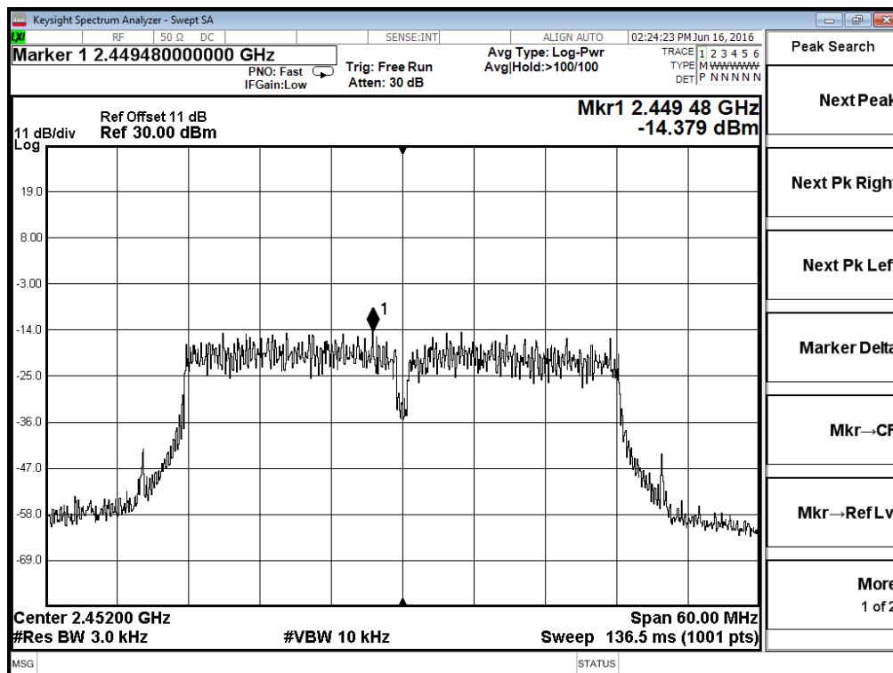
Antenna 2 - 802.11n40 - Channel 9
