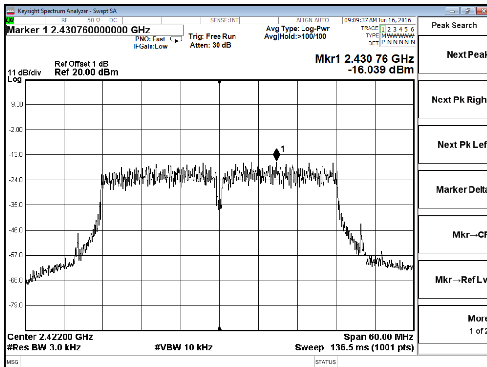
Antenna 1 - 802.11n40 - Channel 3
