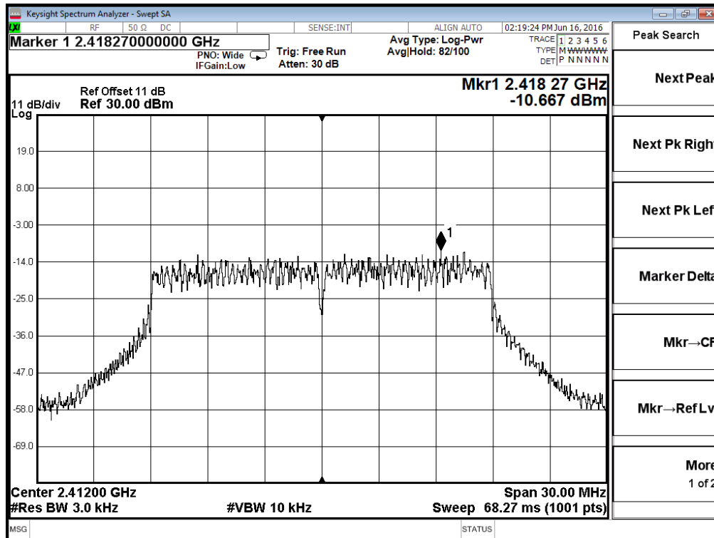
Antenna 2 - 802.11n20 - Channel 1
