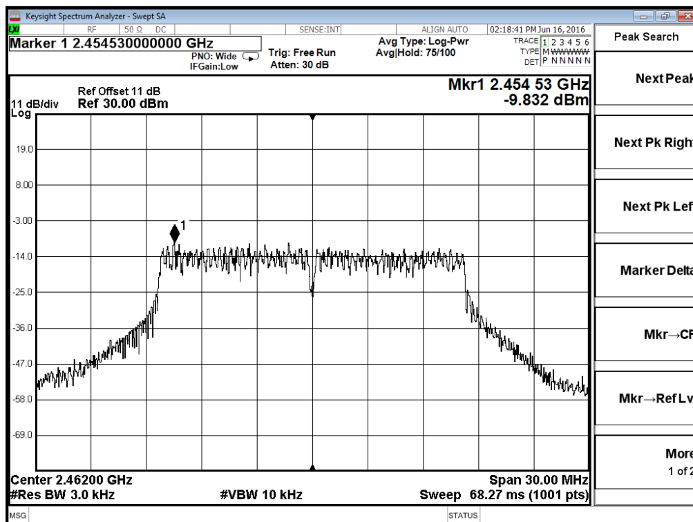
Antenna 2 - 802.11g - Channel 11
