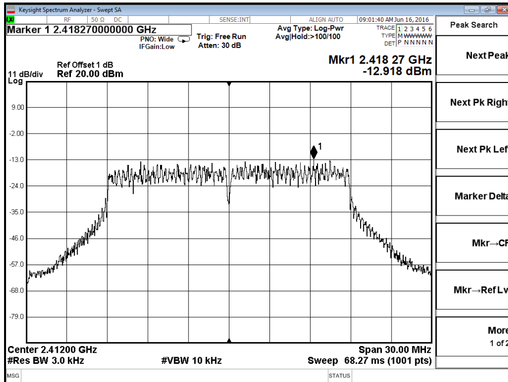
Antenna 1 - 802.11n20 - Channel 1
