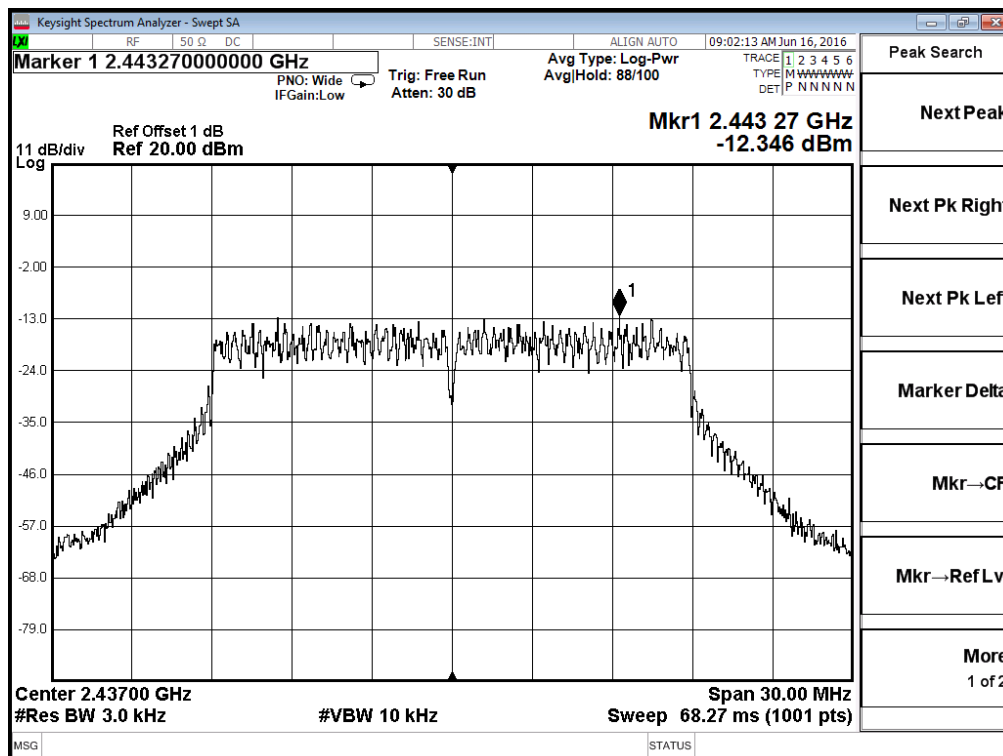
Antenna 1 - 802.11n20 - Channel 6
