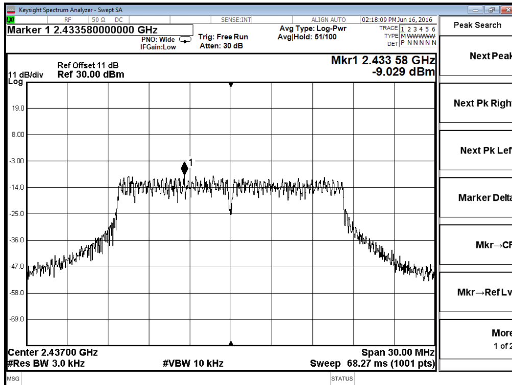
Antenna 2 - 802.11g - Channel 6
