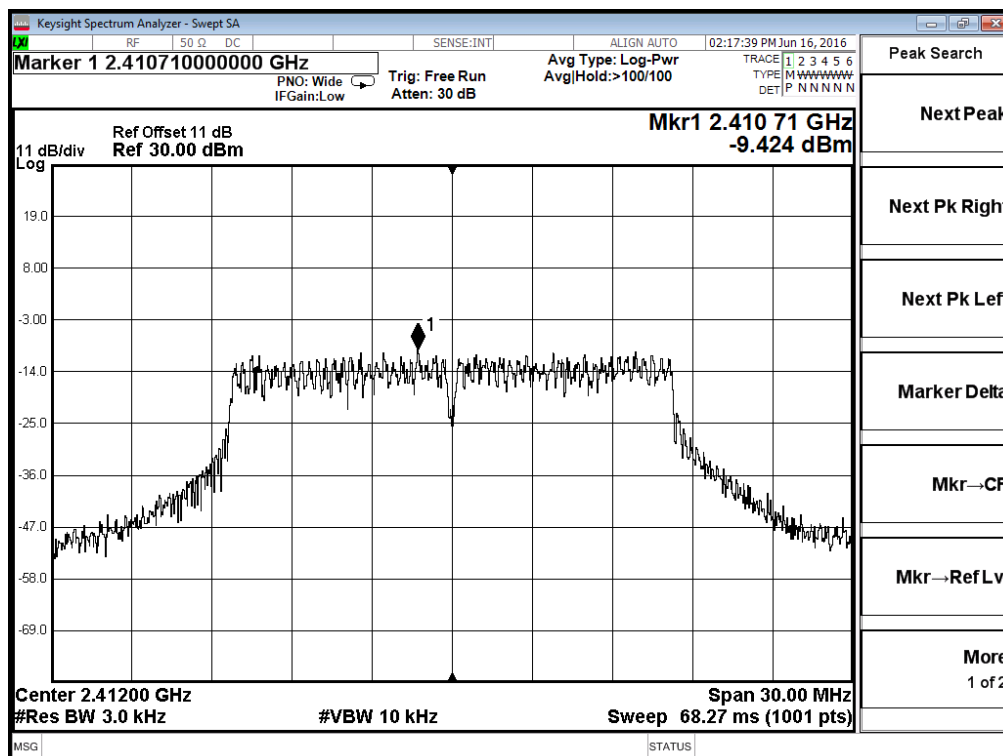
Antenna 2 - 802.11g - Channel 1
