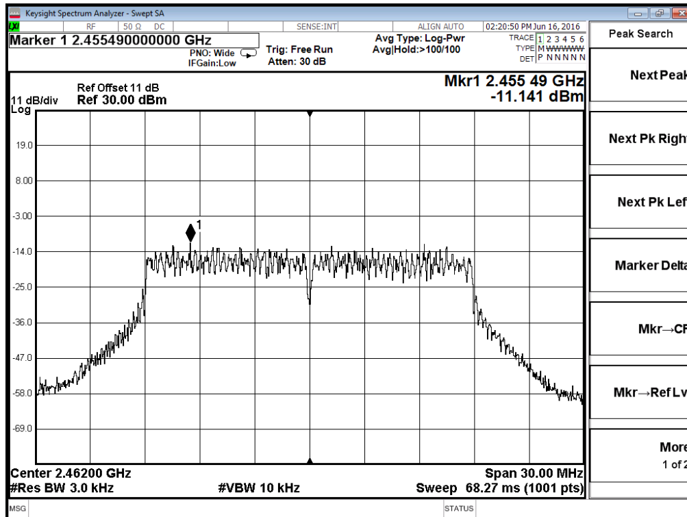
Antenna 2 - 802.11n20 - Channel 11
