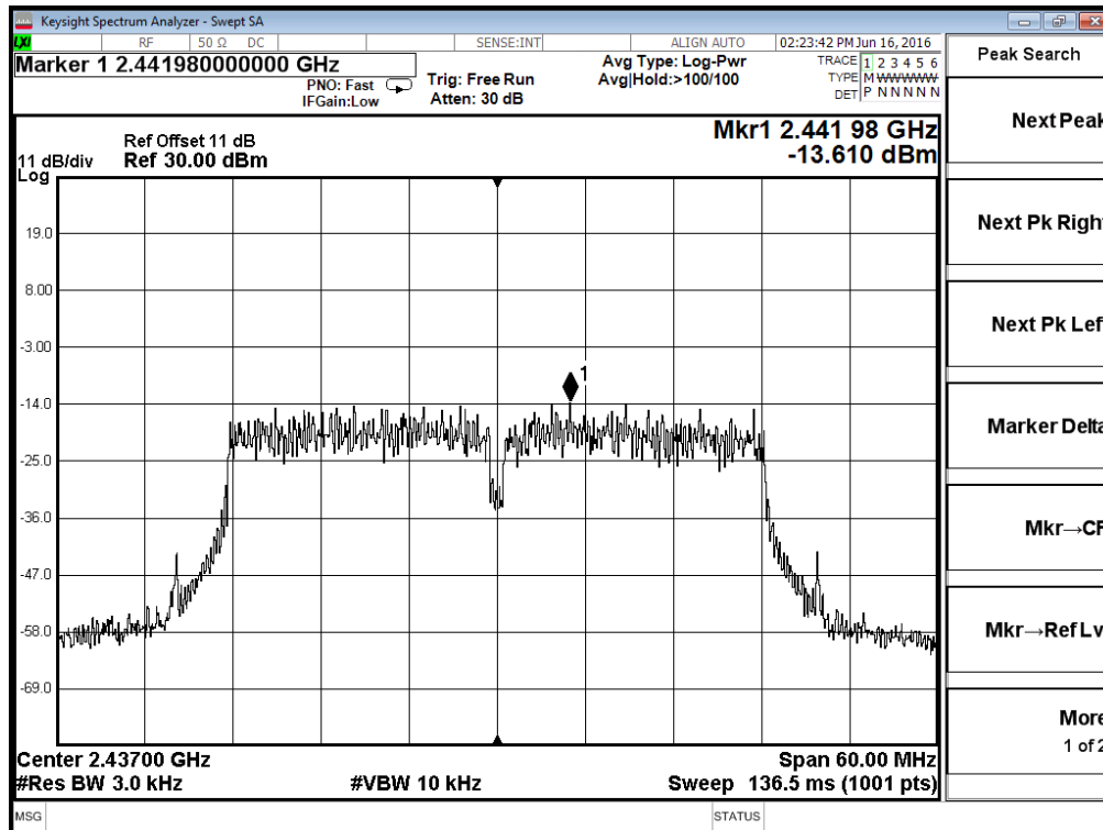
Antenna 2 - 802.11n40 - Channel 6
