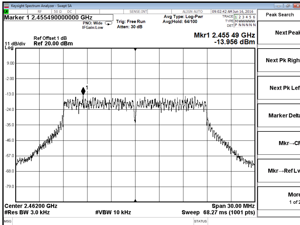
Antenna 1 - 802.11n20 - Channel 11
