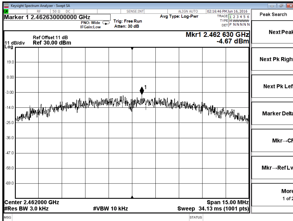
Antenna 2 - 802.11b - Channel 11
