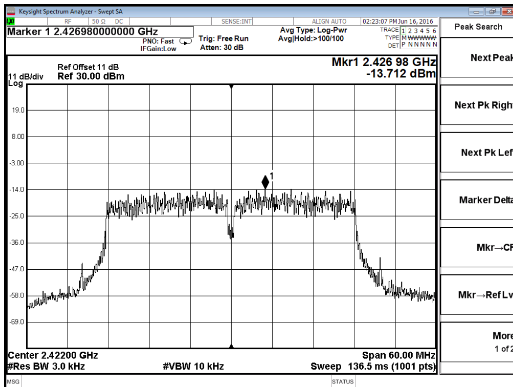
Antenna 2 - 802.11n40 - Channel 3
