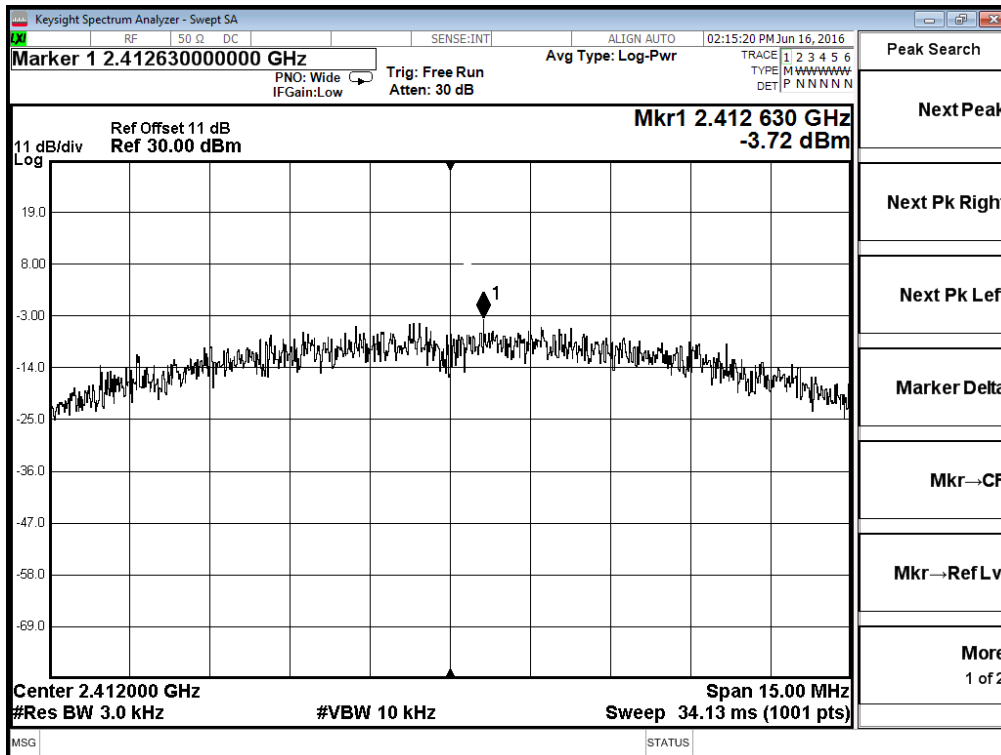
Antenna 2 - 802.11b - Channel 1
