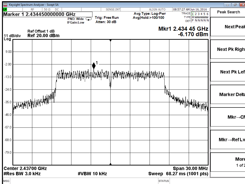
Antenna 1 - 802.11g - Channel 6
