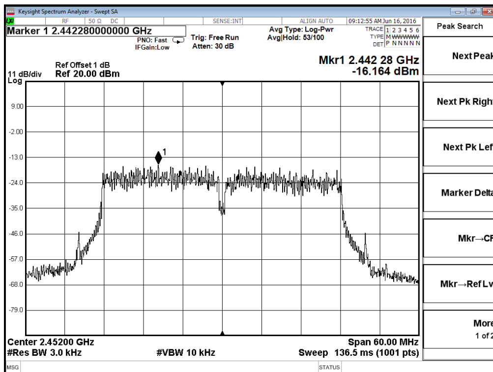
Antenna 1 - 802.11n40 - Channel 9
