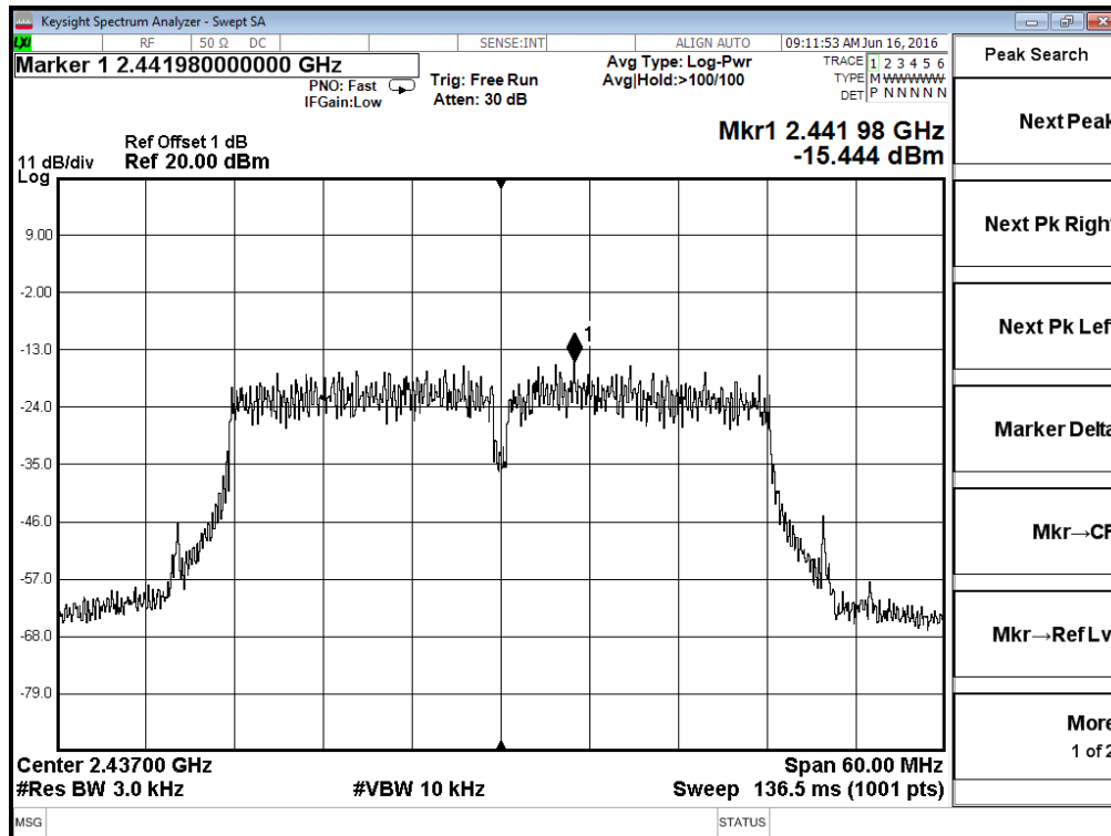
Antenna 1 - 802.11n40 - Channel 6
