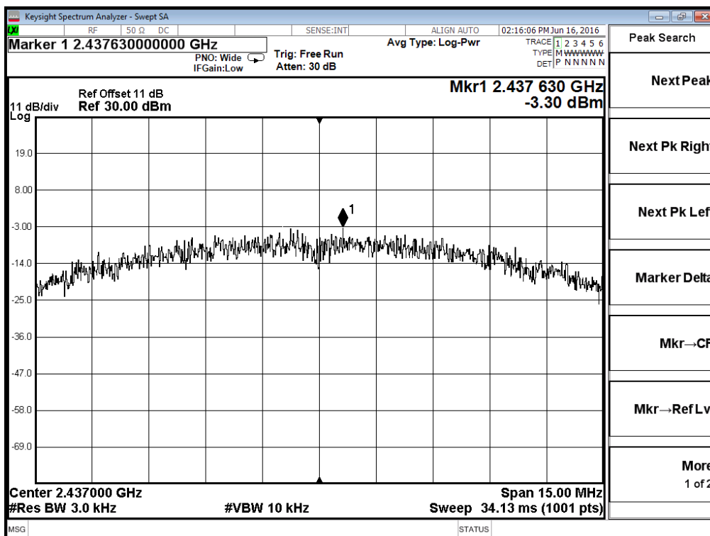
Antenna 2 - 802.11b - Channel 6
