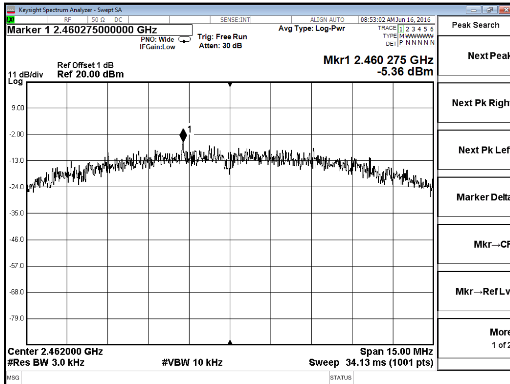
Antenna 1 - 802.11b - Channel 11
