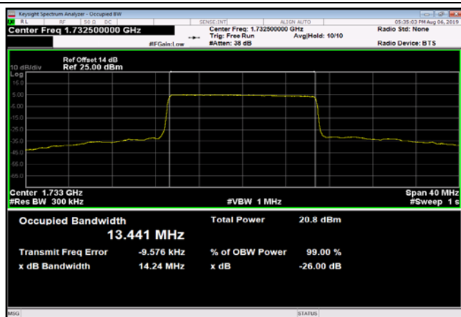
FDD04_MidRange_20_1732.5_Q16
