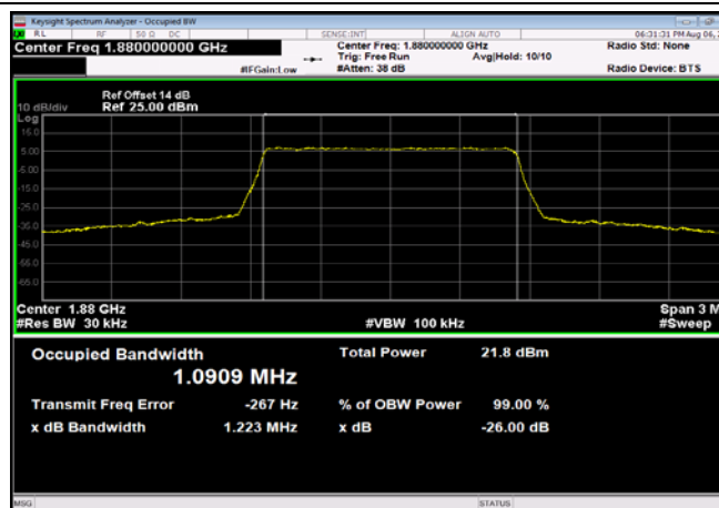
FDD02_MidRange_3_1880_QPSK
