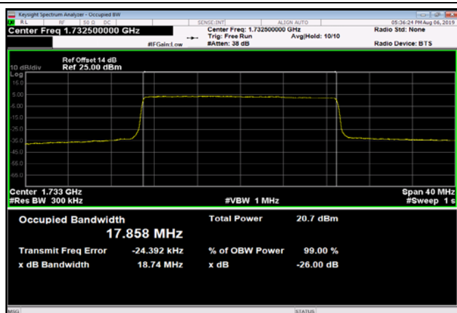
FDD04_MidRange_20_1732.5_Q16
