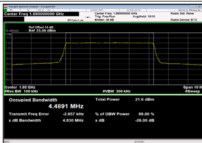
FDD02_MidRange_5_1880_QPSK
