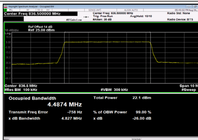
FDD05_MidRange_5_836.5_QPSK
