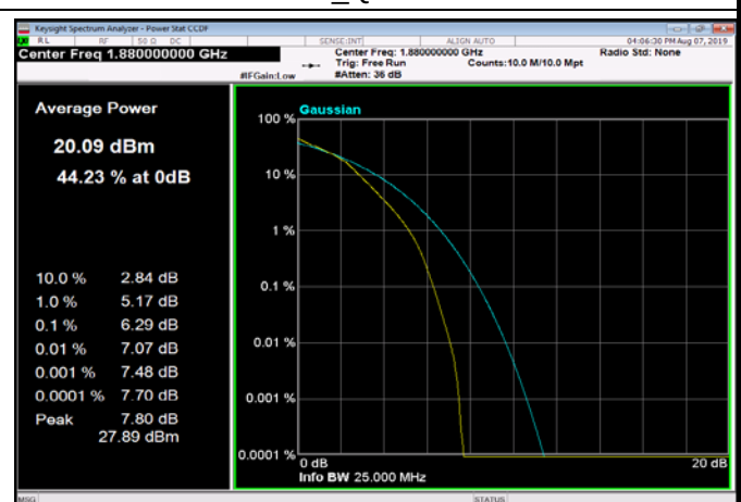
FDD02_MidRange_20MHz_1880_fullRB_Q16
