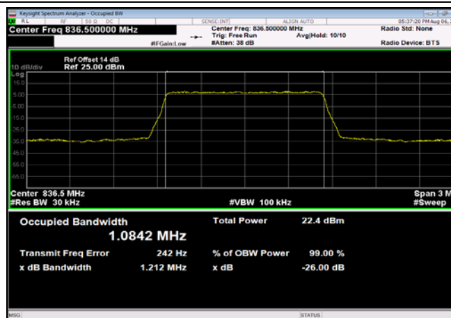
FDD05_MidRange_3_836.5_QPSK
