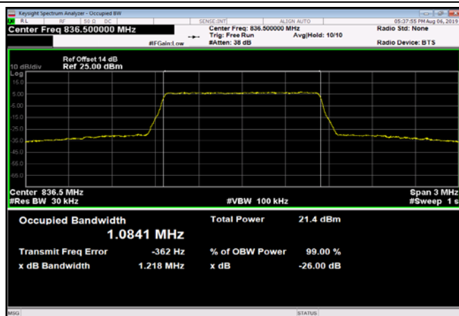
FDD05_MidRange_3_836.5_Q16
