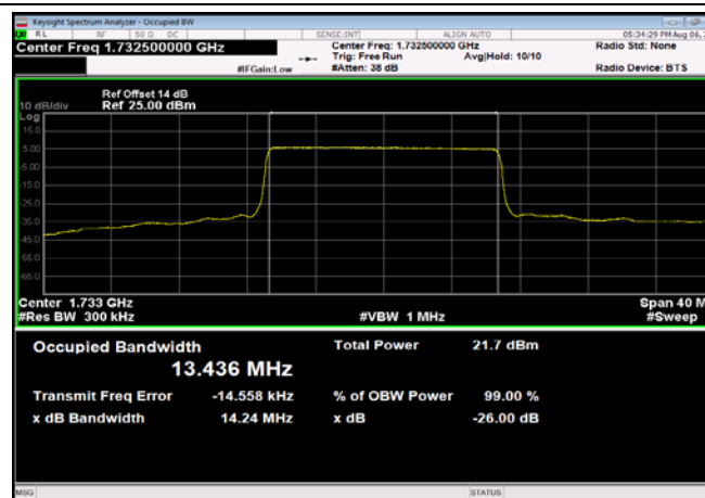
FDD04_MidRange_20_1732.5_QPSK
