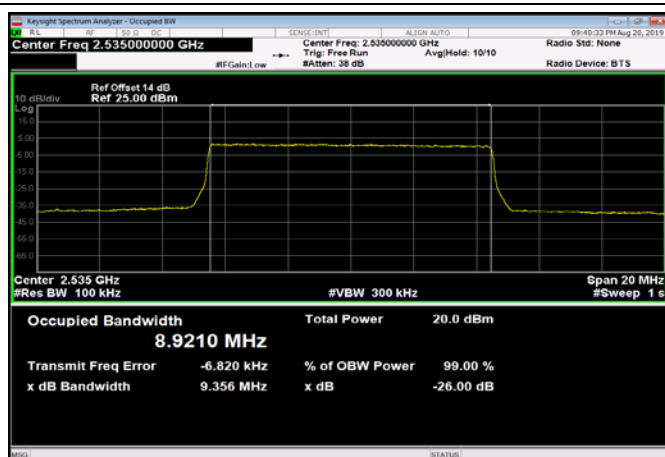
FDD07_MidRange_10_2535_Q16
