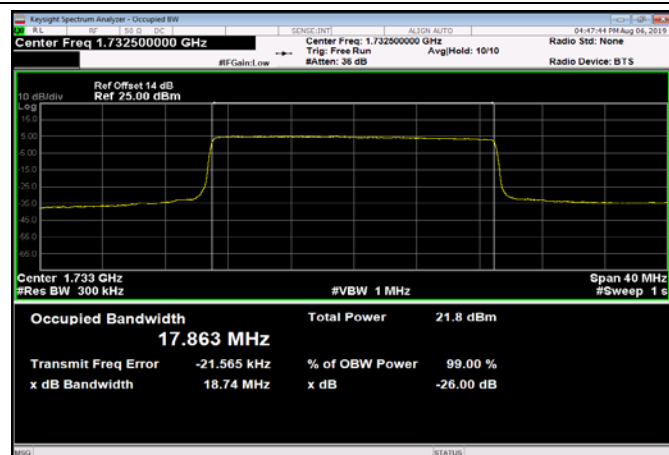
FDD04_MidRange_20MHz_1732.5MHz _QPSK
