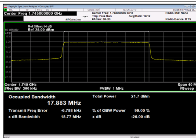
FDD66_MidRange_20_1745_QPSK
