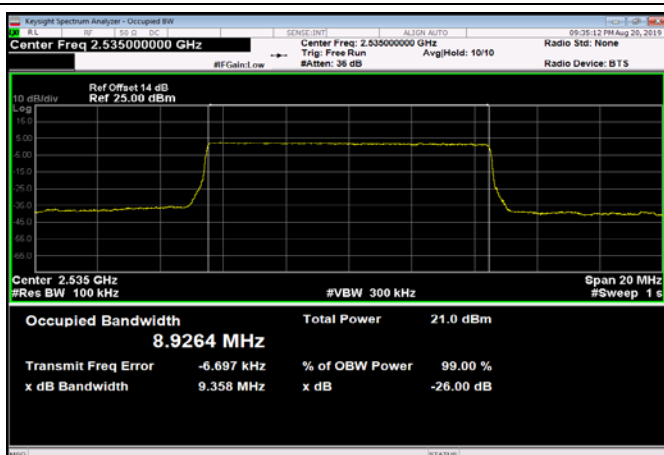
FDD07_MidRange_10MHz_2535MHz_QPSK
