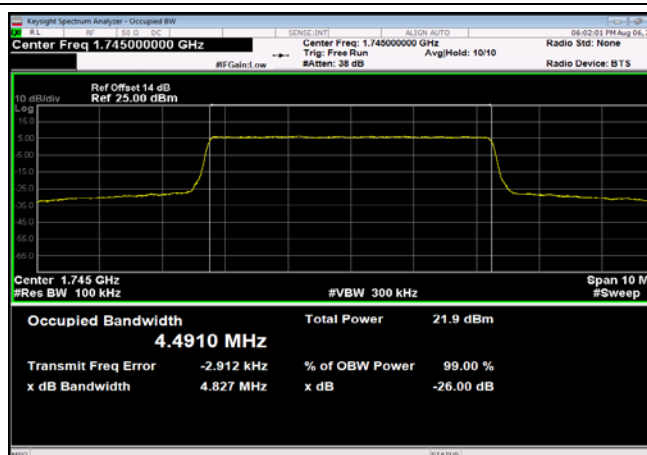
FDD66_MidRange_5_1745_QPSK
