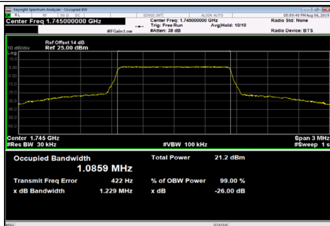
FDD66_MidRange_3_1745_Q16
