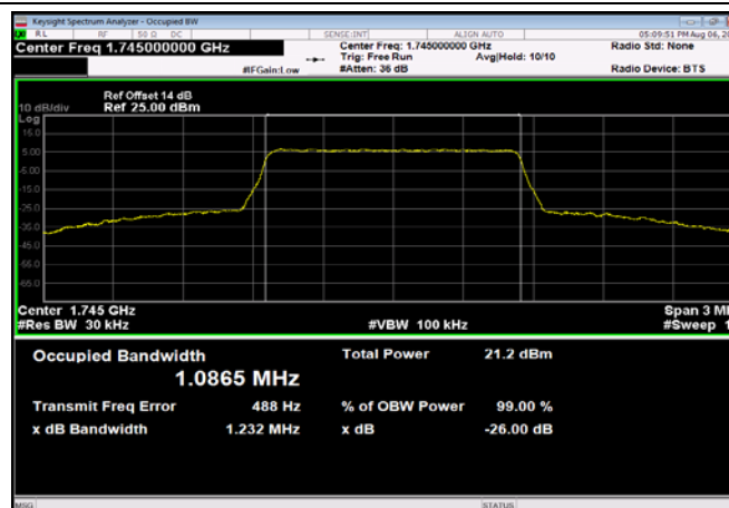
FDD66_MidRange_3MHz_1745MHz_Q16
