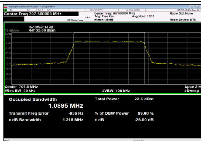
FDD12_MidRange_1.4_707.5_QPSK
