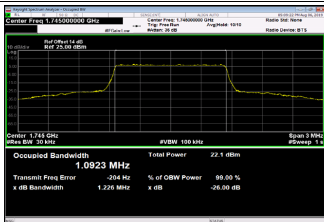
FDD66_MidRange_3MHz_1745MHz_QPSK
