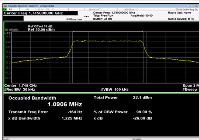
FDD66_MidRange_3_1745_QPSK
