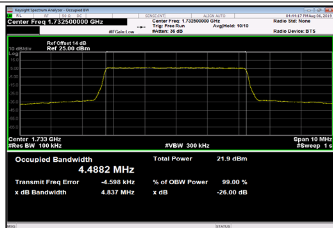
FDD04_MidRange_5MHz_1732.5MHz_QPSK
