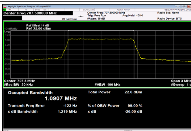
FDD12_MidRange_1.4MHz_707.5MHz_QPSK
