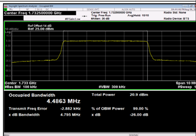
FDD04_MidRange_5MHz_1732.5MHz_Q16
