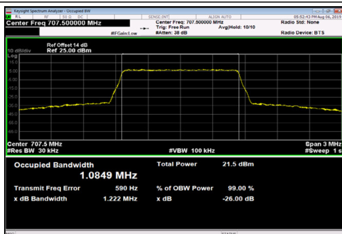
FDD12_MidRange_1.4_707.5_Q16
