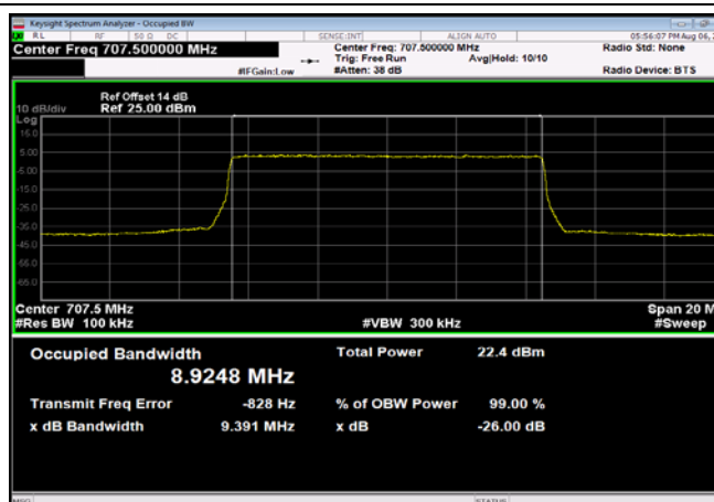
FDD12_MidRange_10_707.5_QPSK
