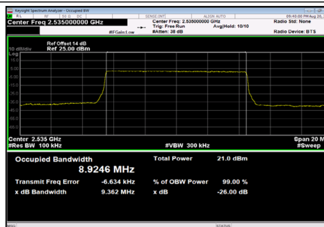
FDD07_MidRange_10_2535_QPSK
