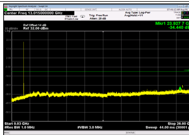
FDD66_LowRange_10MHz_30MHz~26GHz
