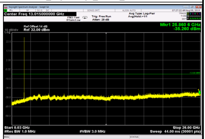
FDD04_LowRange_15MHz_30MHz~26GHz
