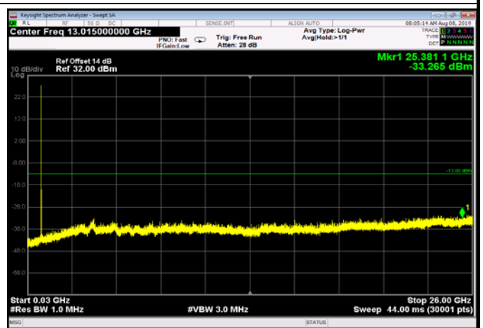
FDD05_HighRange_5MHz_30MHz~26GHz
