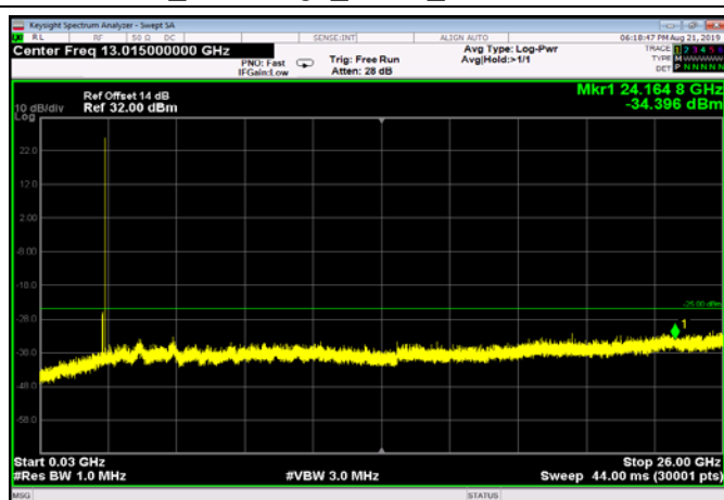
FDD07_LowRange_5MHz_30MHz~26GHz
