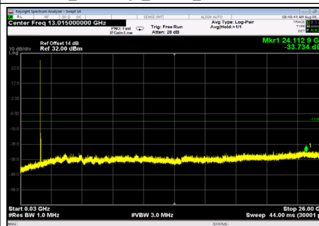
FDD04_MidRange_10MHz_30MHz~26GHz
