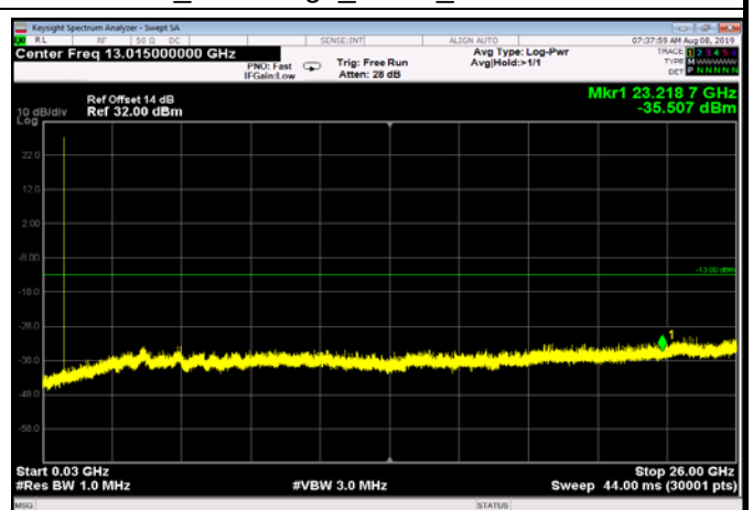
FDD05_LowRange_5MHz_30MHz~26GHz
