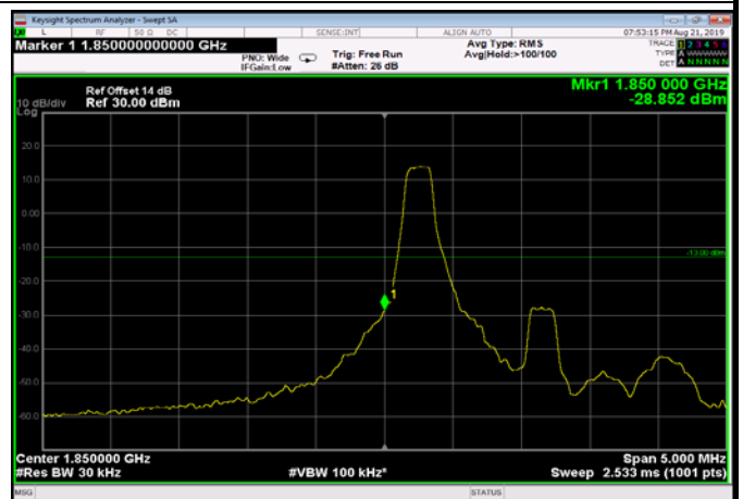
LowRange_FDD02_1.4MHz_1850.7_fullRB _Low_Q16
