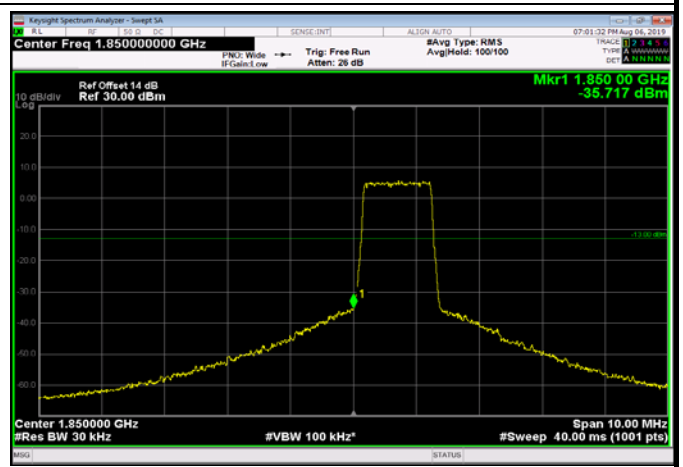
LowRange_FDD02_1.4MHz_1850.7_fullRB _Low_Q16
