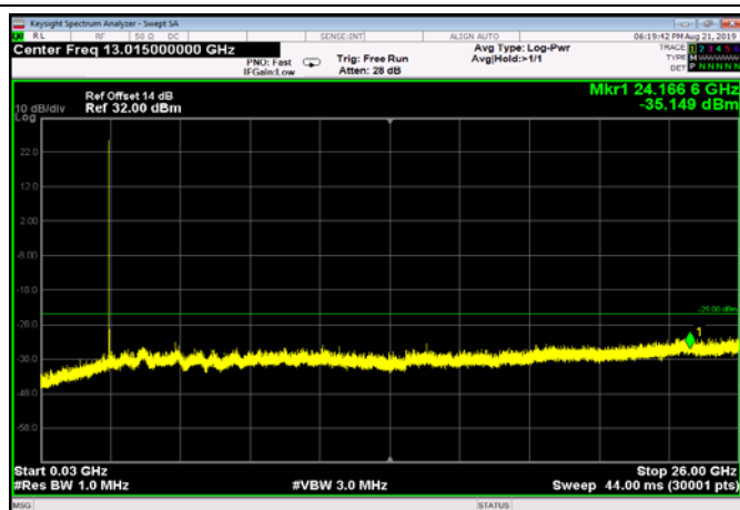
FDD07_LowRange_15MHz_30MHz~26GHz
