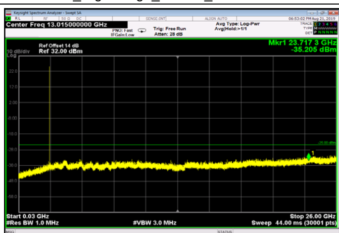
FDD07_HighRange_15MHz_30MHz~26GHz
