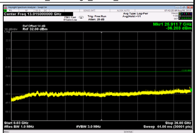
FDD66_LowRange_5MHz_30MHz~26GHz
