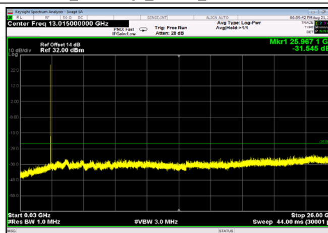
FDD07_LowRange_20MHz_30MHz~26GHz
