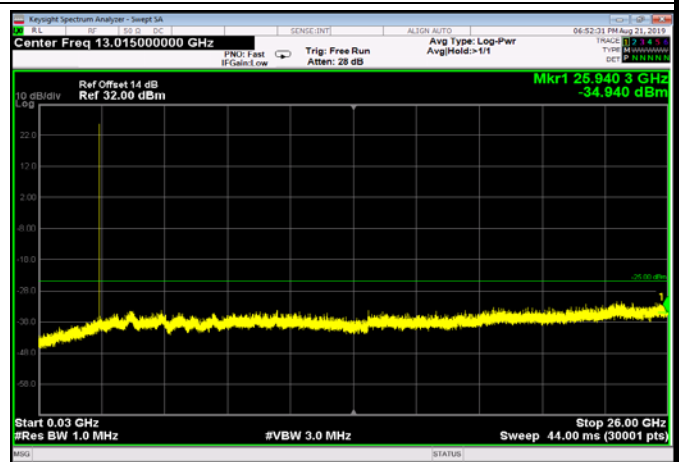
FDD07_MidRange_5MHz_30MHz~26GHz
