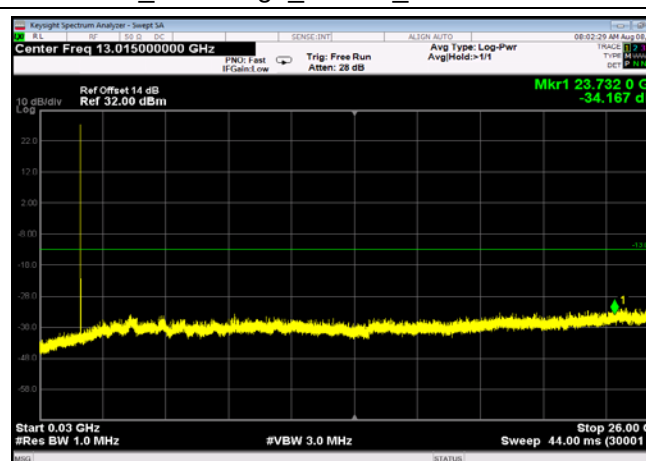
FDD04_LowRange_10MHz_30MHz~26GHz
