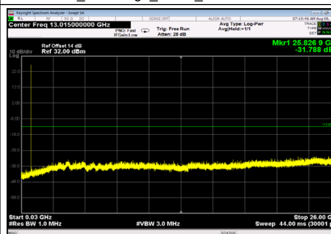
FDD07_HighRange_10MHz_30MHz~26GHz
