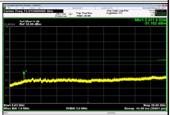
FDD66_LowRange_20MHz_30MHz~26GHz
