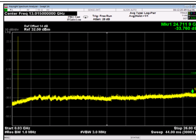
FDD05_HighRange_3MHz_30MHz~26GHz
