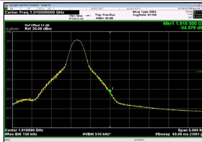
HighRange_FDD02_15MHz_1902.5_fullIRB _High_QPSK
