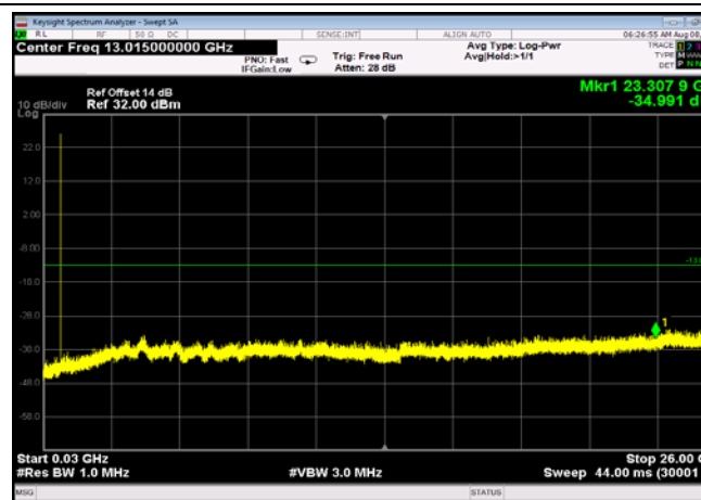
FDD12_LowRange_10MHz_30MHz~26GHz
