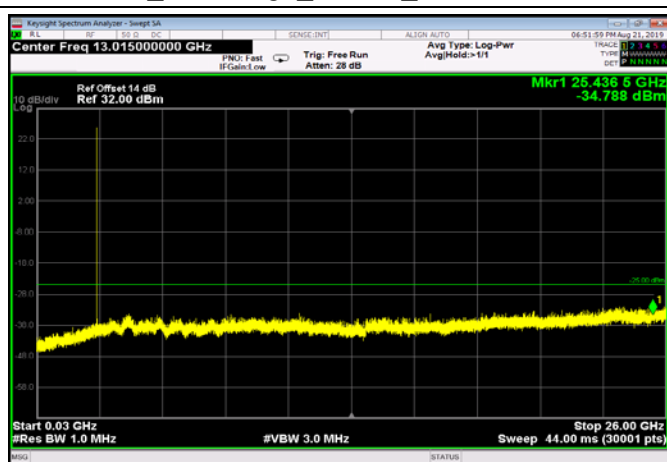
FDD07_LowRange_5MHz_30MHz~26GHz
