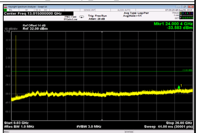
FDD12_LowRange_5MHz_30MHz~26GHz
