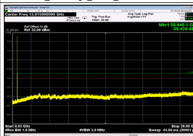
FDD66_HighRange_3MHz_30MHz~26GHz
