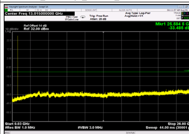
FDD05_MidRange_3MHz_30MHz~26GHz
