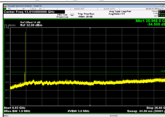
FDD07_LowRange_20MHz_30MHz~26GHz
