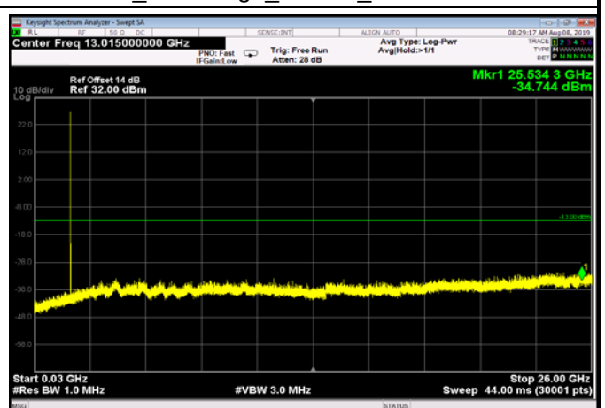
FDD04_LowRange_15MHz_30MHz~26GHz
