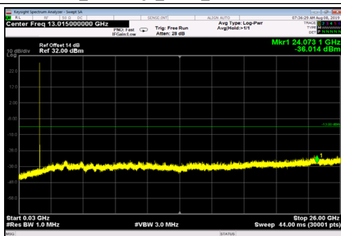
FDD04_MidRange_15MHz_30MHz~26GHz
