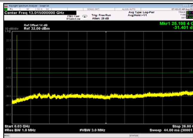
FDD12_LowRange_1.4MHz_30MHz~26GHz
