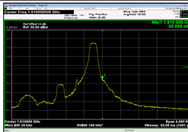
HighRange_FDD02_1.4MHz_1909.3 _fullRB_High_QPSK
