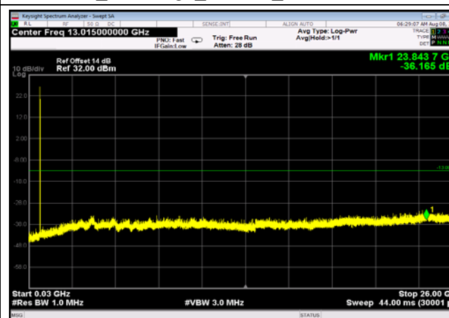
FDD12_MidRange_5MHz_30MHz~26GHz
