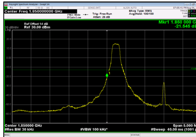
LowRange_FDD02_3MHz_1851.5_fullRB _Low_QPSK
