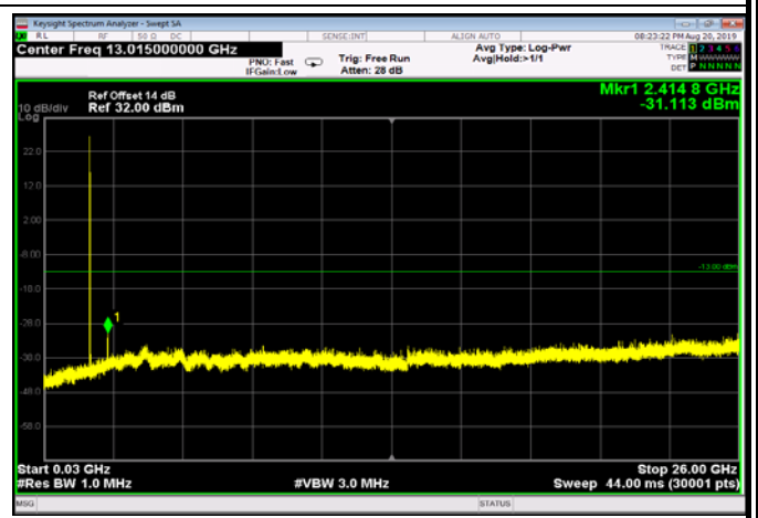
FDD66_MidRange_1.4MHz_30MHz~26GHz
