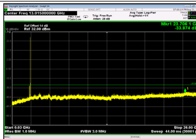
FDD12_HighRange_1.4MHz_30MHz~26GHz
