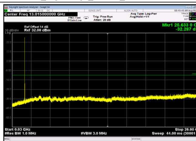
FDD04_LowRange_10MHz_30MHz~26GHz
