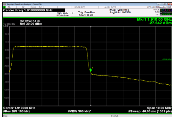
HighRange_FDD02_10MHz_1905_OneRB _high_Q16
