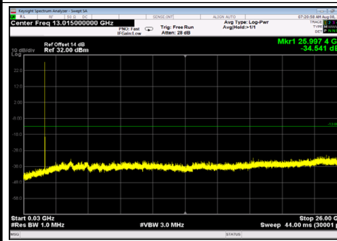
FDD66_MidRange_3MHz_30MHz~26GHz
