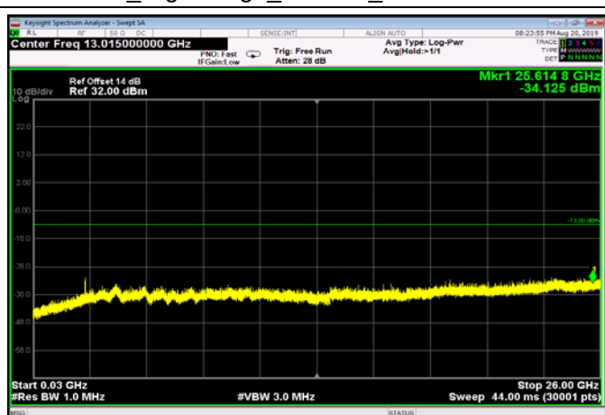
FDD66_HighRange_1.4MHz_30MHz~26GHz
