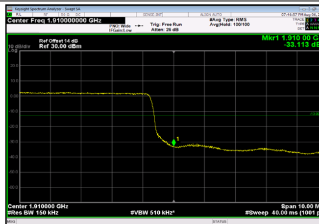
HighRange_FDD02_20MHz_1900_OneRB _high_QPSK
