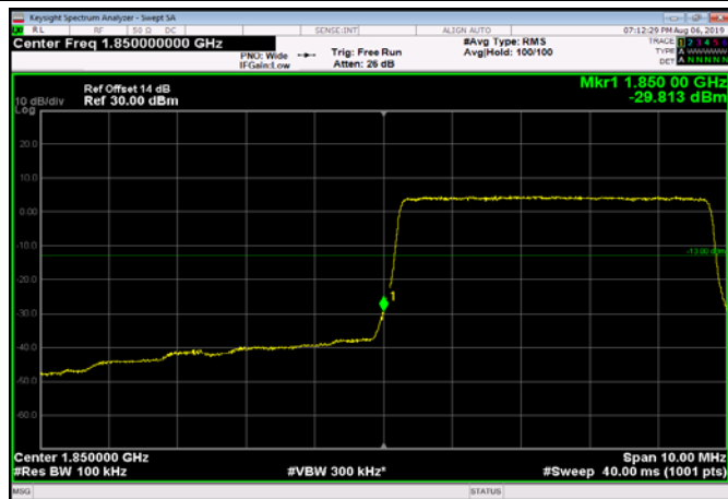
LowRange_FDD02_10MHz_1855_OneRB _low_Q16
