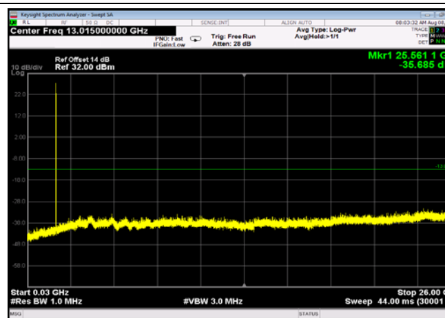
FDD04_HighRange_20MHz_30MHz~26GHz
