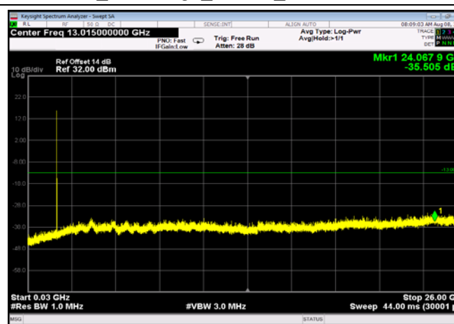
FDD66_LowRange_3MHz_30MHz~26GHz
