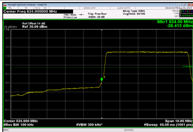
LowRange_FDD05_10MHz_829_OneRB _low_Q16
