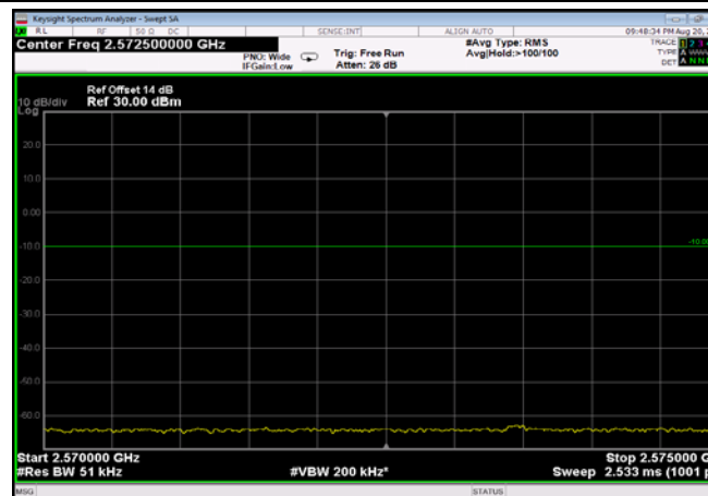
FDD07_5MHz_2502.5_QPSK_OneRB_high _ExtraBands_Range_2570~2575
