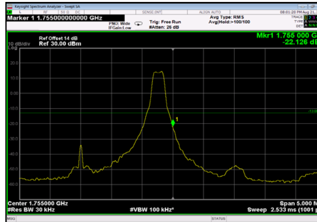
HighRange_FDD04_3MHz_1753.5_fullRB _High_QPSK
