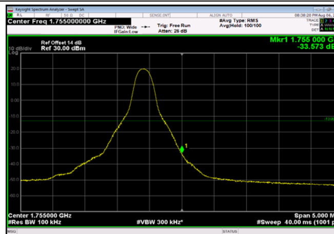
HighRange_FDD04_10MHz_1750_fullRB _High_QPSK
