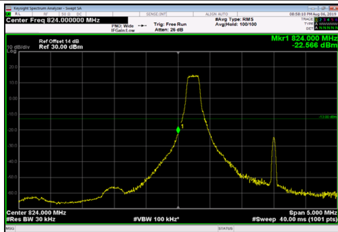
LowRange_FDD05_3MHz_825.5_fullIRB _Low_Q16
