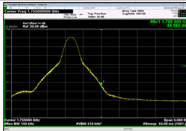
HighRange_FDD04_15MHz_1747.5_fullIRB _High_QPSK
