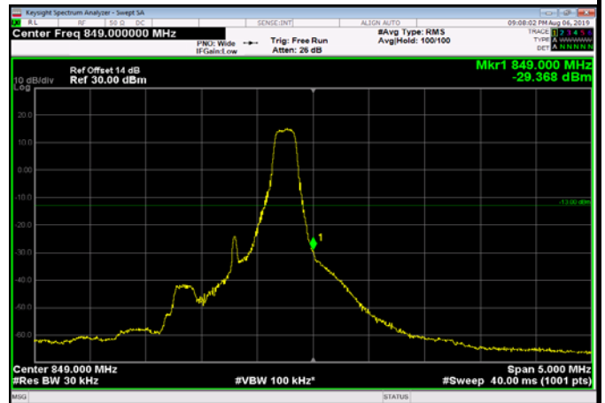
HighRange_FDD05_1.4MHz_848.3_fullIRB _High_Q16
