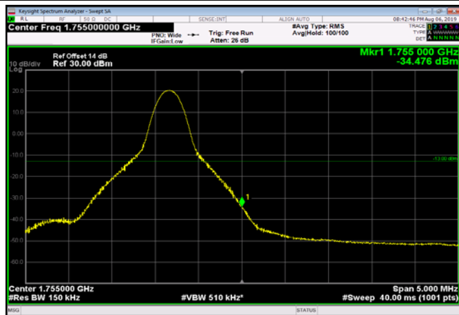
HighRange_FDD04_15MHz_1747.5_fullIRB _High_Q16
