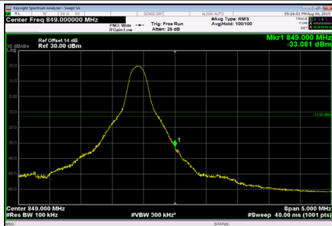
HighRange_FDD05_10MHz_844_fullIRB _High_Q16
