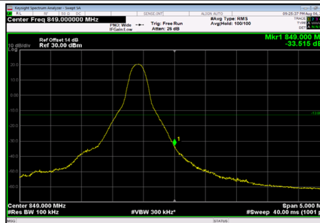
HighRange_FDD05_10MHz_844_fullIRB _High_QPSK
