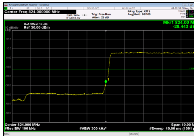
LowRange_FDD05_10MHz_829_OneRB _low_QPSK
