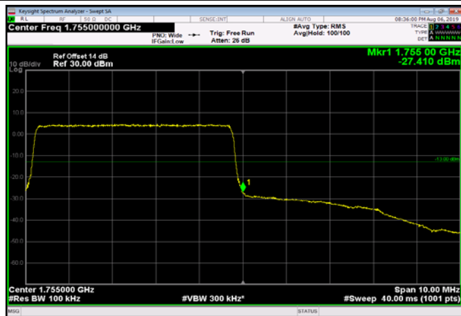
HighRange_FDD04_10MHz_1750_OneRB _high_Q16
