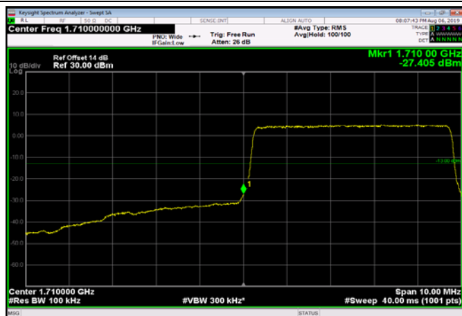
LowRange_FDD04_10MHz_1715_OneRB _low_Q16
