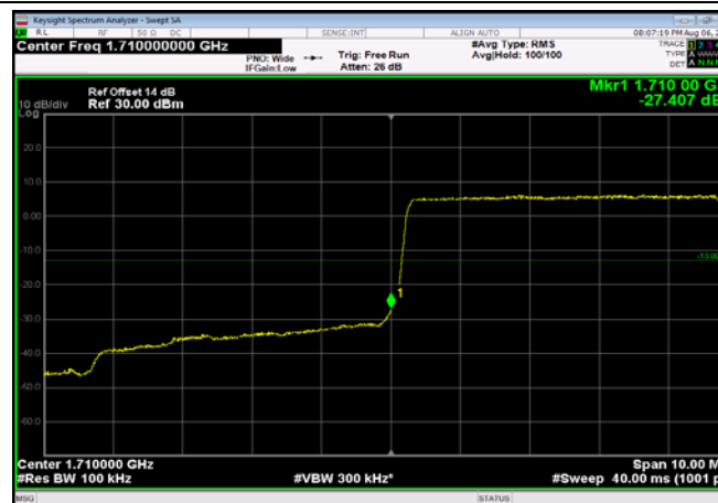
LowRange_FDD04_10MHz_1715_OneRB _low_QPSK
