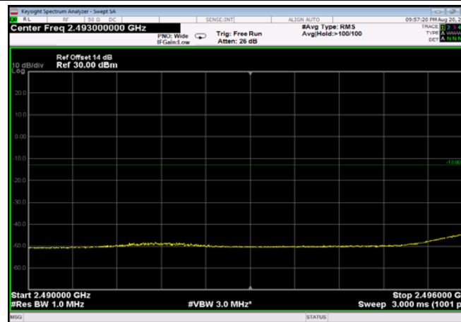
LowRange_FDD07_10MHz_2505_fullRB _Low_Q16
