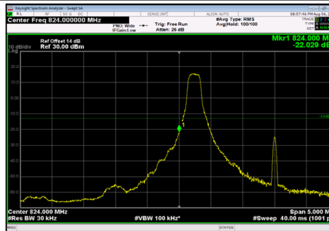
LowRange_FDD05_3MHz_825.5_fullIRB _Low_QPSK
