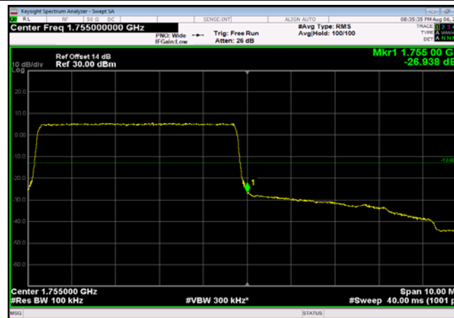
HighRange_FDD04_10MHz_1750_OneRB _high_QPSK
