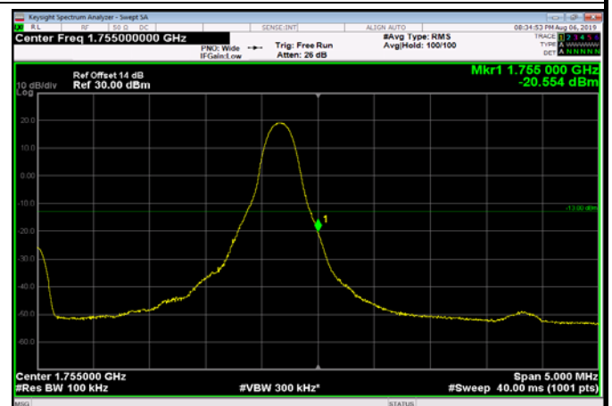
HighRange_FDD04_5MHz_1752.5_OneRB _high_Q16
