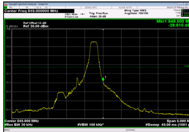
HighRange_FDD05_1.4MHz_848.3_fullIRB _High_QPSK
