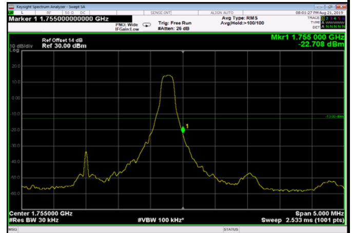
HighRange_FDD04_3MHz_1753.5_fullRB _High_Q16
