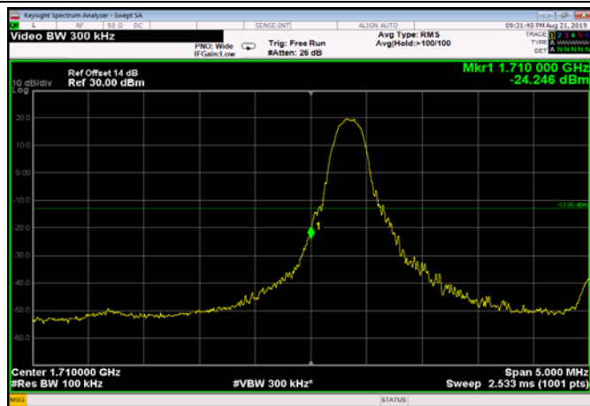
LowRange_FDD66_5MHz_1712.5_fullRB _Low_Q16
