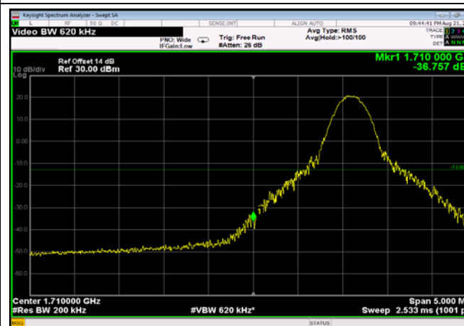
LowRange_FDD66_20MHz_1720_OneRB _low_QPSK
