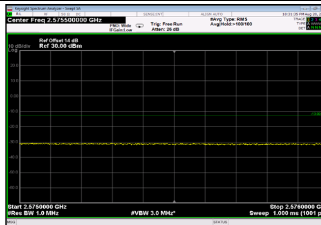
FDD07_15MHz_2562.5_QPSK_fullRB _ExtraBands_Range_2575~2576
