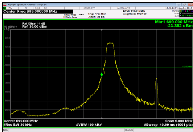
LowRange_FDD12_3MHz_700.5_fullIRB _Low_Q16
