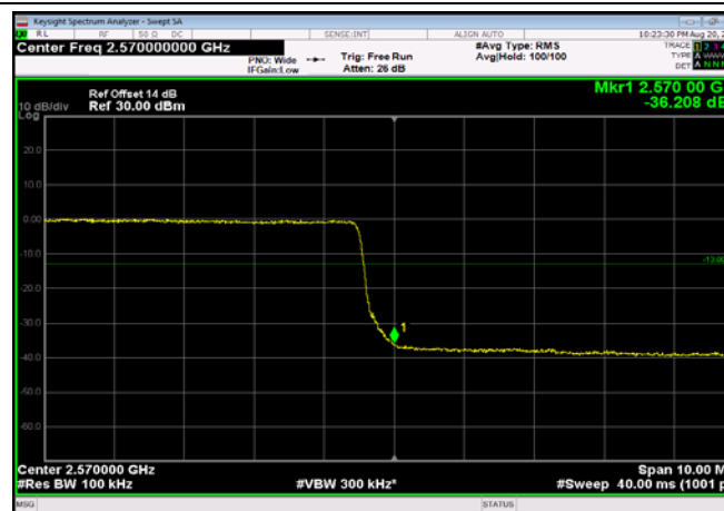
HighRange_FDD07_10MHz_2565_fullRB _High_Q16
