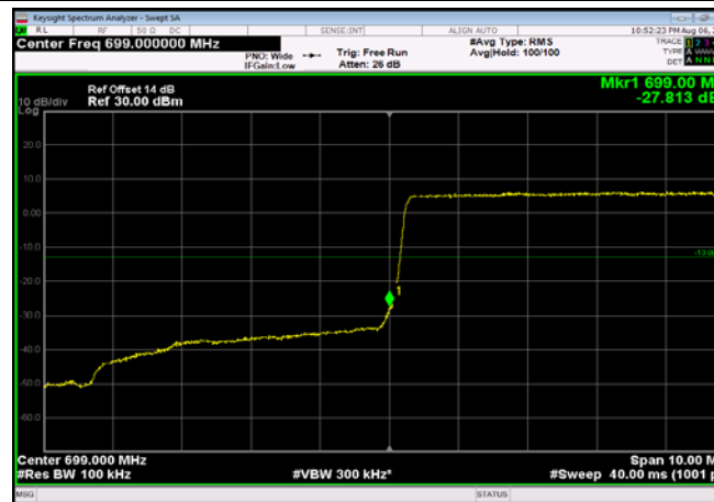
LowRange_FDD12_10MHz_704_OneRB _low_QPSK
