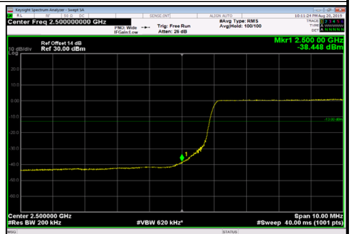
LowRange_FDD07_20MHz_2510_fullRB _Low_QPSK
