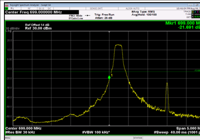
LowRange_FDD12_3MHz_700.5_fullIRB _Low_QPSK
