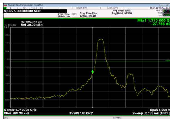
LowRange_FDD66_1.4MHz_1710.7_OneRB _low_QPSK
