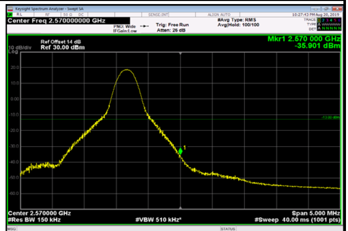
HighRange_FDD07_15MHz_2562.5_OneRB _high_Q16
