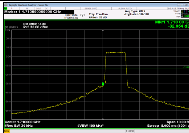
LowRange_FDD66_3MHz_1711.5_OneRB _low_QPSK
