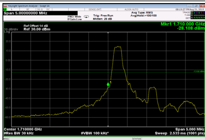
LowRange_FDD66_1.4MHz_1710.7_OneRB _low_Q16
