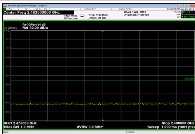
FDD07_10MHz_2565_QPSK_fullRB_ExtraBan ds_Range_2475~2490
