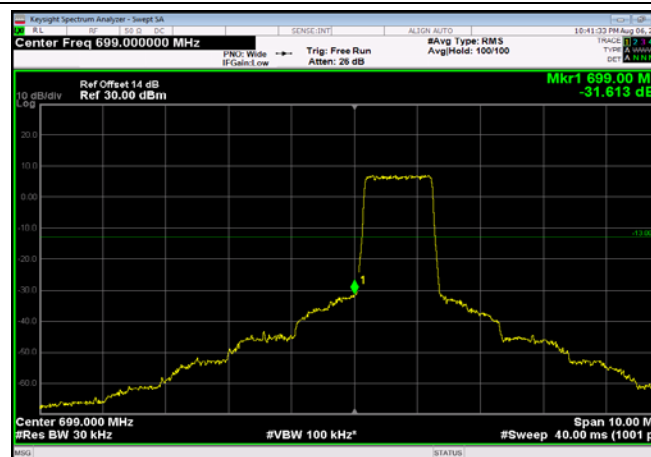
LowRange_FDD12_1.4MHz_699.7_fullRB _Low_QPSK
