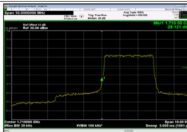
LowRange_FDD66_3MHz_1711.5_fullRB _Low_QPSK
