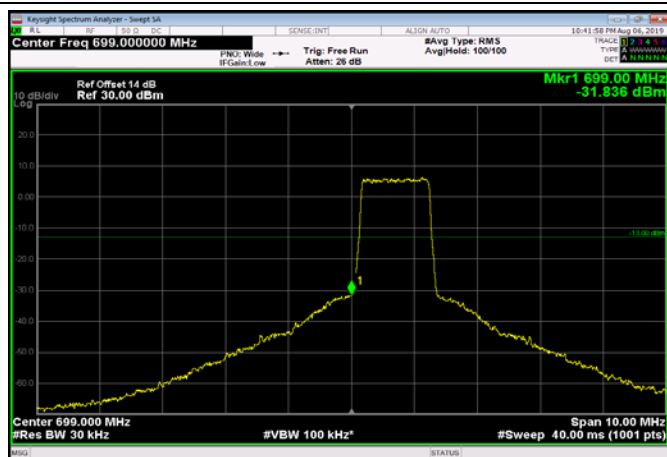
LowRange_FDD12_1.4MHz_699.7_fullRB _Low_Q16
