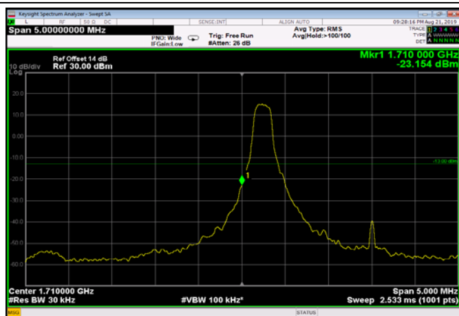
LowRange_FDD66_3MHz_1711.5_fullRB _Low_Q16
