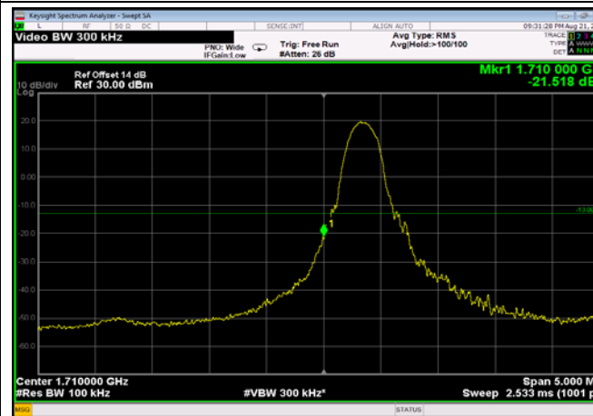
LowRange_FDD66_5MHz_1712.5_fullRB _Low_QPSK
