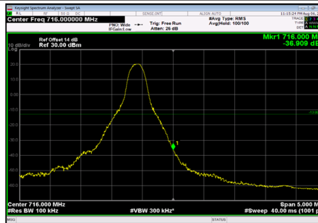
HighRange_FDD12_10MHz_711_fullRB _High_QPSK
