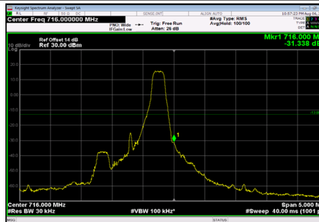
HighRange_FDD12_1.4MHz_715.3_fullIRB _High_QPSK
