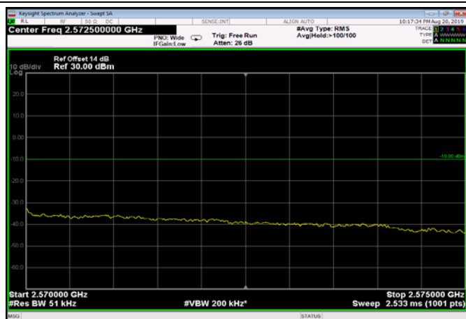
FDD07_5MHz_2567.5_QPSK_fullRB_ExtraBa nds_Range_2570~2575
