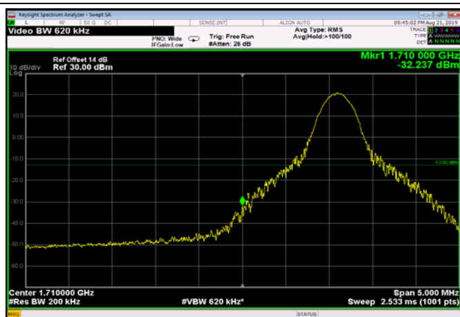
LowRange_FDD66_20MHz_1720_OneRB _low_Q16
