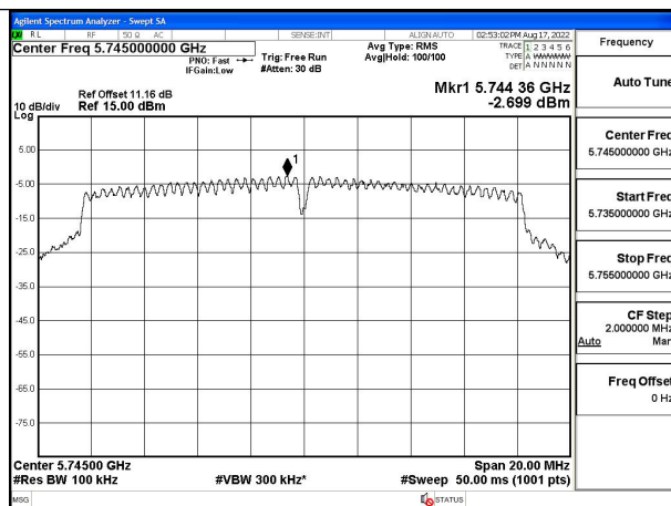
Test Mode:802.11n HT20 5745MHz Chain1
