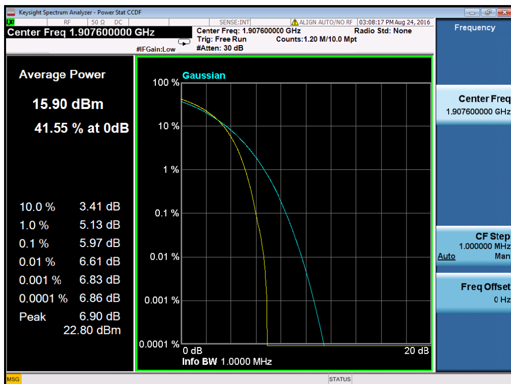
(Plot D3: WCDMA 1900MHz Channel = 9538)
