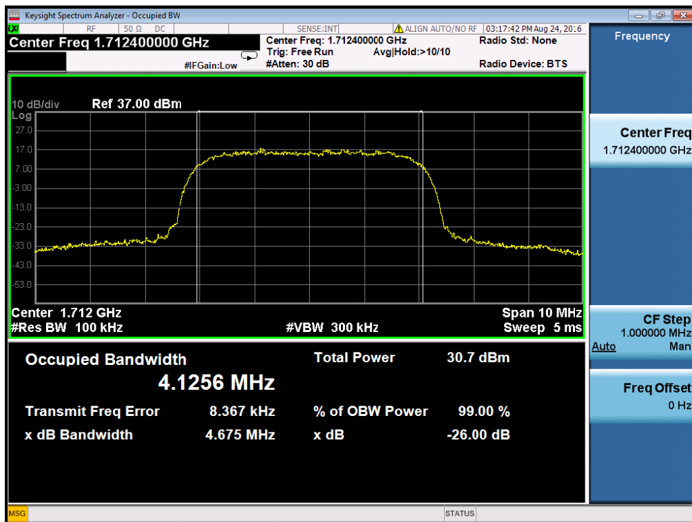
(Plot G1: WCDMA 1700MHz Channel = 1312)
