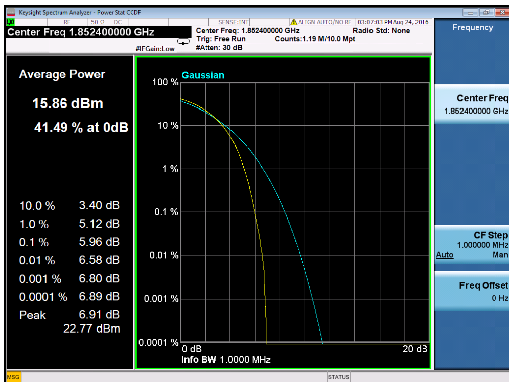
(Plot D1: WCDMA 1900MHz Channel = 9262)
