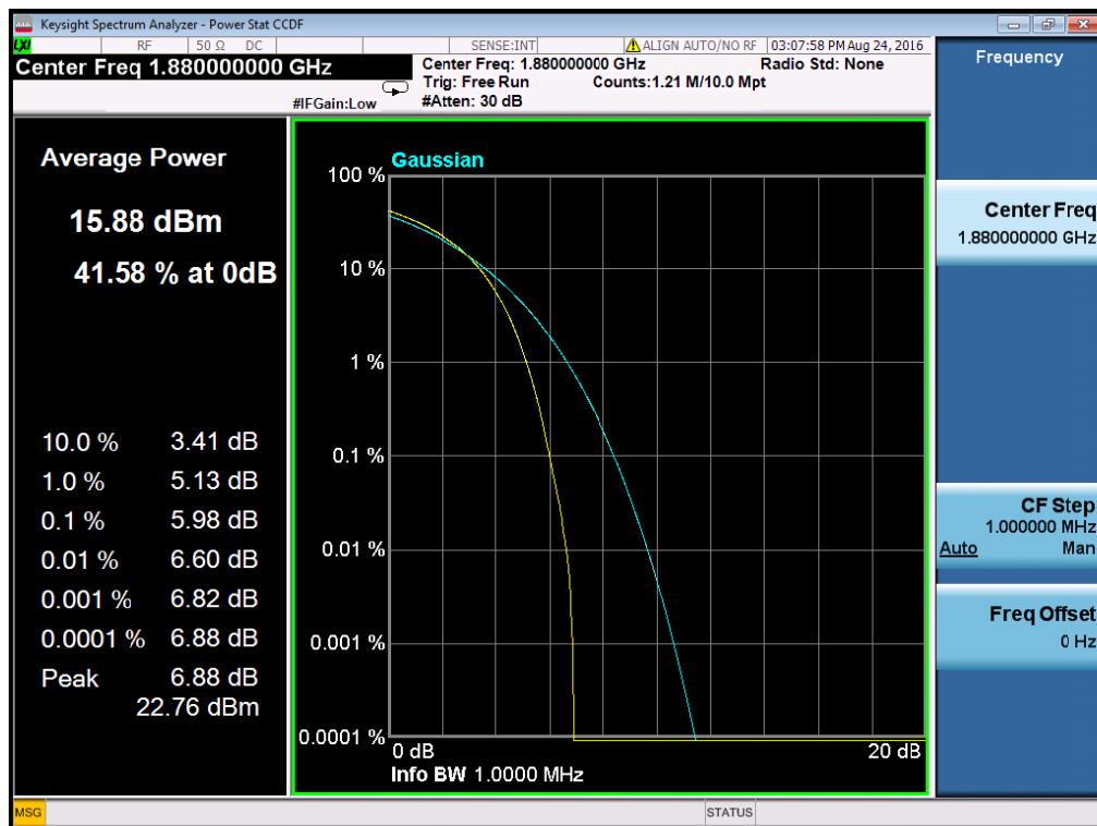
(Plot D2: WCDMA 1900MHz Channel = 9400)
