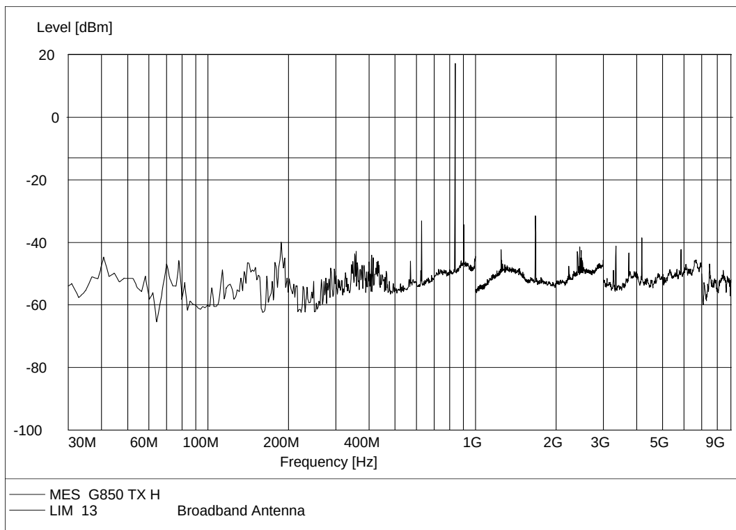
GPRS 850MHz, Test Antenna Horizontal
