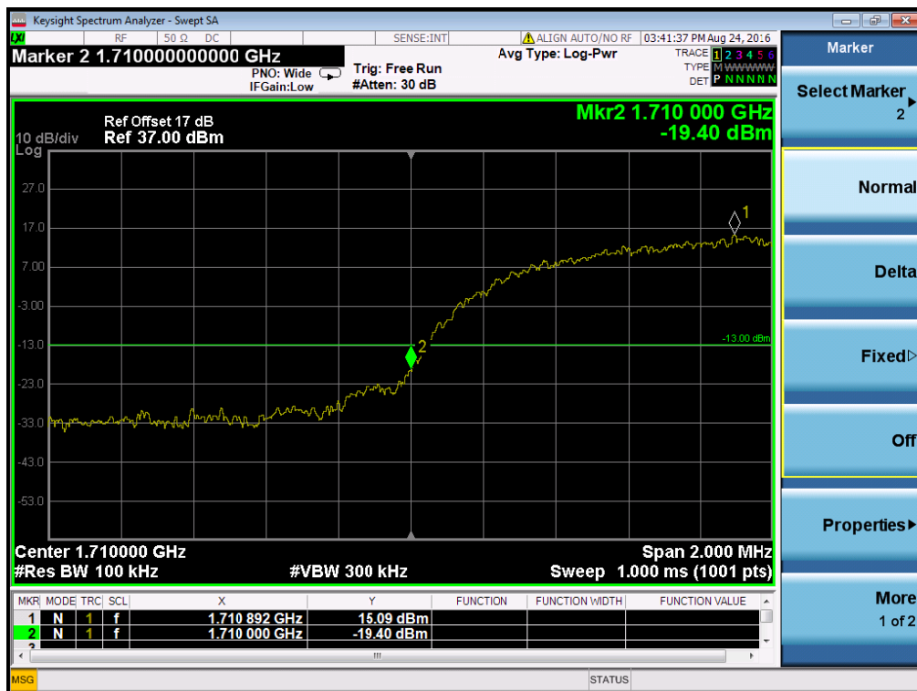
(Plot M: WCDMA 1700 Channel = 1312)
