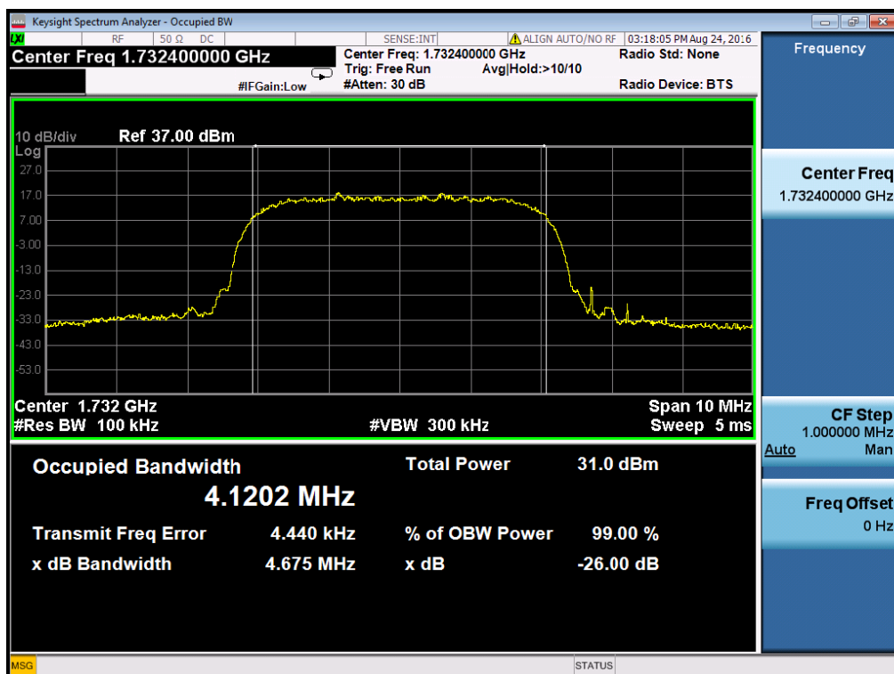
(Plot G2: WCDMA 1700MHz Channel = 1412)
