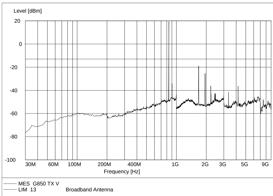
GPRS 850MHz, Test Antenna Vertical
