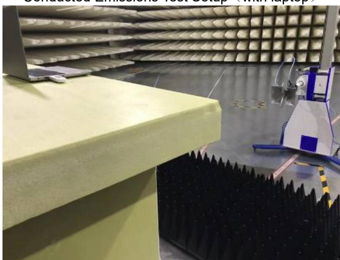
Conducted Emissions Test Setup (with laptop)
