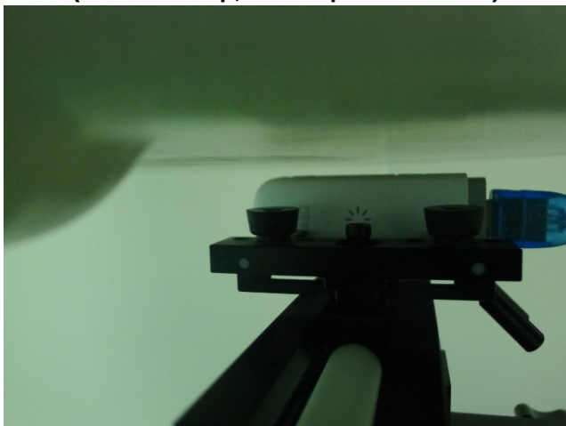
USB Cable Plug-in for USB Configuration 3 (Vertical Front, Test Separation 5 mm)
