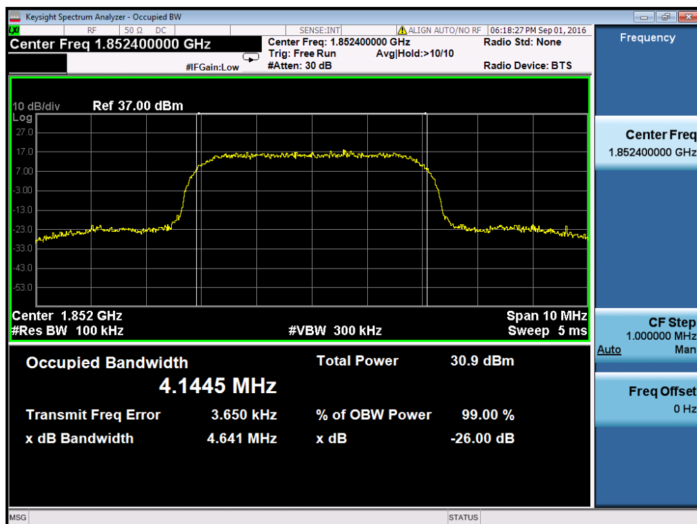
(Plot F1: WCDMA 1900MHz Channel = 9262 Occupied bandwidth)
