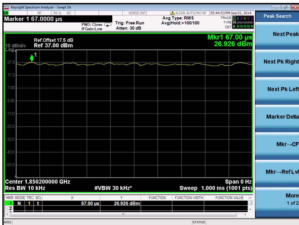
(Plot A1: GPRS 1900 MHz Channel = 512)
