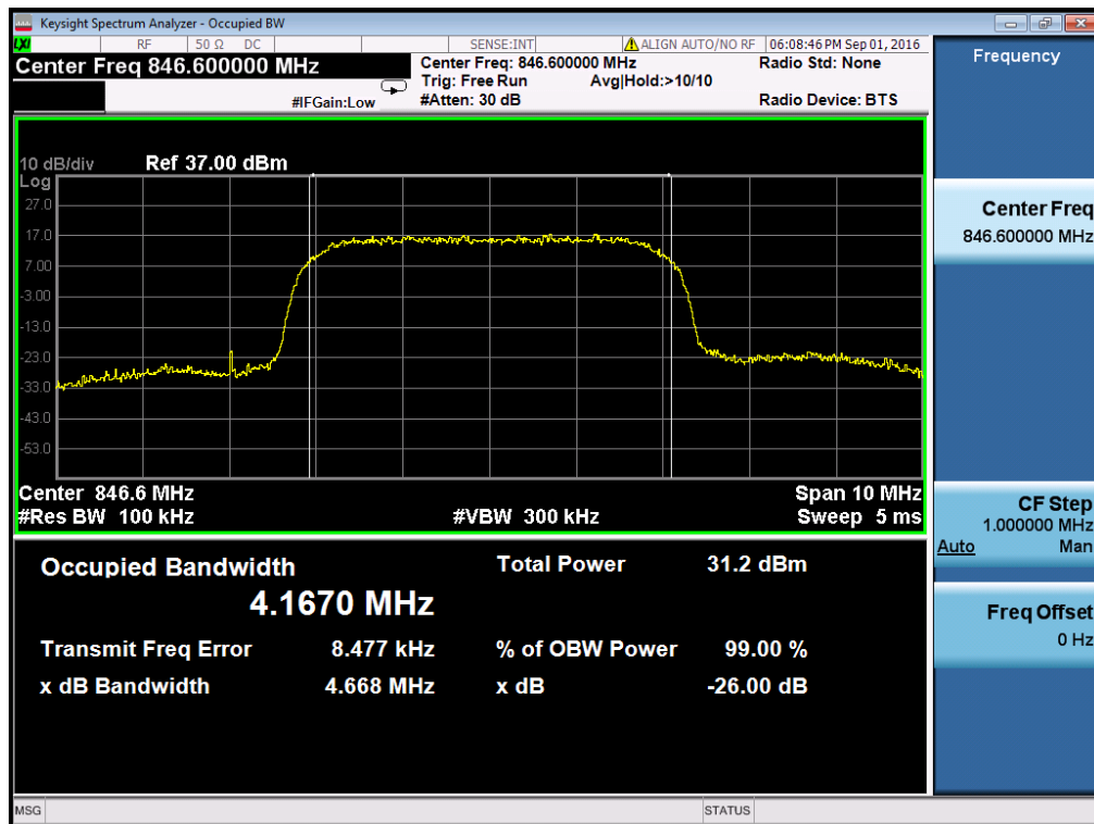
(Plot E3: WCDMA 850MHz Channel = 4233 Occupied bandwidth)
