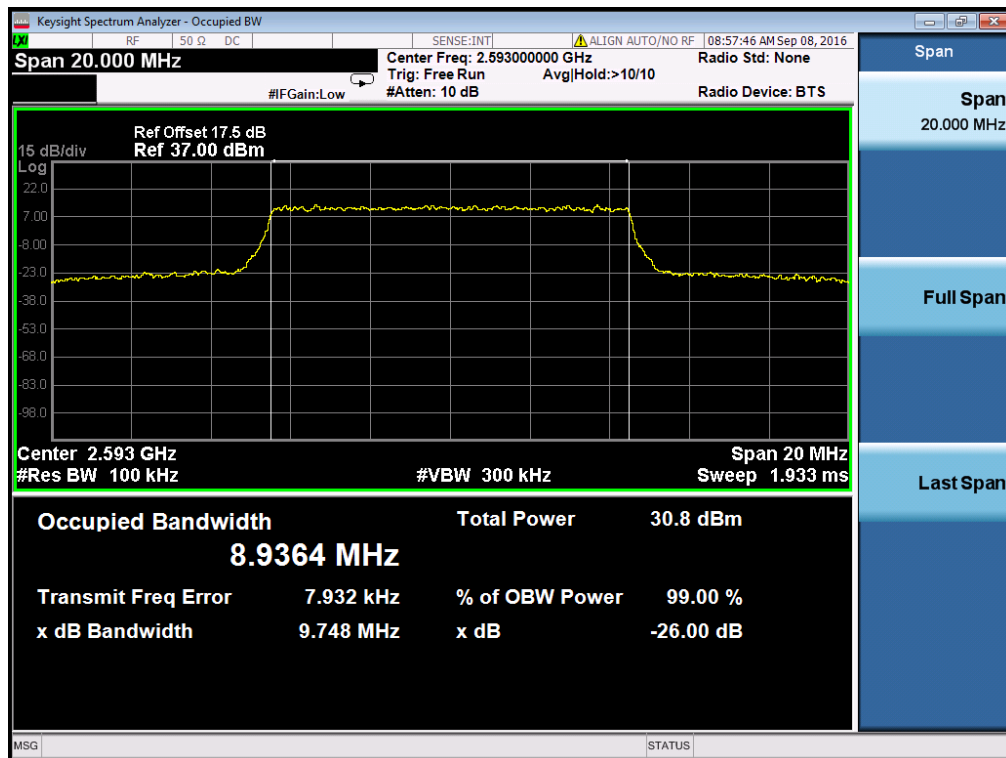
Occupied Bandwidth LTE Band 41/10MHz/QPSK
