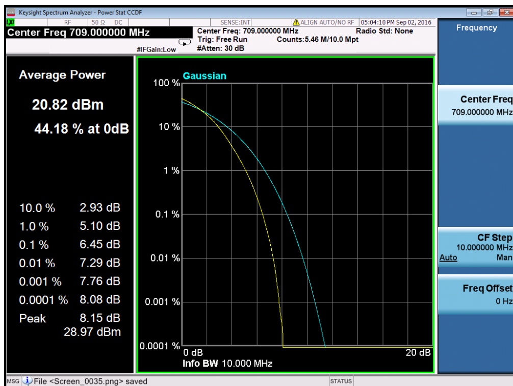
(Plot C4: Band 17/10MHz/16QAM in M Ch 50RB Size)
