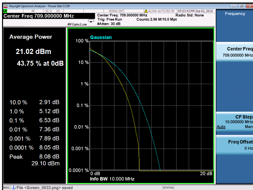
(Plot C2: Band 17/10MHz/16QAM in L Ch 50RB Size)
