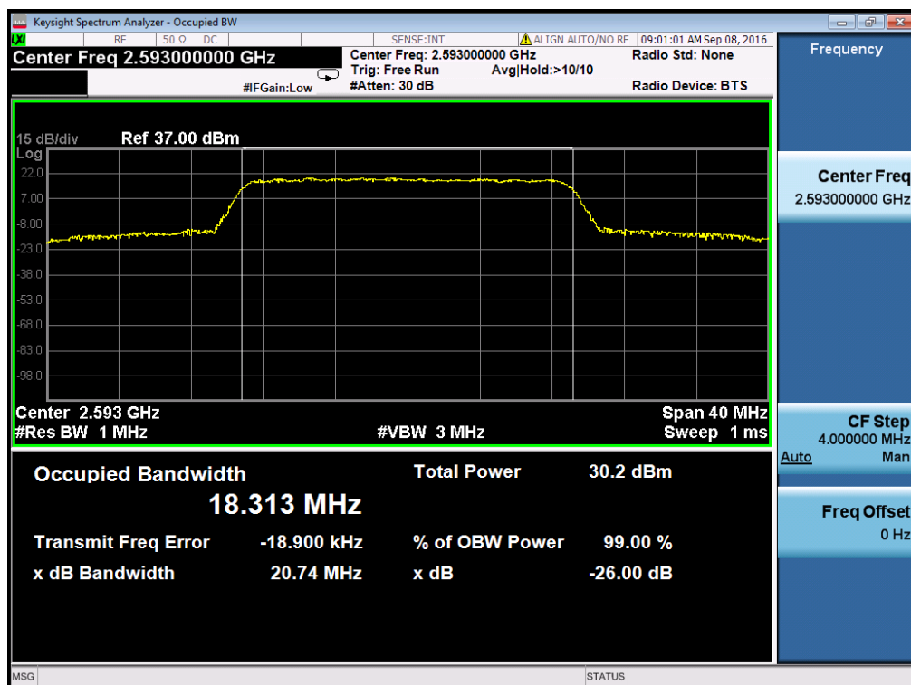
Occupied Bandwidth LTE Band 41/20MHz/16QAM
