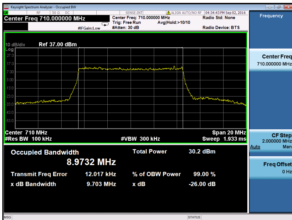
Occupied Bandwidth LTE Band 17/10MHz/16QAM
