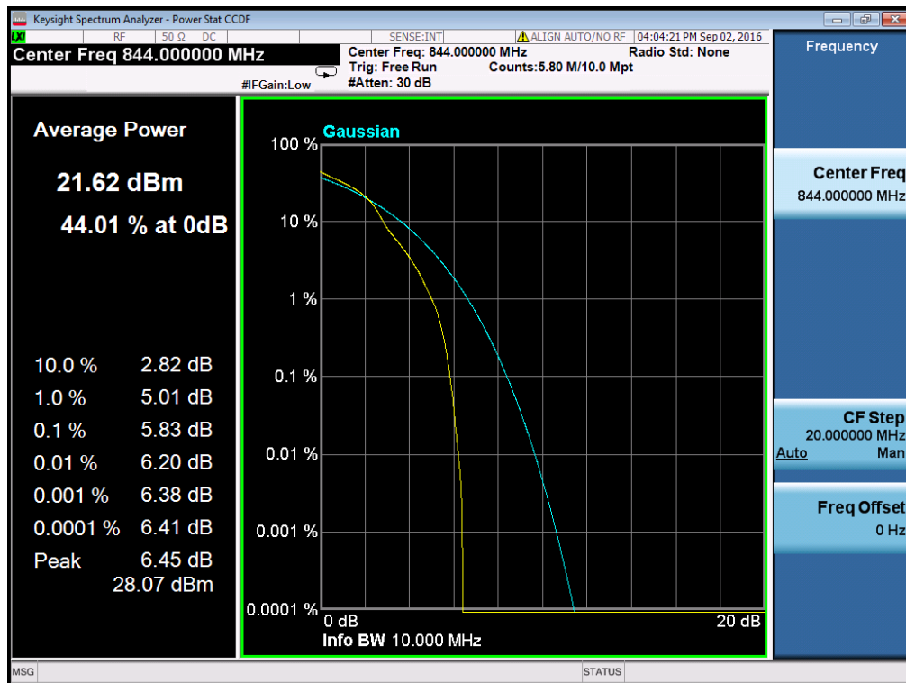
(Plot B5: Band 5/10MHz/16QAM in H Ch 1RB Size)
