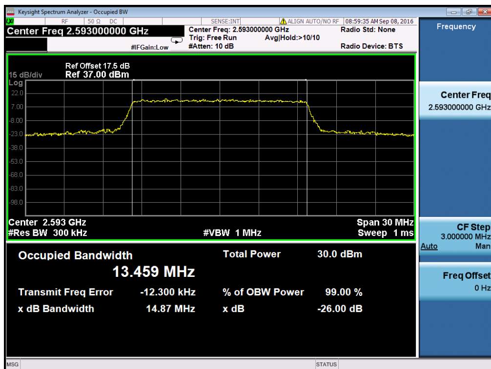
Occupied Bandwidth LTE Band 41/15MHz/16QAM
