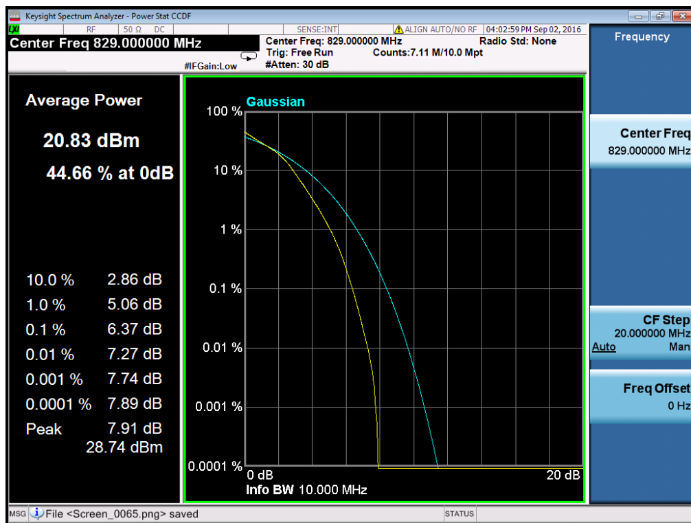
(Plot B2: Band 5/10MHz/16QAM in L Ch 50RB Size)
