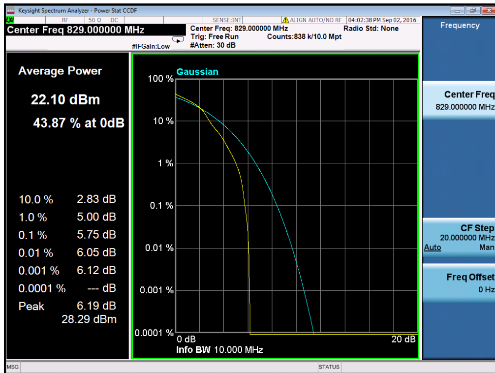
(Plot B1: Band 5/10MHz/16QAM in L Ch 1RB Size )
