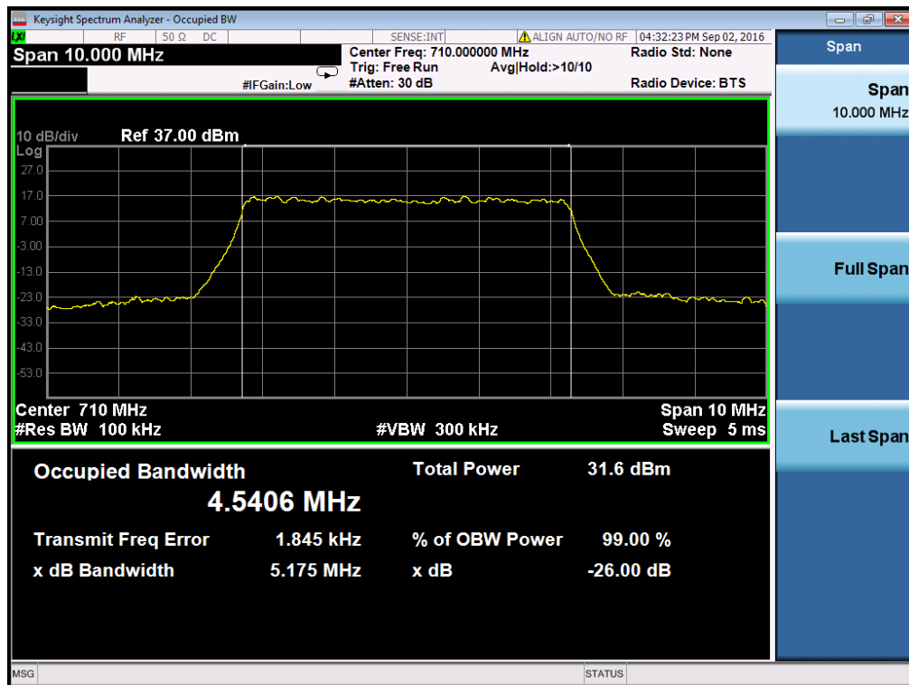
Occupied Bandwidth LTE Band 17/5MHz/QPSK
