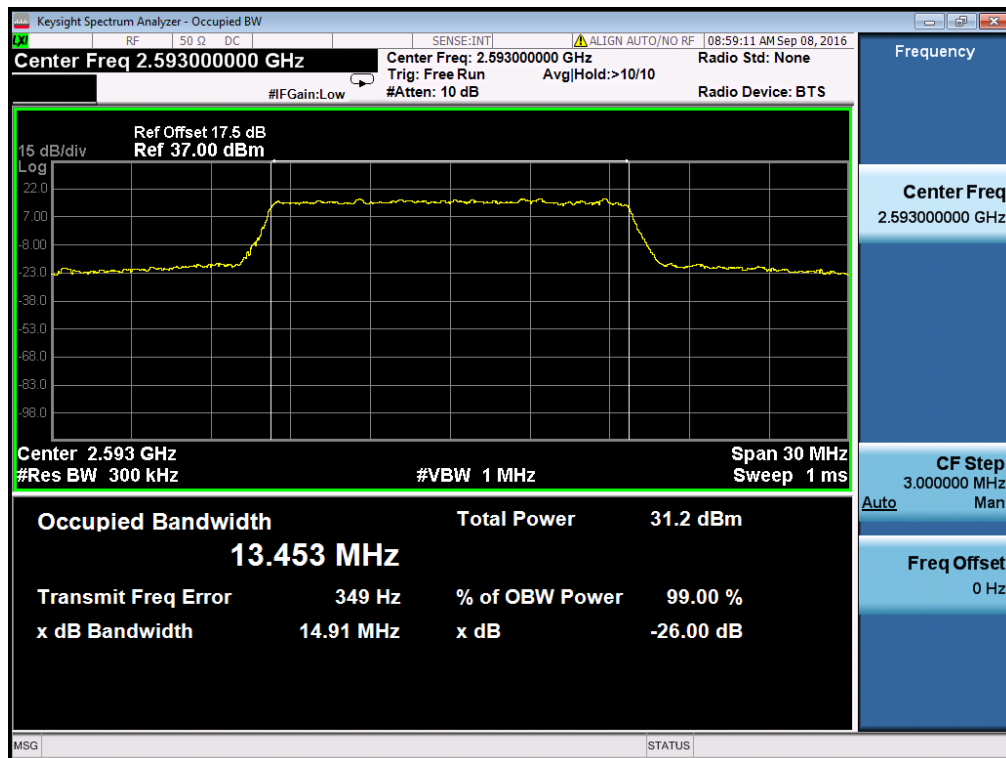
Occupied Bandwidth LTE Band 41/15MHz/QPSK
