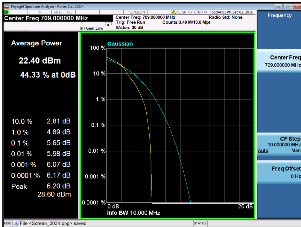
(Plot C3: Band 17/10MHz/16QAM in M Ch 1RB Size)
