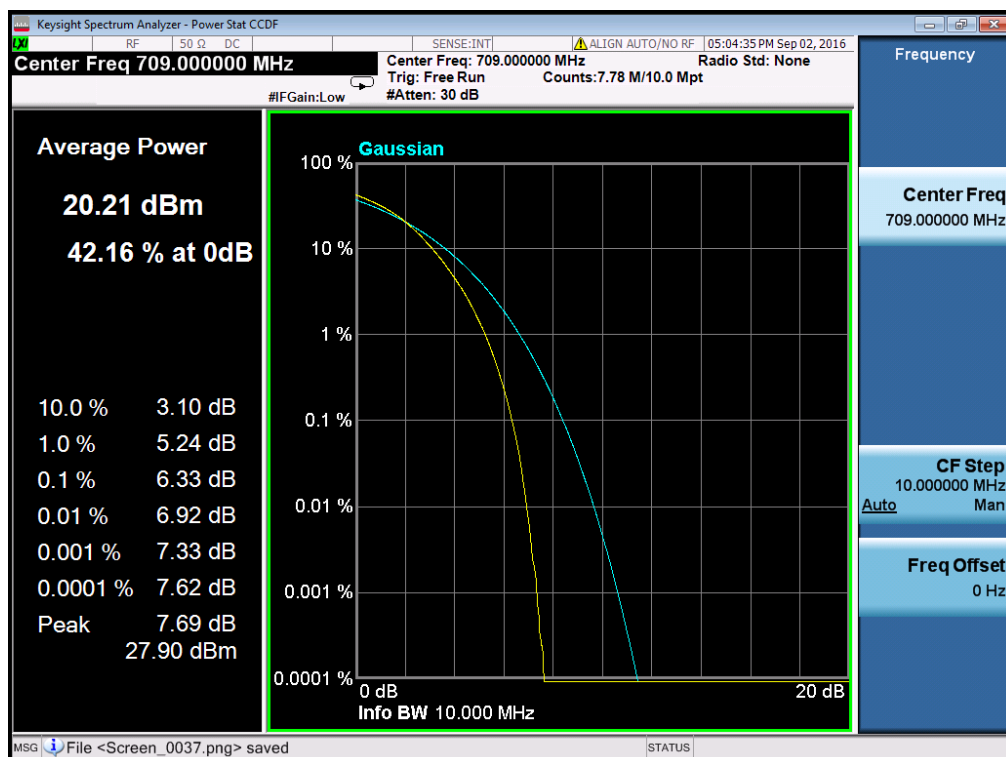
(Plot C6: Band 17/10MHz/16QAM in H Ch 50RB Size)
