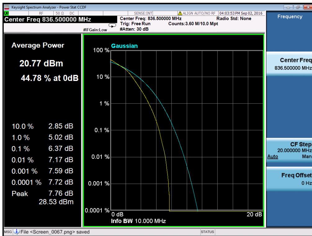
(Plot B4: Band 5/10MHz/16QAM in M Ch 50RB Size)
