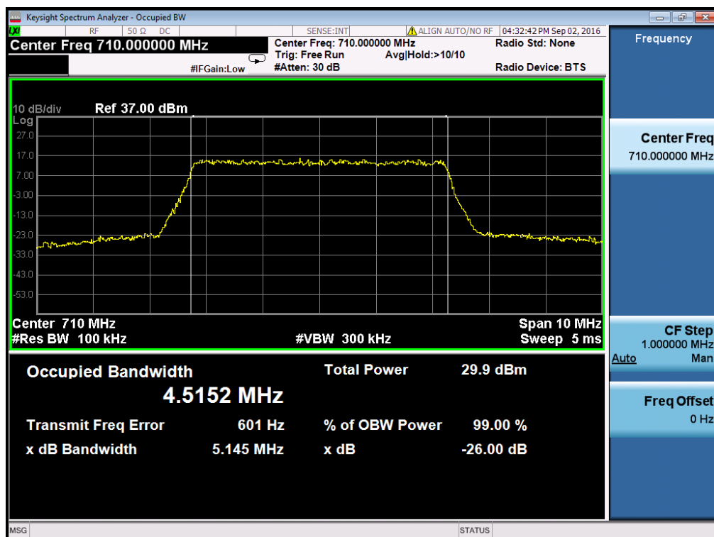
Occupied Bandwidth LTE Band 17/5MHz/16QAM
