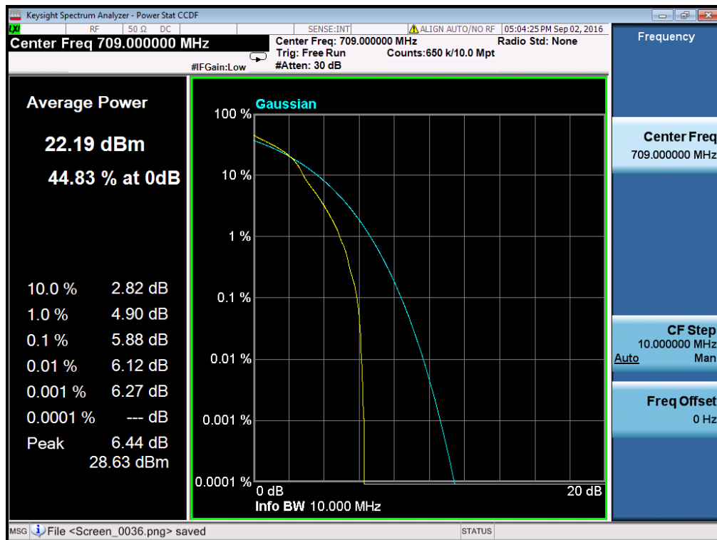
(Plot C5: Band 17/10MHz/16QAM in H Ch 1RB Size)
