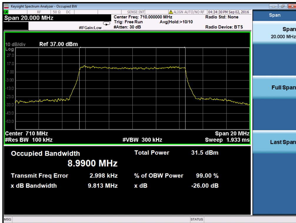
Occupied Bandwidth LTE Band 17/10MHz/QPSK
