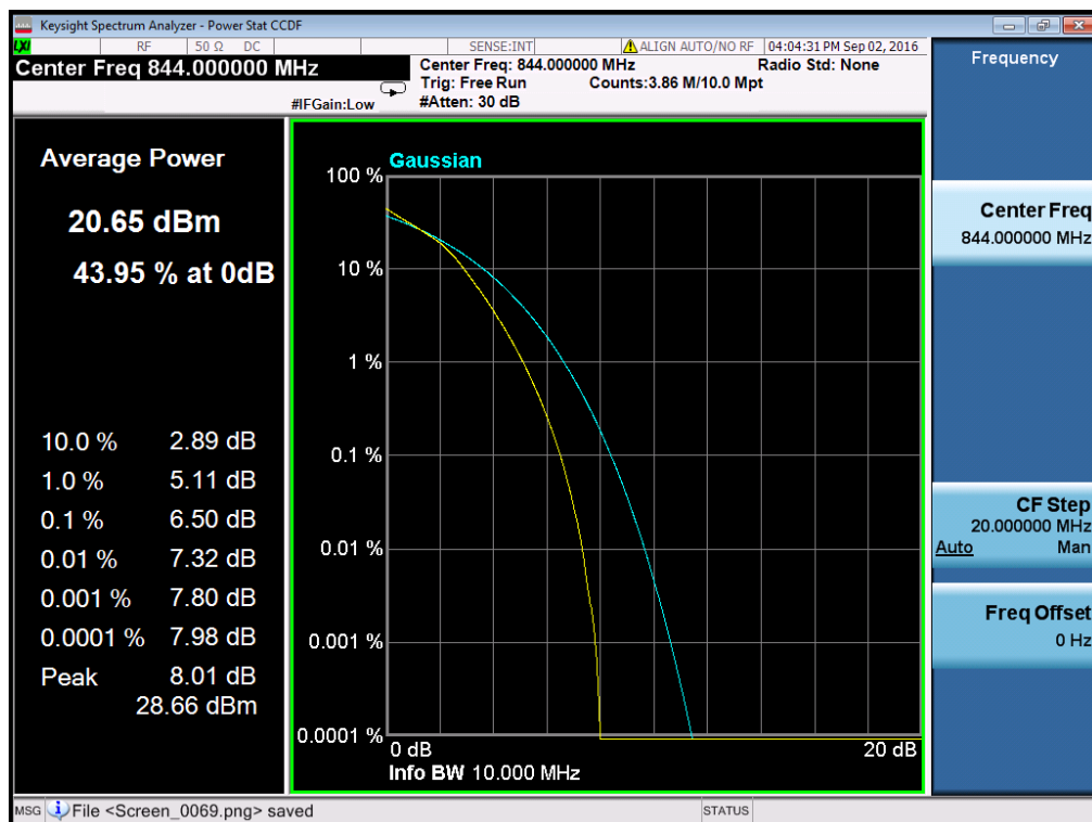
(Plot B6: Band 5/10MHz/16QAM in H Ch 50RB Size)
