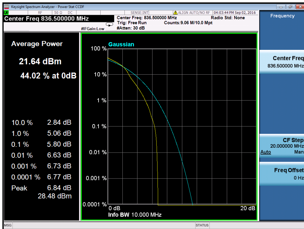
(Plot B3: Band 5/10MHz/16QAM in M Ch 1RB Size)
