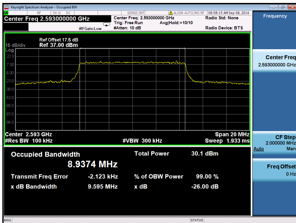
Occupied Bandwidth LTE Band 41/10MHz/16QAM
