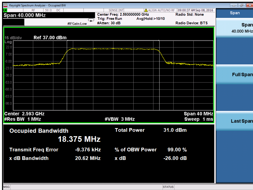
Occupied Bandwidth LTE Band 41/20MHz/QPSK
