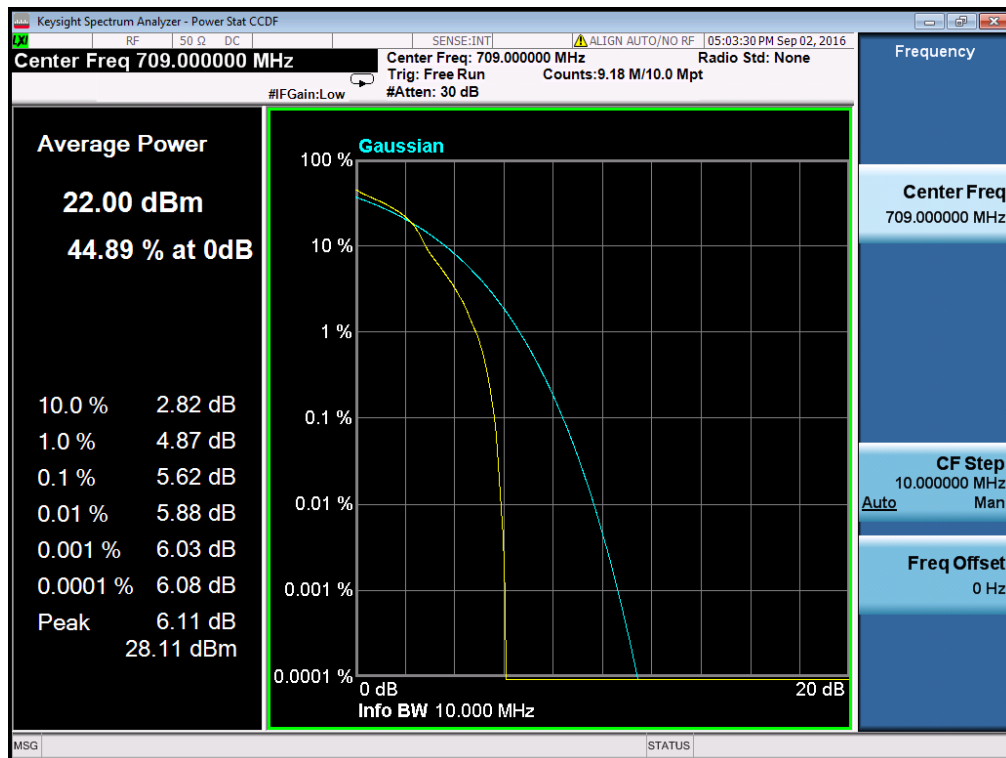
(Plot C1: Band 17/10MHz/16QAM in L Ch 1RB Size )
