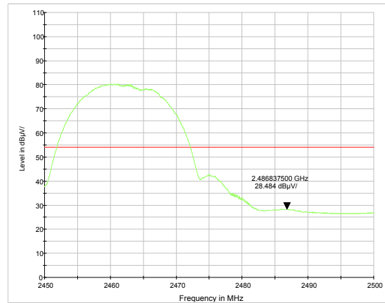
802.11g-Channel 11: Peak
