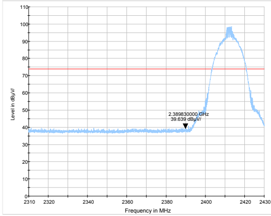
802.11b-Channel 1: Average
