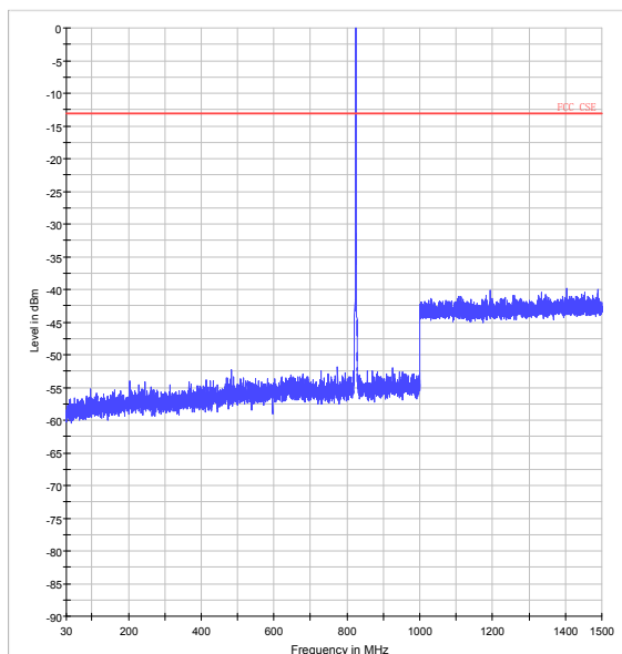
LTE Band 5 1.4MHz CH-Middle 30MHz~1.5GHz
