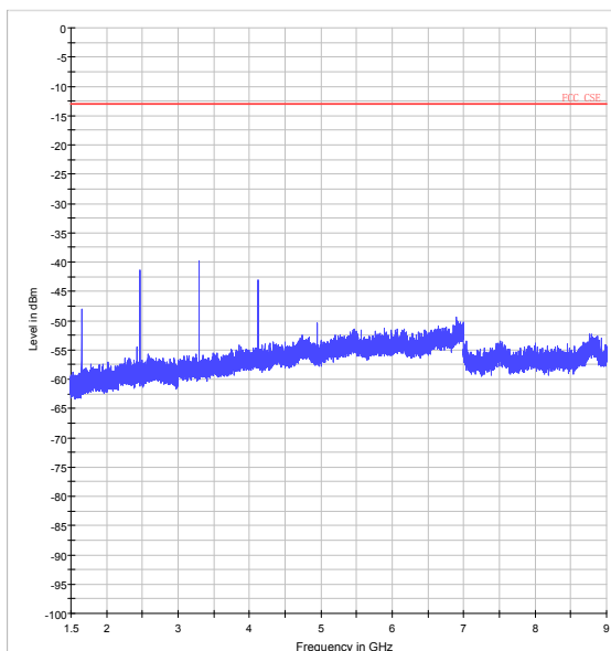
LTE Band 5 1.4MHz CH-Middle 1.5GHz~9GHz
