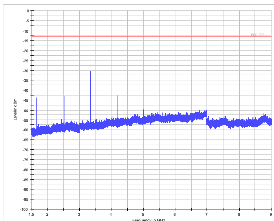
LTE Band 5 3MHz CH-High 1.5GHz~9GHz
