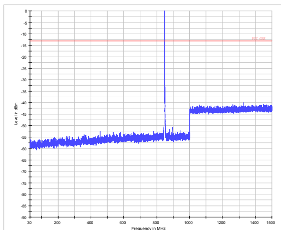
LTE Band 5 1.4MHz CH-High 30MHz~1.5GHz
