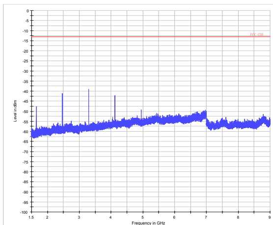
LTE Band 5 3MHz CH-Middle 1.5GHz~9GHz
