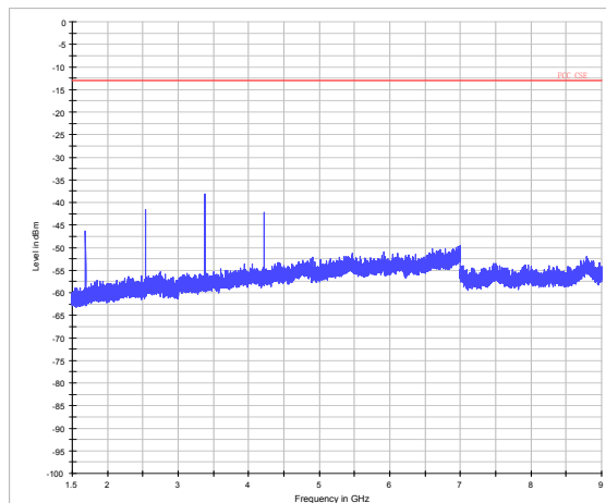
LTE Band 5 5MHz CH-High 1.5GHz~9GHz
