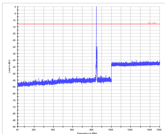
LTE Band 5 5MHz CH-High 30MHz~1.5GHz
