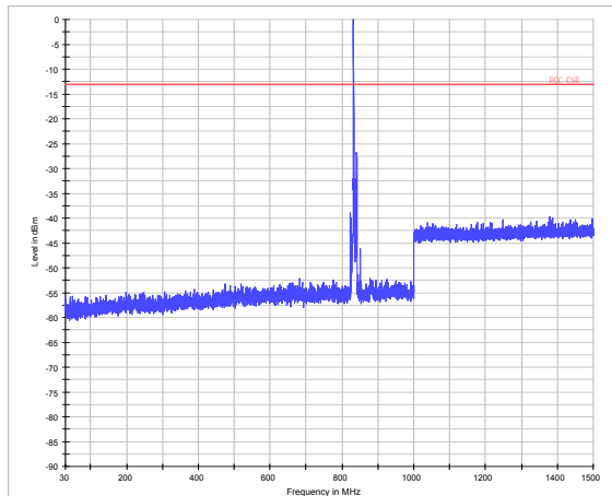
LTE Band 5 10MHz CH-High 30MHz~1.5GHz
