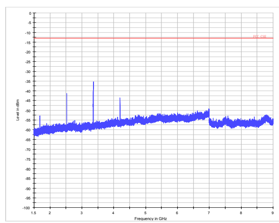
LTE Band 5 10MHz CH-High 1.5GHz~9GHz
