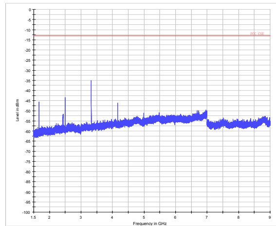
LTE Band 5 10MHz CH-High 1.5GHz~9GHz
