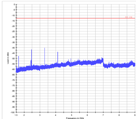
LTE Band 5 5MHz CH-Middle 1.5GHz~9GHz
