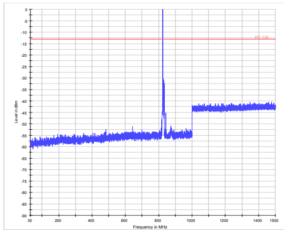
LTE Band 5 10MHz CH-Low 30MHz~1.5GHz
