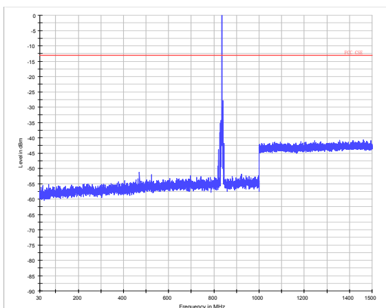
LTE Band 5 3MHz CH-High 30MHz~1.5GHz
