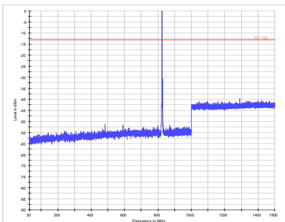
LTE Band 5 3MHz CH-Middle 30MHz~1.5GHz
