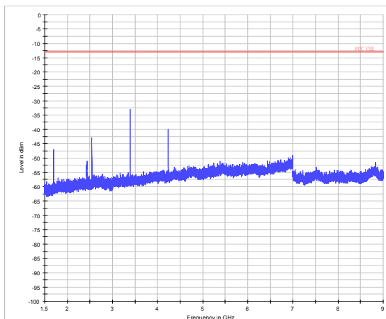
LTE Band 5 1.4MHz CH-High 1.5GHz~9GHz
