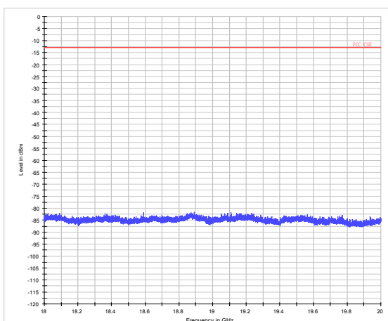
LTE Band 2 5MHz CH-High 18GHz~20GHz
