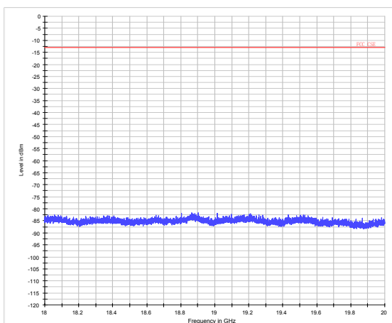
LTE Band 2 10MHz CH-Middle 18GHz~20GHz
