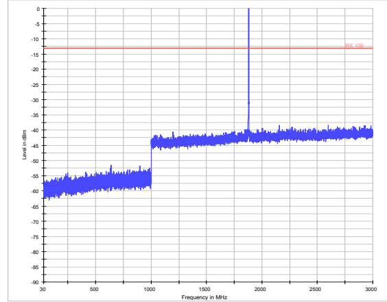
LTE Band 2 1.4MHz CH-Middle 30MHz~3GHz
