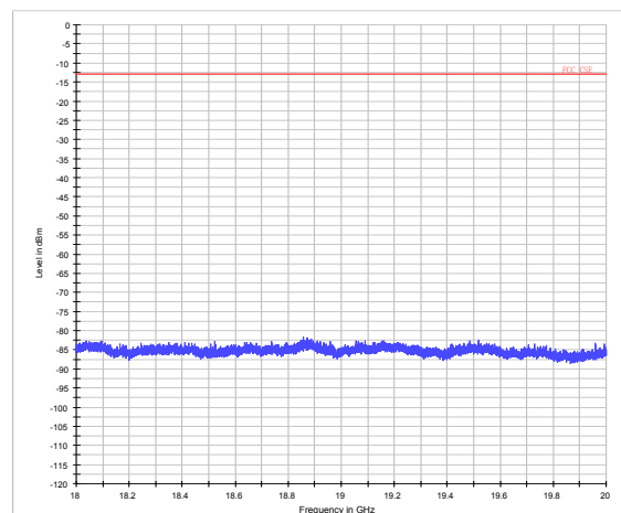
LTE Band 2 3MHz CH-Low 18GHz~20GHz
