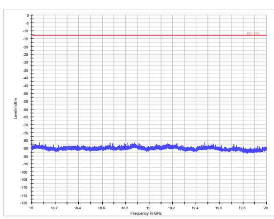
LTE Band 2 20MHz CH-Low 18GHz~20GHz
