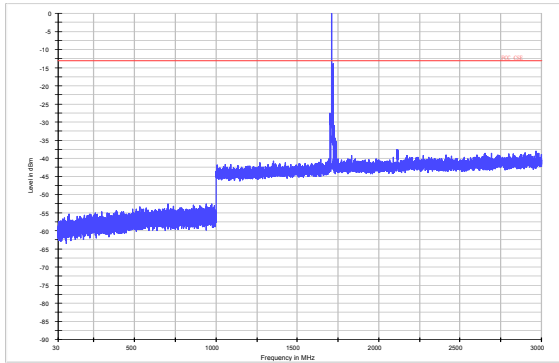
LTE Band 4 10MHz CH-Middle 30MHz~3GHz
