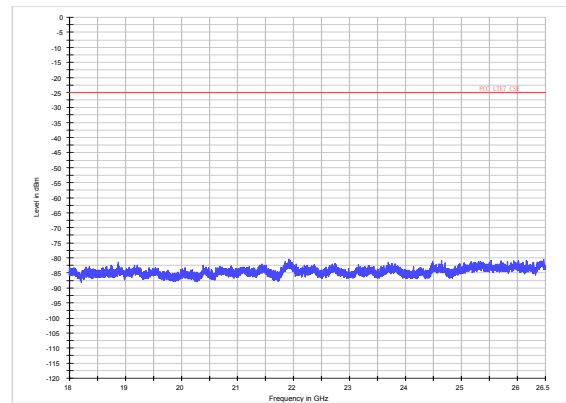
LTE Band 7 10MHz CH-High 18GHz~26.5GHz
