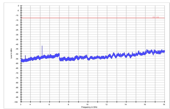
LTE Band 4 3MHz CH-High 3GHz~18GHz
