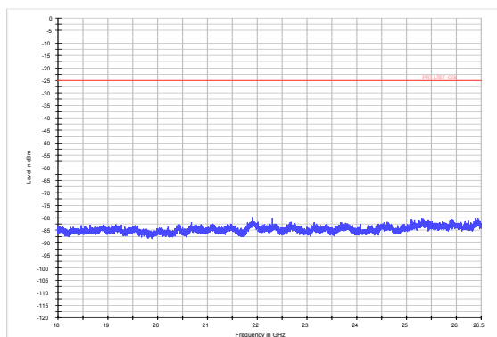
LTE Band 7 15MHz CH-High 18GHz~26.5GHz
