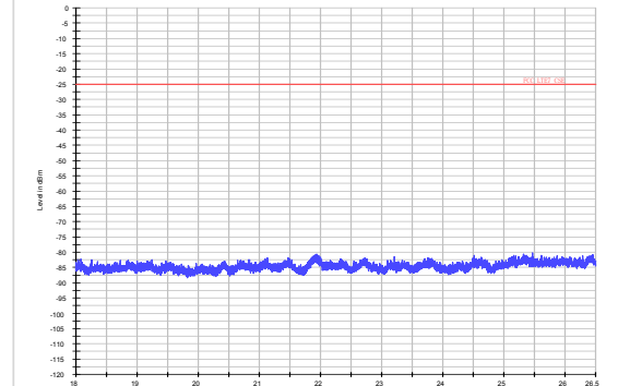
LTE Band 7 15MHz CH-Middle 18GHz~26.5GHz
