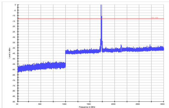
LTE Band 4 15MHz CH-High 30MHz~3GHz
