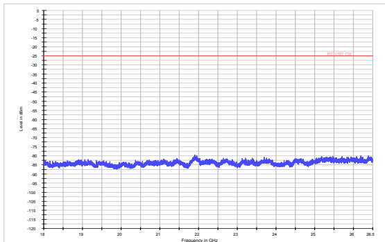
LTE Band 7 5MHz CH-High 18GHz~26.5GHz
