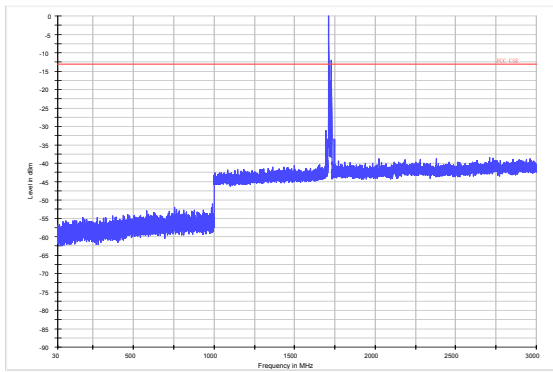
LTE Band 4 20MHz CH-Middle 30MHz~3GHz
