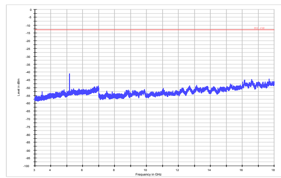
LTE Band 4 15MHz CH-High 3GHz~18GHz
