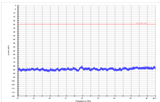
LTE Band 7 15MHz CH-Low 18GHz~26.5GHz
