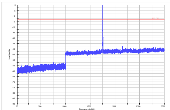
LTE Band 4 3MHz CH-High 30MHz~3GHz
