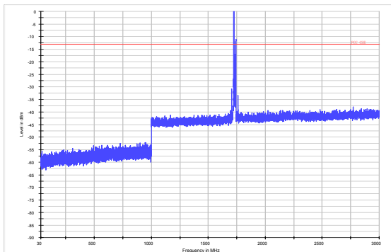
LTE Band 4 20MHz CH-High 30MHz~3GHz
