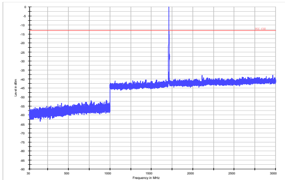
LTE Band 4 3MHz CH-Middle 30MHz~3GHz
