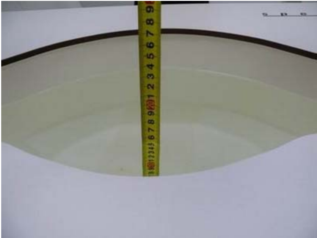
Picture 9: Liquid depth in the flat Phantom (5250 MHz, 15.3cm depth)
