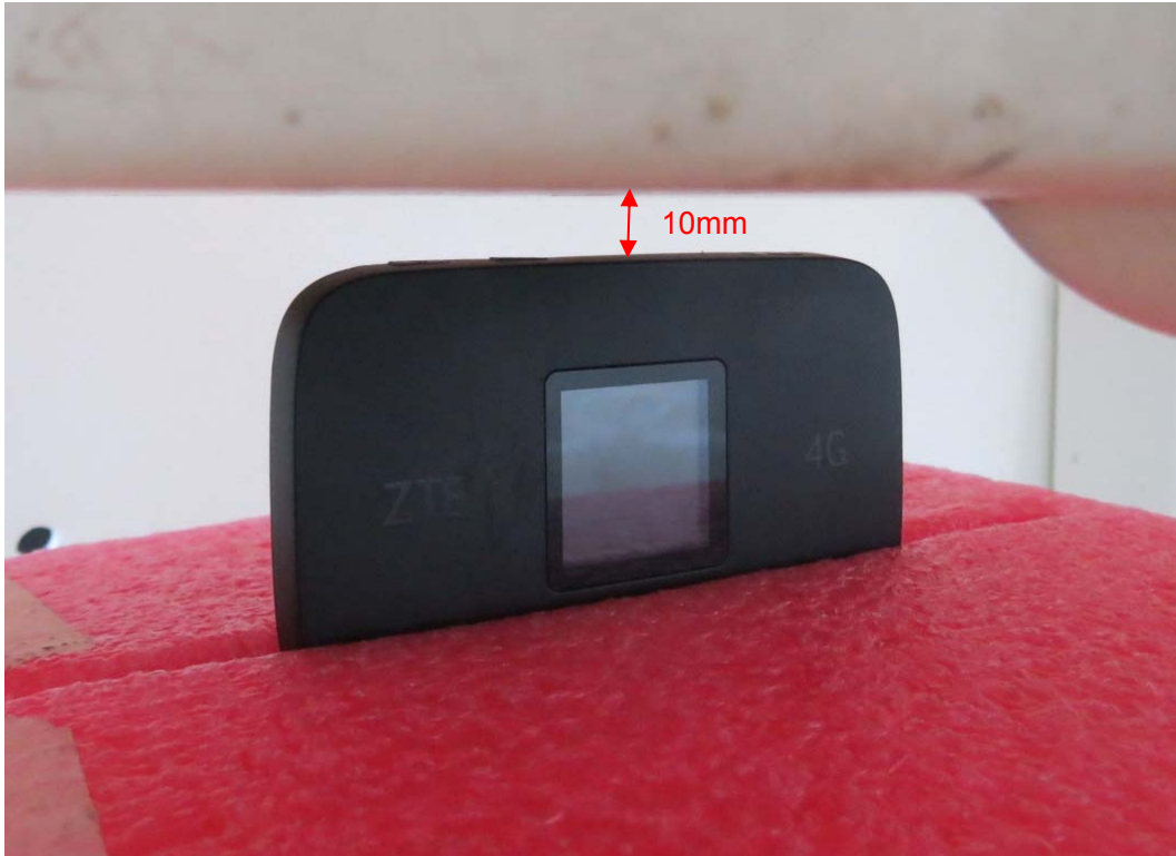
Picture 15: Top Edge, the distance from EUT to the bottom of the Phantom is 10mm
