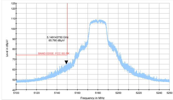
802.11a-Channel 36: Peak
