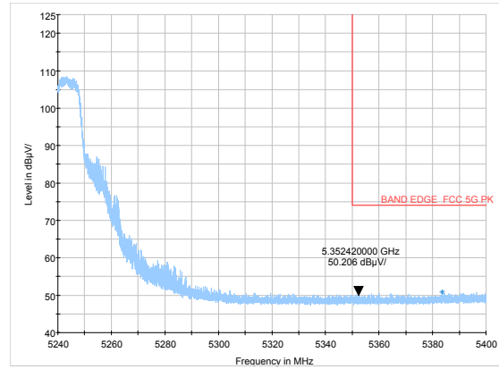
802.11a-Channel 48: Peak
