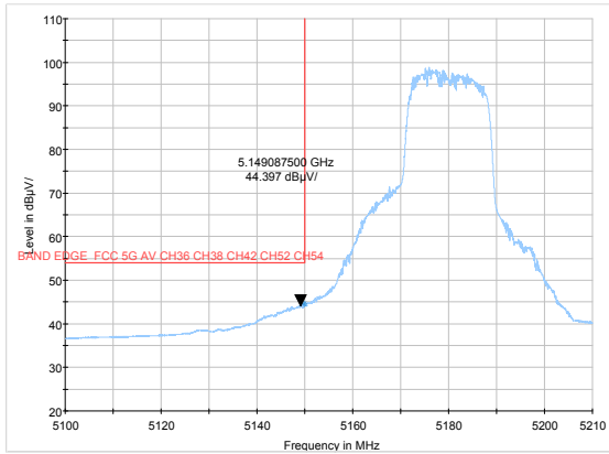
802.11a-Channel 36: Average
