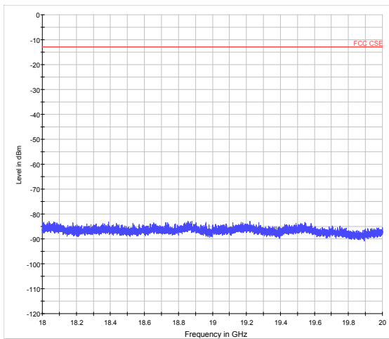
LTE Band 2 1.4MHz CH-Low 18GHz~20GHz
