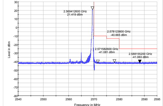
LTE Band 7 QPSK 10MHz CH-High, 1 RB
