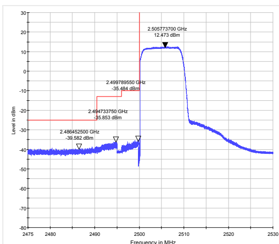
LTE Band 7 16QAM 10MHz CH-Low, 100%RB
