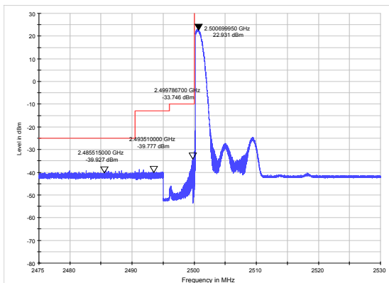
LTE Band 7 16QAM 10MHz CH-Low, 100%RB
