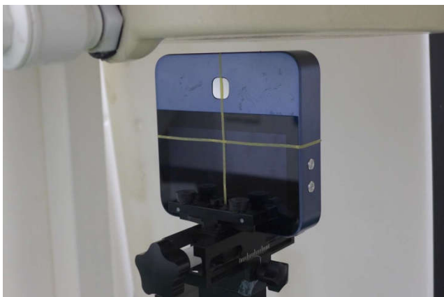
Bottom Side of the DUT with Phantom 10 mm Gap
