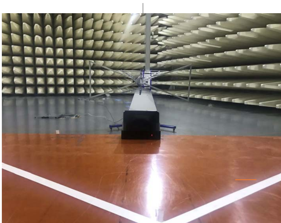
Spurious Radiated Emissions Test setup (below 1GHz)
