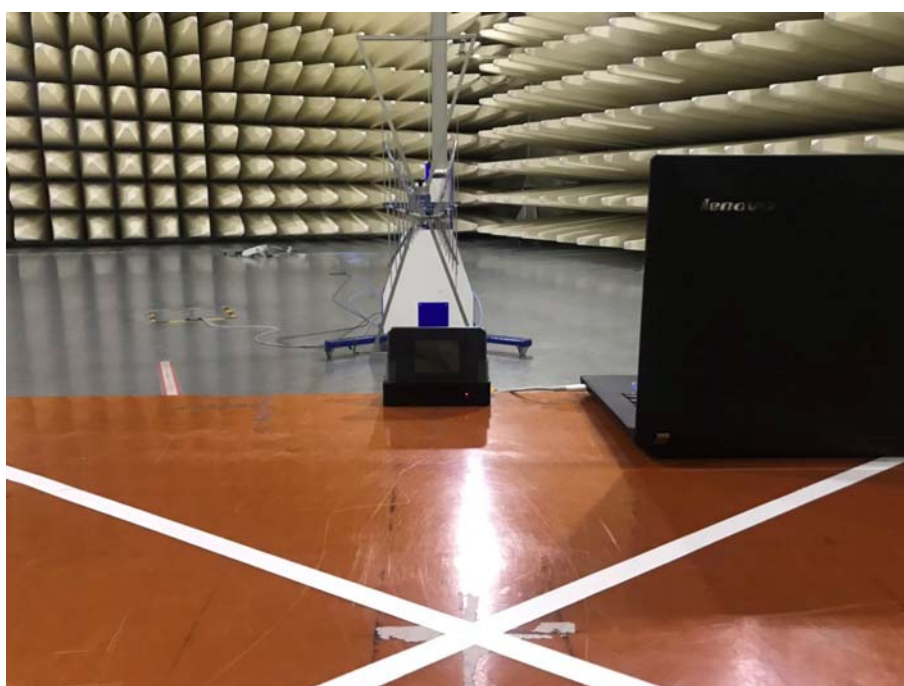
Spurious Radiated Emissions Test setup (30MHz~1GHz with laptop)
