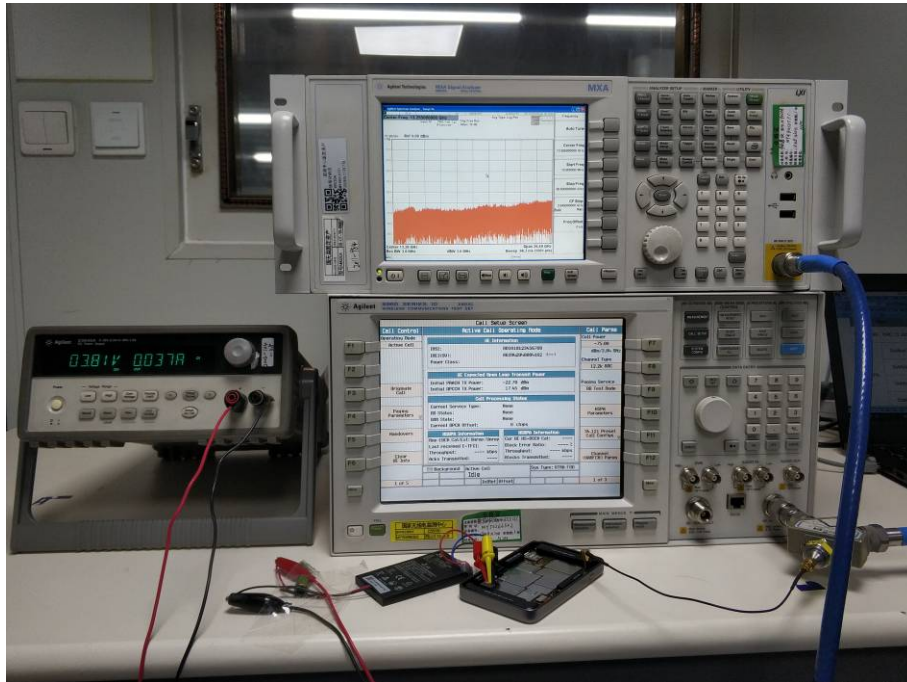
RF Conducted Test setup (WCDMA)
