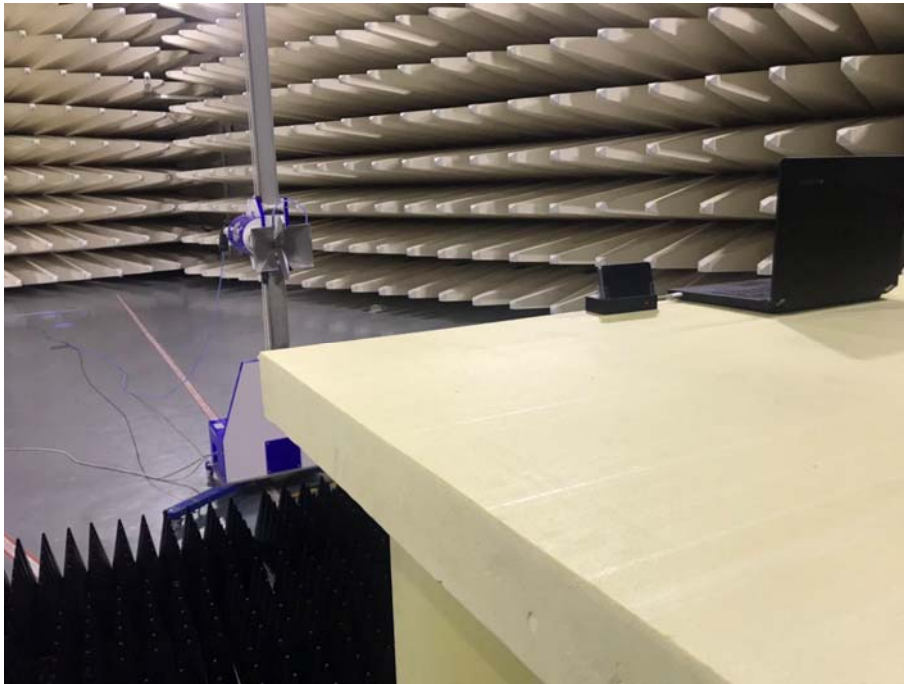
Spurious Radiated Emissions Test setup (>1GHz with laptop)
