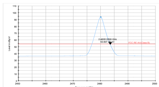
DH5-Channel 78: Average
