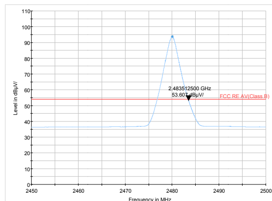
3DH5-Channel 78: Average
