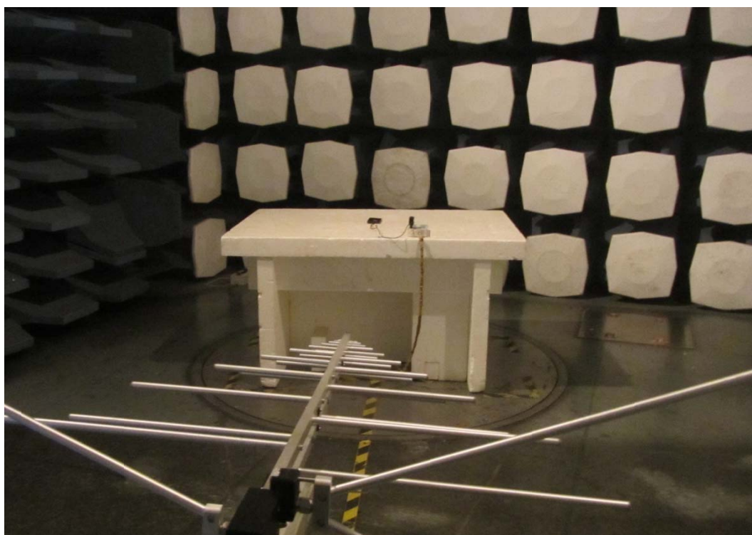
Below 1GHz
