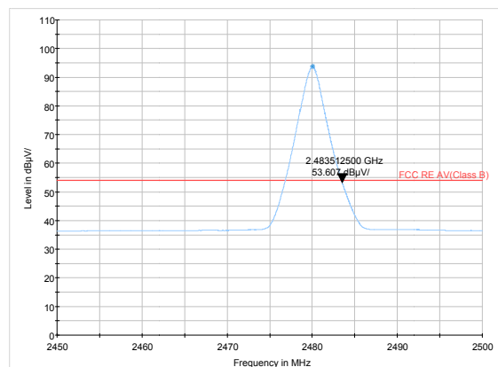
3DH5-Channel 78: Average
