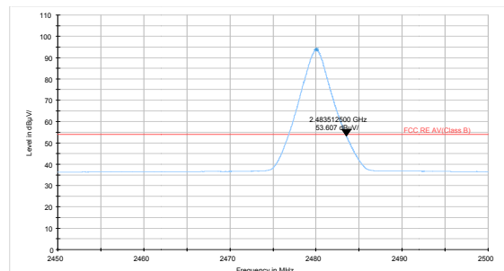
DH5-Channel 78: Average
