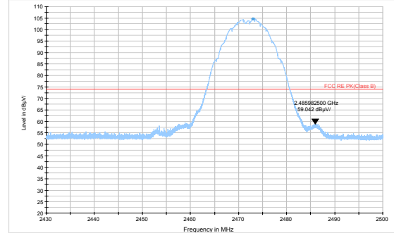
802.11b-Channel 13: Peak
