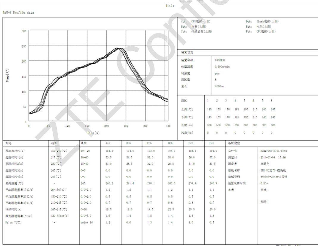
Figure 9-4 Module Furnace Temperature Curve Diagram
