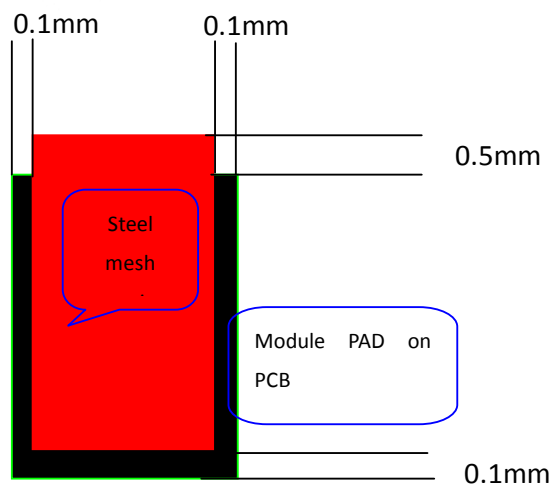
Figure 9-2 Module Board's Steel Mesh Diagram
