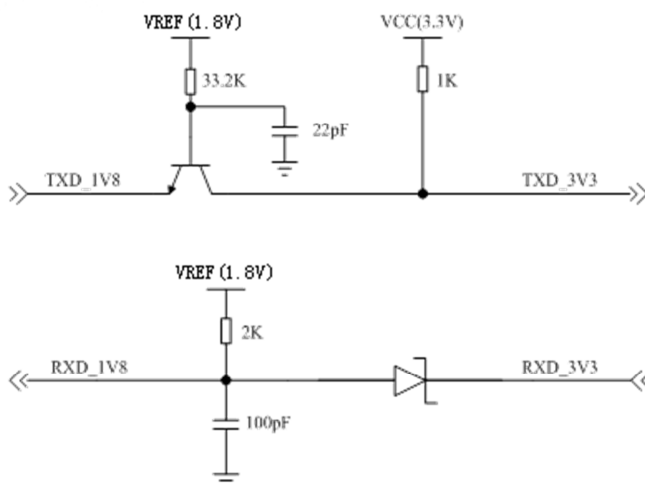
Figure 4-9 Module Serial Port &amp; AP Application Processor
