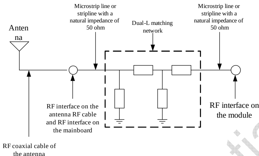
Figure 5-1 Translation Circuit Diagram
