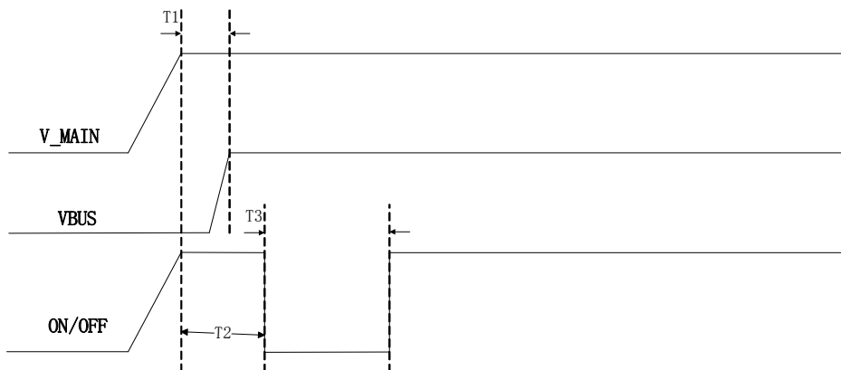
Figure 4-7 Power-off Sequence Chart of Module
