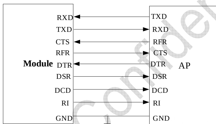
Figure 4-9 Module Serial Port &amp; AP Application Processor
