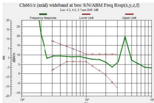
Fig 7.2 GSM1900 Ch661
