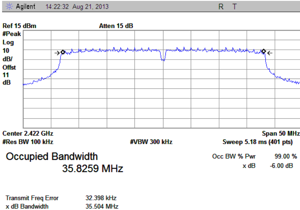
(Plot G: Channel 1: 2422MHz @ 802.11n-40)
