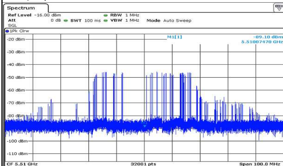
EUT (Client ) links with master on 5510MHz
