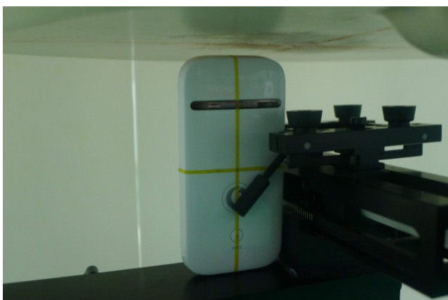
Top Side of the DUT with Phantom 0.5 cm Gap
