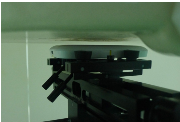
Back of the DUT with Phantom 0.5 cm Gap
