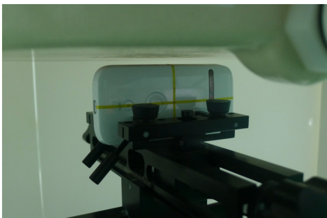
Left Side of the DUT with Phantom 0.5 cm Gap
