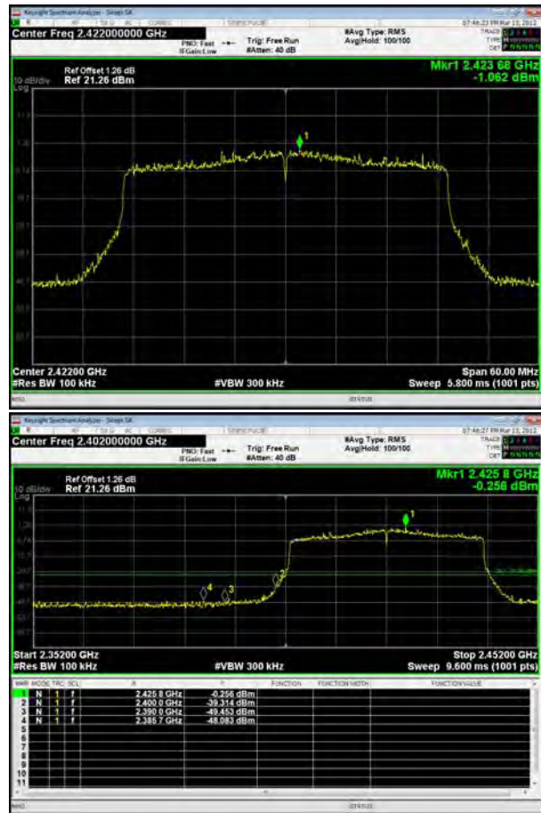
802.11ax(HE40), Channel No. 3
