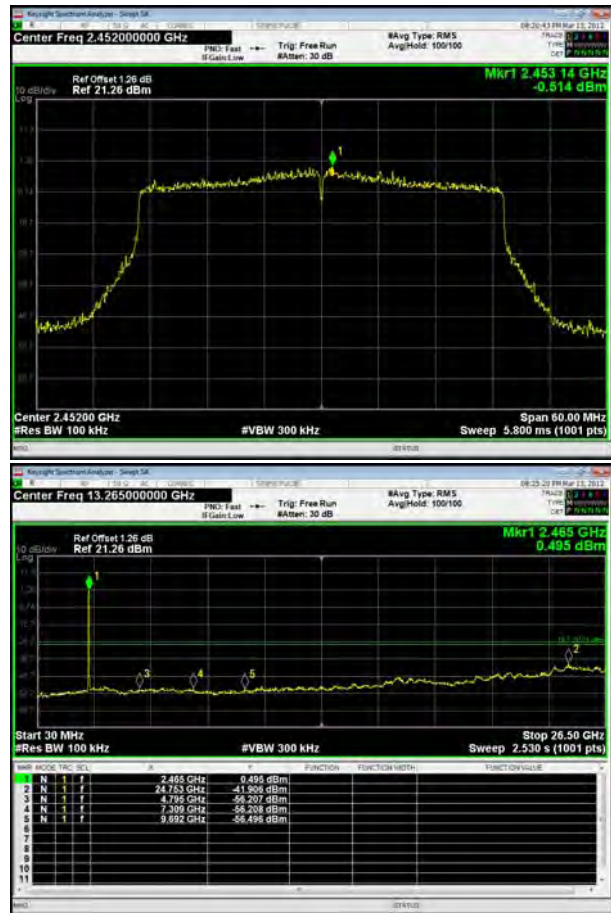
802.11ax(HE40), Channel No. 9
