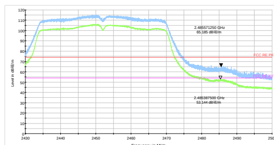
40 -Channel 9 Peak+ Average
