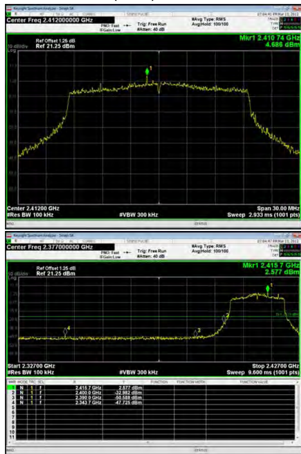
802.11ax(HE20), Channel No. 1
