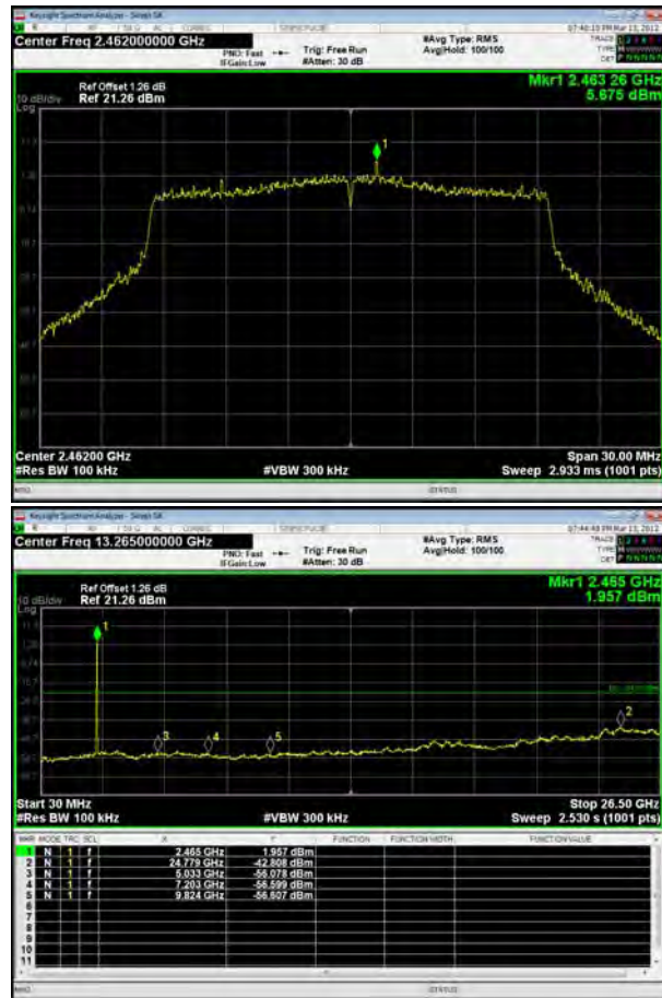
802.11ax(HE20), Channel No. 11
