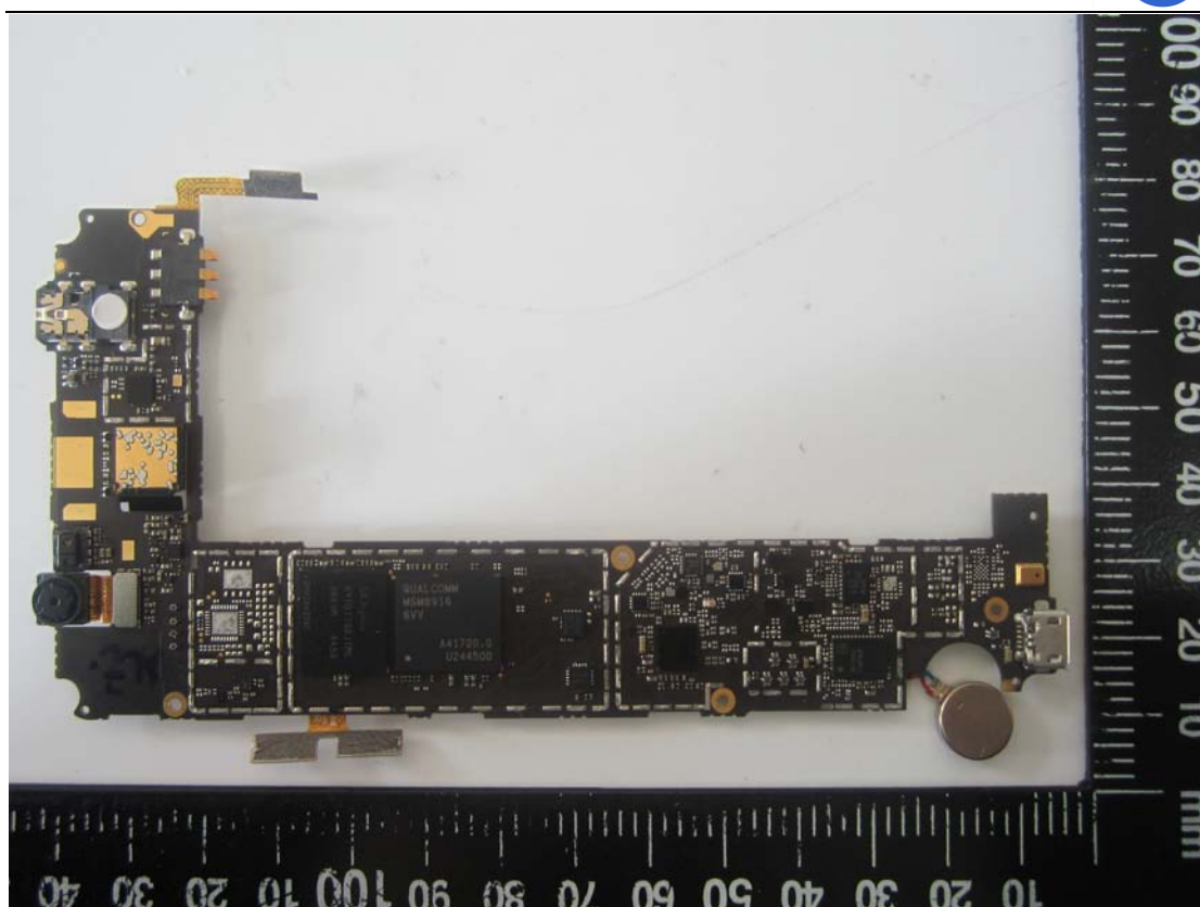
4. GSM/WCDMA/LTE chip view
