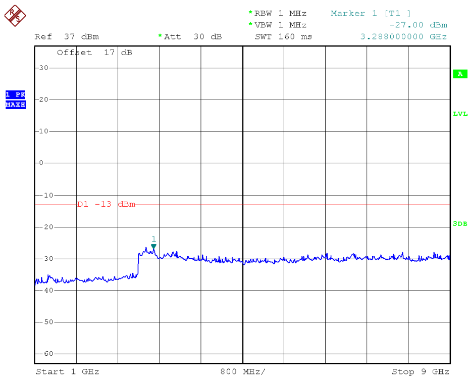
WCDMA850MHz Channel = 4233, 1GHz to 9GHz
