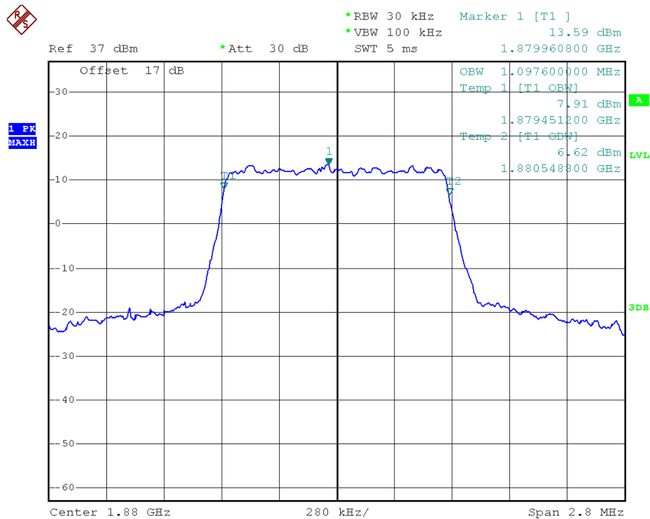
99% Occupied Bandwidth LTE Band 2 1.4MHz/QPSK
