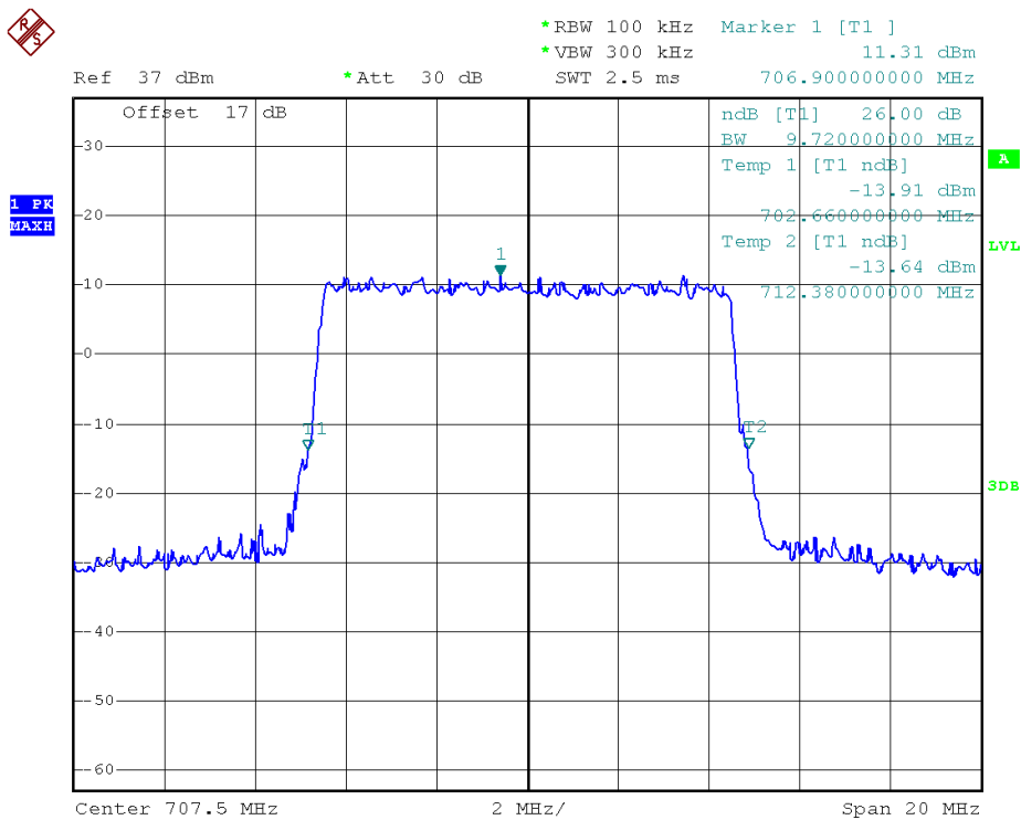
26dB Bandwidth LTE Band 12/10MHz/QPSK
