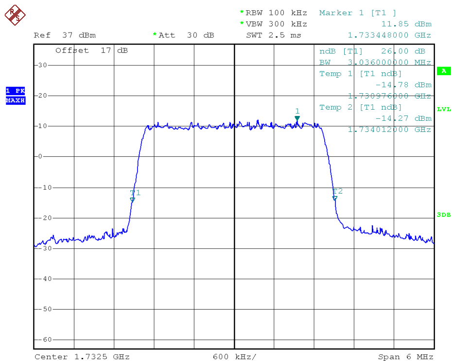
26dB Bandwidth LTE Band 4/3MHz/QPSK
