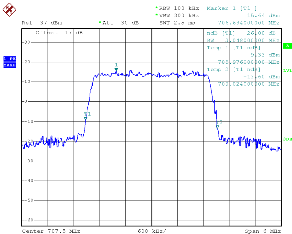
26dB Bandwidth LTE Band 12/3MHz/16QAM
