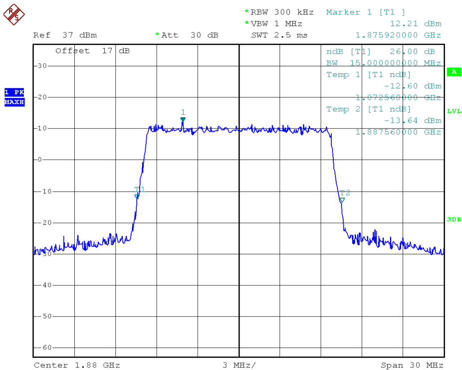
26dB Bandwidth LTE Band 2/15MHz/16QAM
