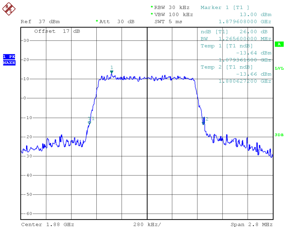
26dB Bandwidth LTE Band 2 1.4MHz/16QAM
