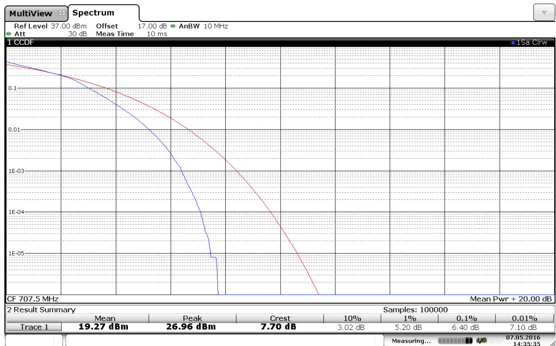
(Plot D3: Band 12/10MHz/16QAM in M Ch 1RB Size)
