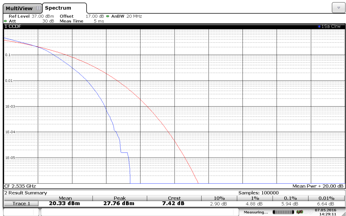
(Plot C3: Band 7/20MHz/16QAM in M Ch 1RB Size)
