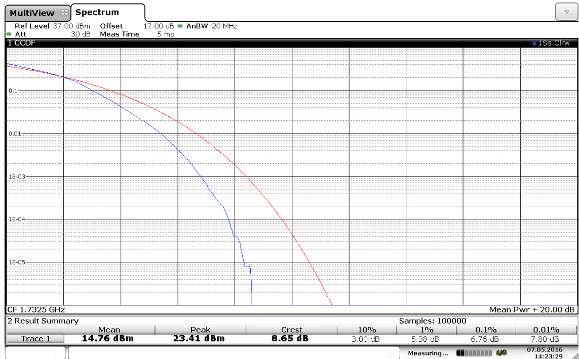
(Plot B4: Band 4/20MHz/16QAM in M Ch 100RB Size)
