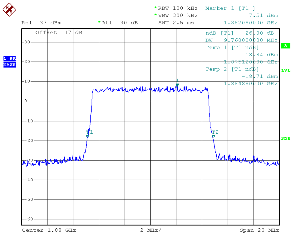
26dB Bandwidth LTE Band 2/10MHz/16QAM
