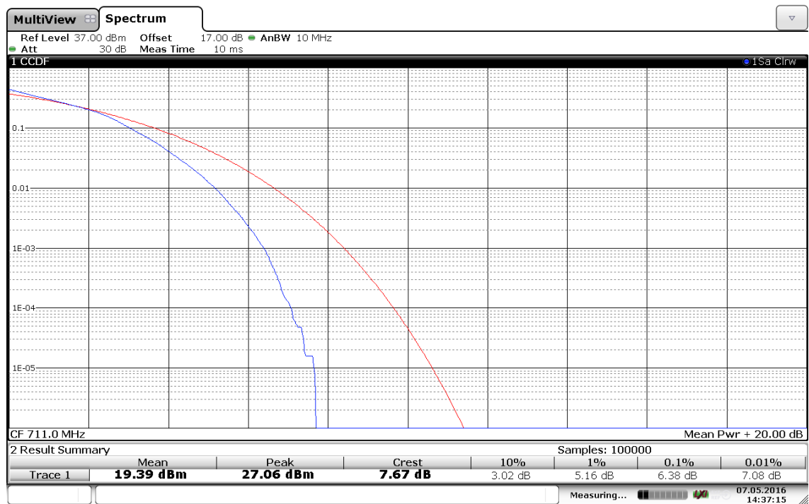
(Plot D5: Band 12/10MHz/16QAM in H Ch 1RB Size)
