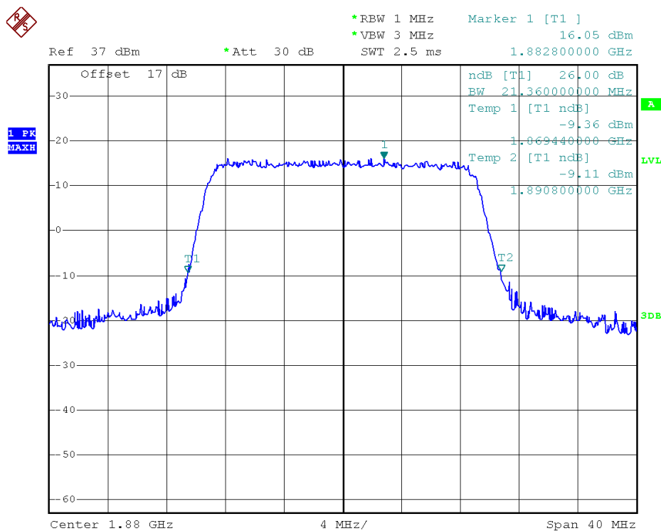
26dB Bandwidth LTE Band 2/20MHz/QPSK
