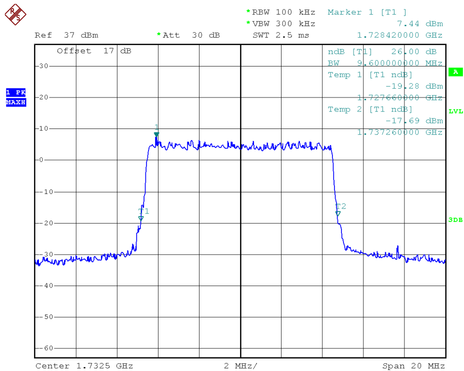
26dB Bandwidth LTE Band 4/10MHz/QPSK
