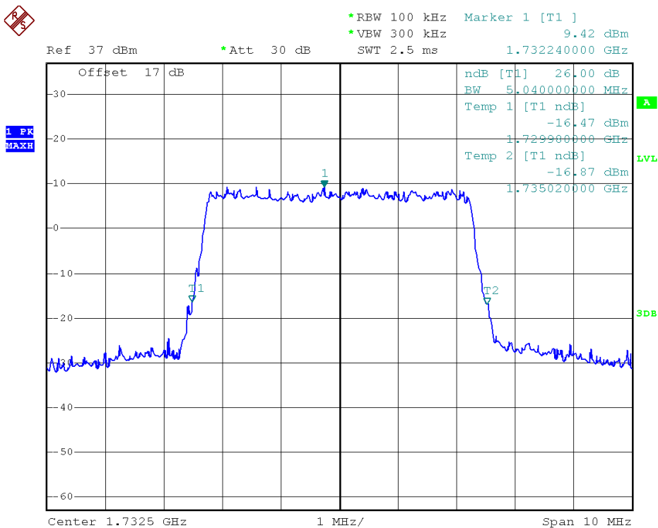
26dB Bandwidth LTE Band 4/5MHz/QPSK
