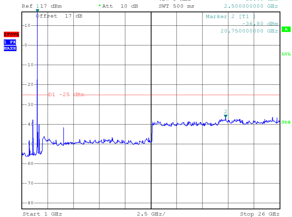
RB Size 1, RB Offset 0 1GHz to 26GHz
