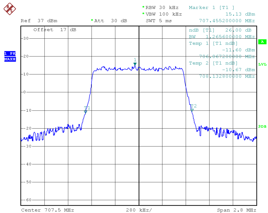
26dB Bandwidth LTE Band 12/1.4MHz/QPSK
