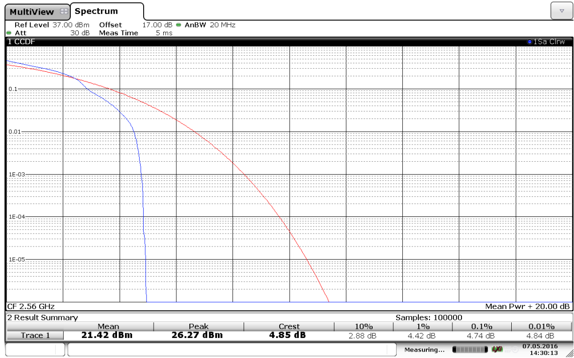
(Plot C5: Band 7/20MHz/16QAM in H Ch 1RB Size)
