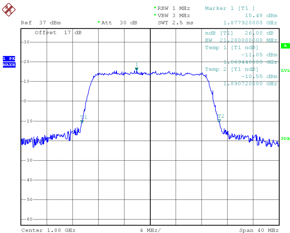
26dB Bandwidth LTE Band 2/20MHz/16QAM
