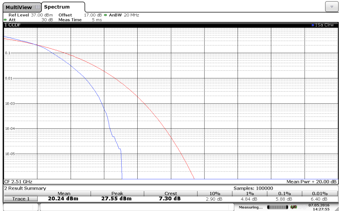
(Plot C1: Band 7/20MHz/16QAM in L Ch 1RB Size )
