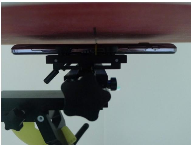
Bottom Face of Tablet with Phantom 1 cm Gap
