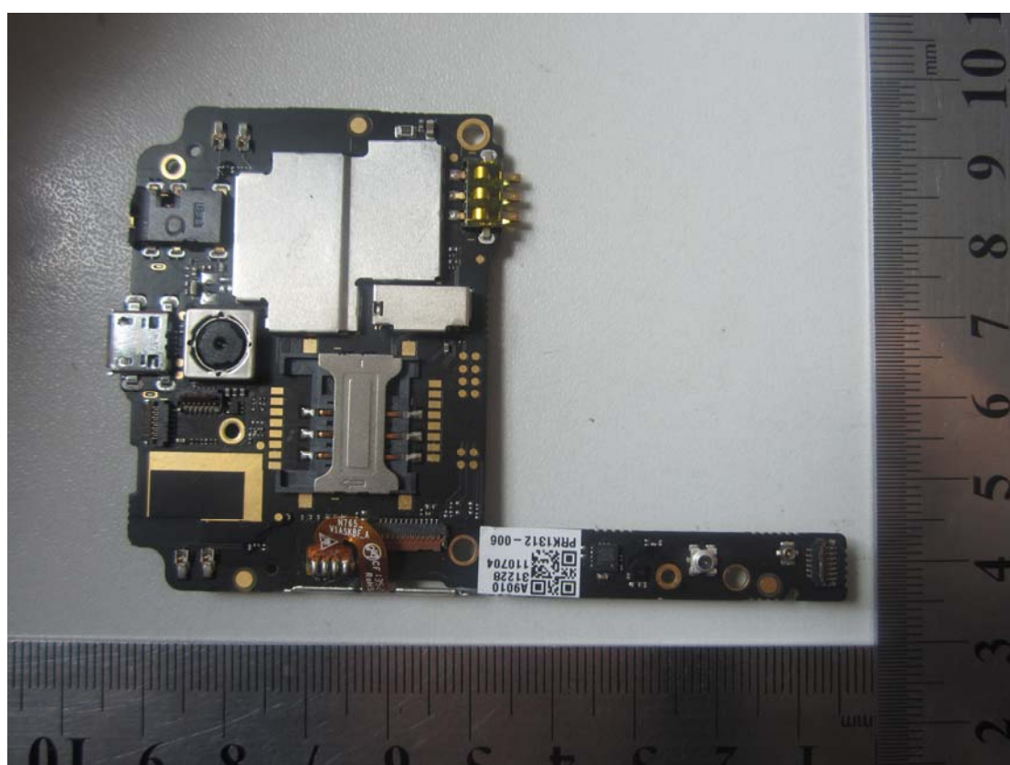
2. Mainboard front view with shielding
