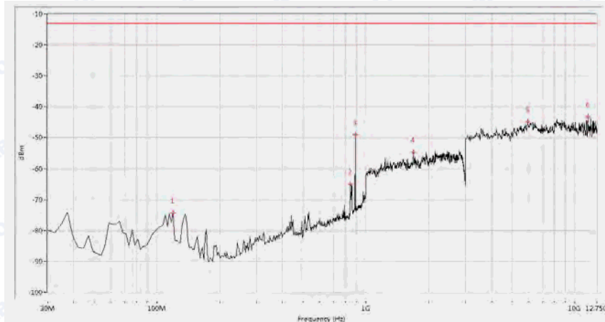
(Plot K.4: HSPA+ 850MHz Channel = 4175, Test Antenna Vertical)
