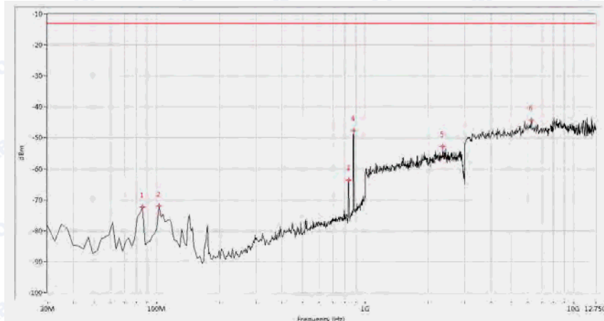
(Plot K.2: HSPA+ 850 MHz Channel = 4132, Test Antenna Vertical)
