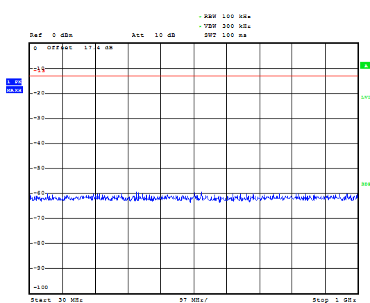
GSM 1900 CH-High 30MHz~1GHz
