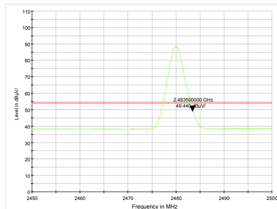
3DH5-Channel 78: Average
