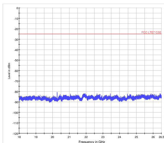
LTE Band 7 5MHz CH-Middle 18GHz~26.5GHz
