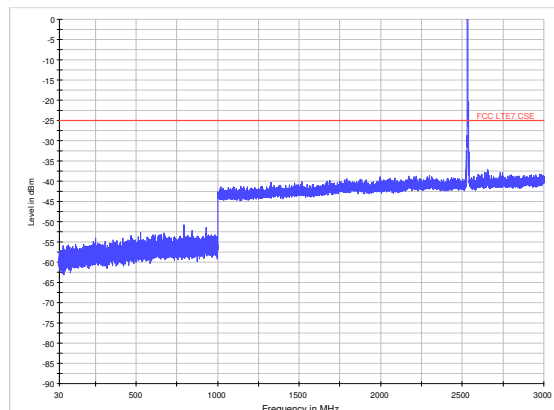
LTE Band 7 5MHz CH-Middle 30MHz~3GHz
