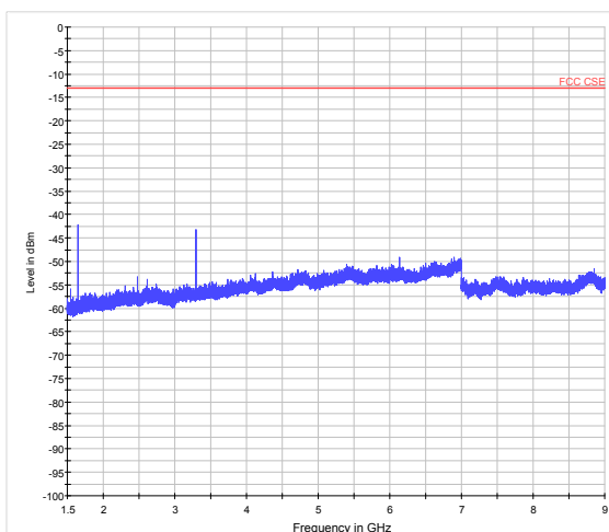
LTE Band 5 1.4MHz CH-Middle 1.5GHz~9GHz
