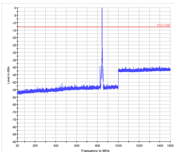
LTE Band 5 5MHz CH-High 30MHz~1.5GHz
