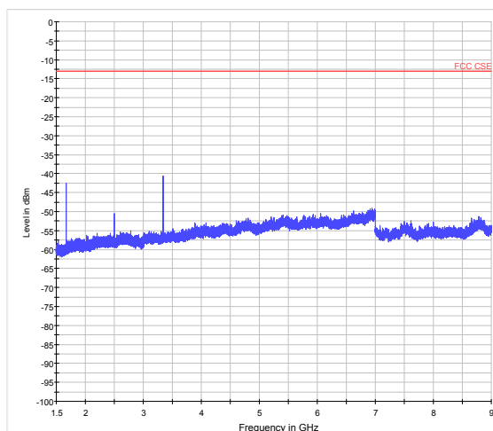
LTE Band 5 5MHz CH-High 1.5GHz~9GHz
