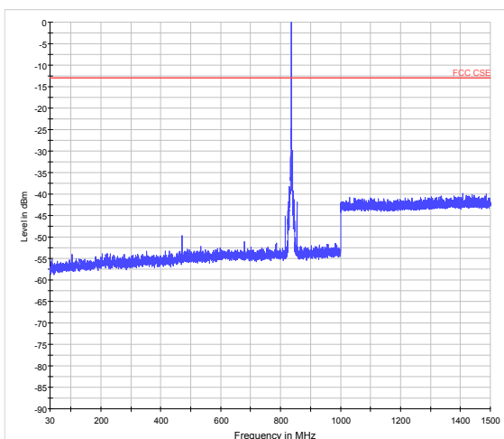
LTE Band 5 3MHz CH-High 30MHz~1.5GHz
