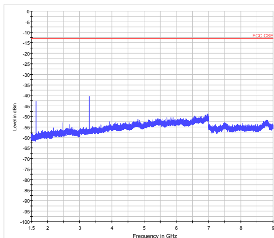
LTE Band 5 3MHz CH-Middle 1.5GHz~9GHz
