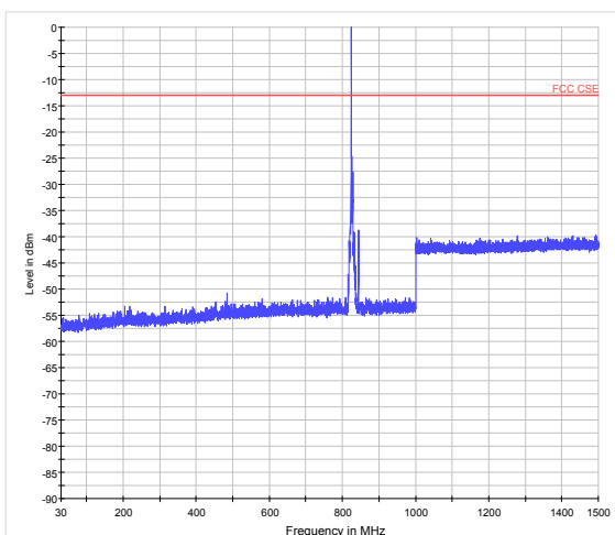
LTE Band 5 5MHz CH-Middle 30MHz~1.5GHz
