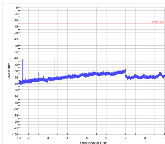
LTE Band 5 10MHz CH-High 1.5GHz~9GHz
