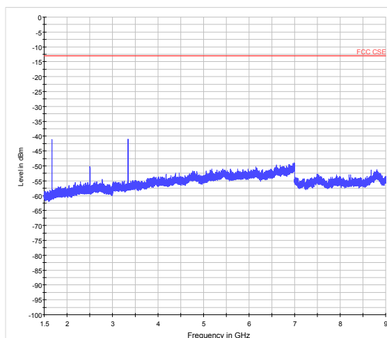
LTE Band 5 3MHz CH-High 1.5GHz~9GHz
