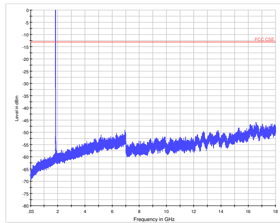
WCDMA Band II CH-Low 30MHz~18GHz
