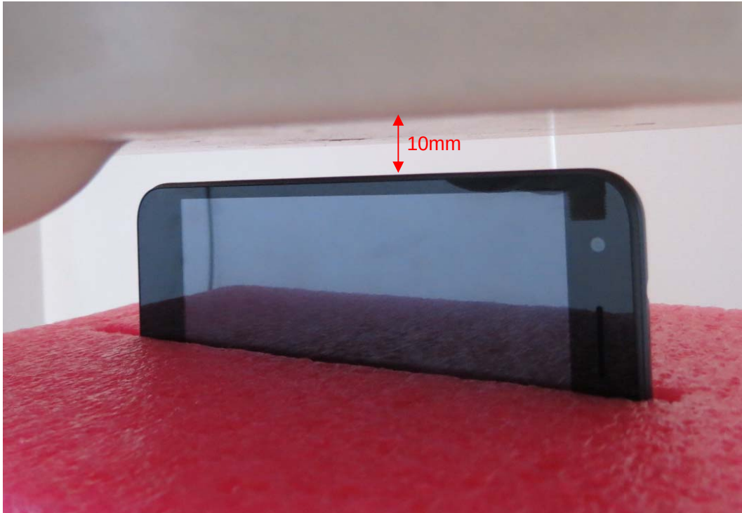
Left Side, the distance from handset to the bottom of the Phantom is 10mm
