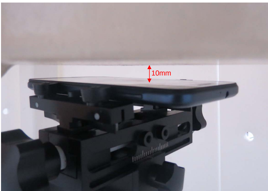
Front Side, the distance from handset to the bottom of the Phantom is 10mm
