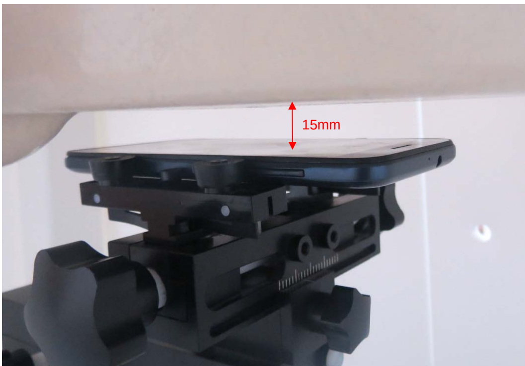
Front Side, the distance from handset to the bottom of the Phantom is 15mm
