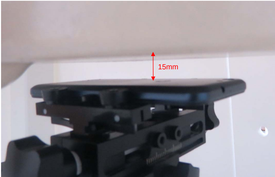
Back Side, the distance from handset to the bottom of the Phantom is 15mm
